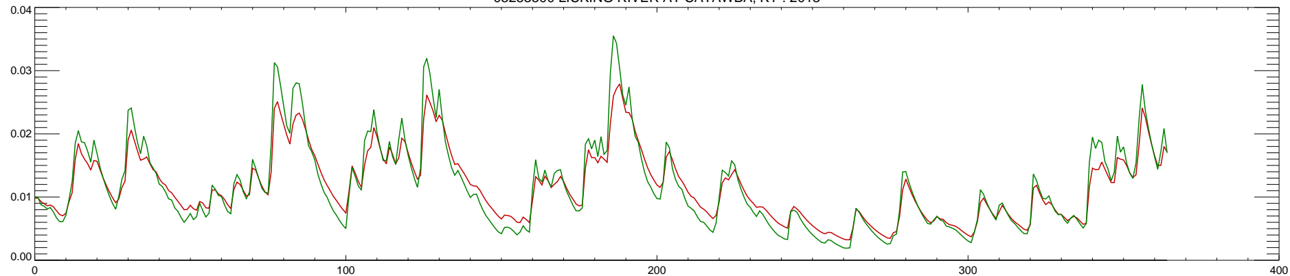
03253500 LICKING RIVER AT CATAWBA, KY : 2013
