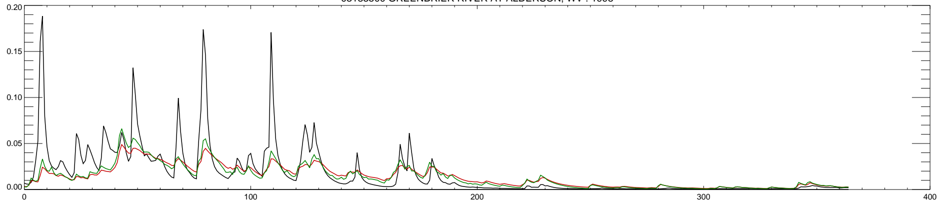
03183500 GREENBRIER RIVER AT ALDERSON, WV : 1998
