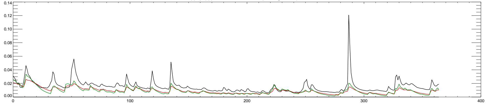
03164000 NEW RIVER NEAR GALAX, VA : 2015
