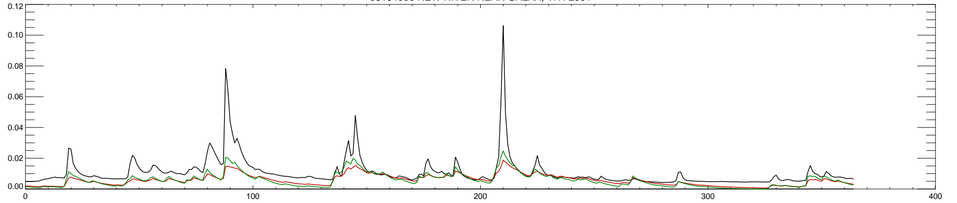
03164000 NEW RIVER NEAR GALAX, VA : 2001
