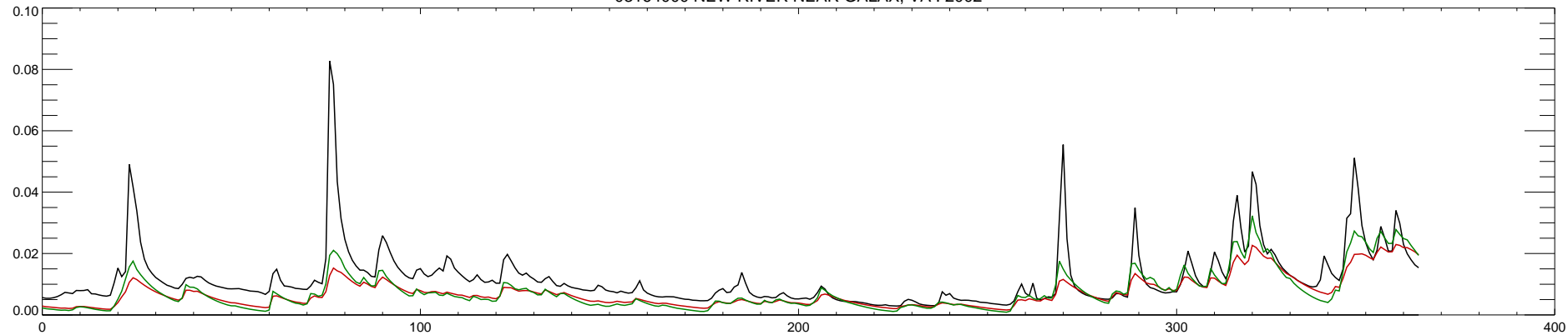
03164000 NEW RIVER NEAR GALAX, VA : 2003
