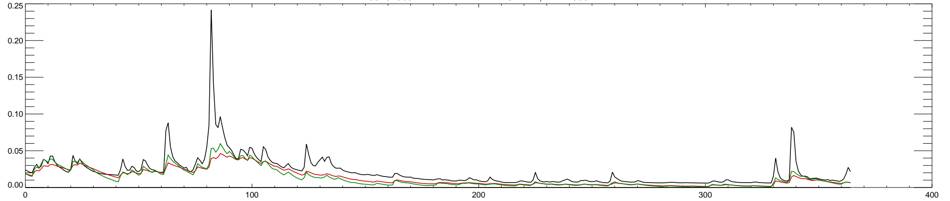
03164000 NEW RIVER NEAR GALAX, VA : 1994
