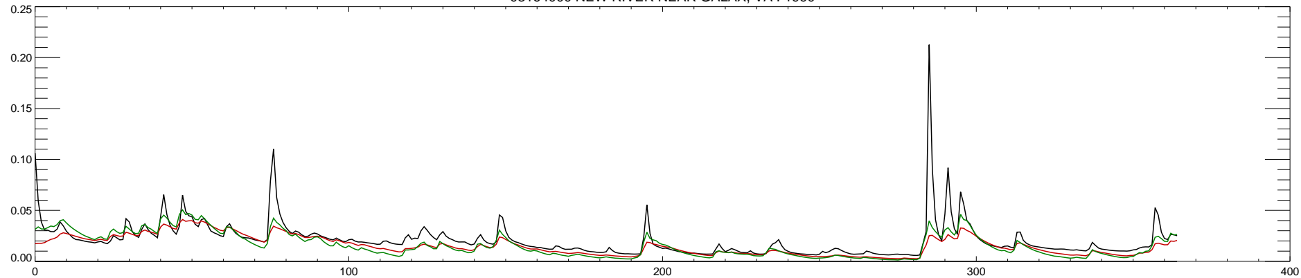
03164000 NEW RIVER NEAR GALAX, VA : 1991
