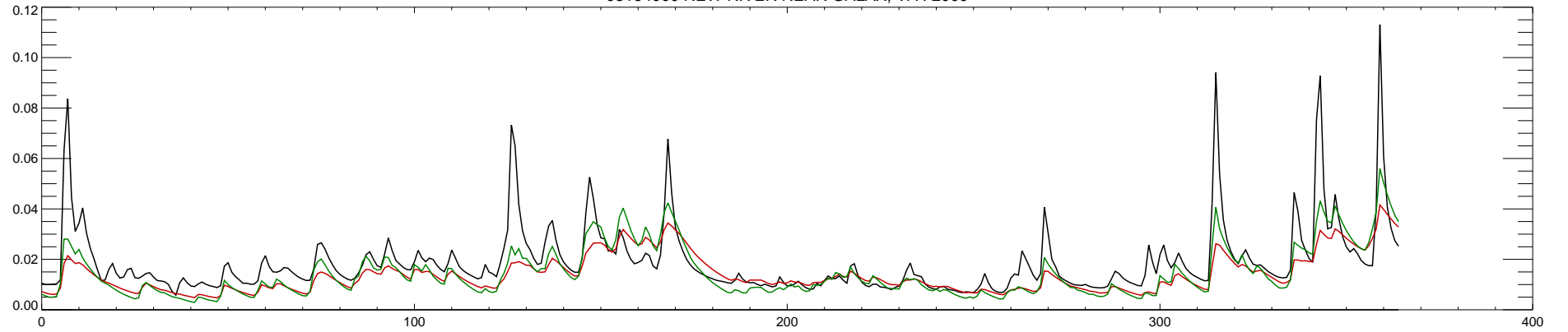
03164000 NEW RIVER NEAR GALAX, VA : 2010
