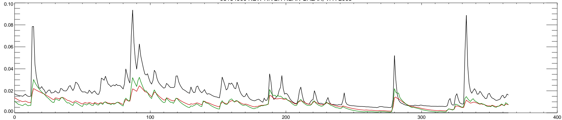
03164000 NEW RIVER NEAR GALAX, VA : 2006
