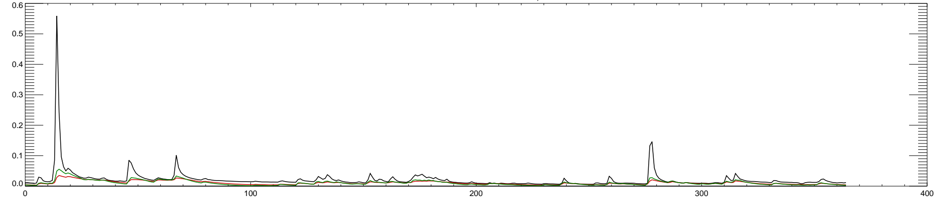
03164000 NEW RIVER NEAR GALAX, VA : 1995
