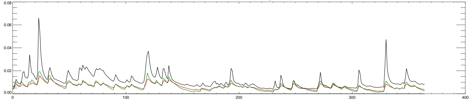
03164000 NEW RIVER NEAR GALAX, VA : 2000
