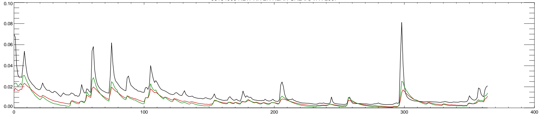
03164000 NEW RIVER NEAR GALAX, VA : 2007
