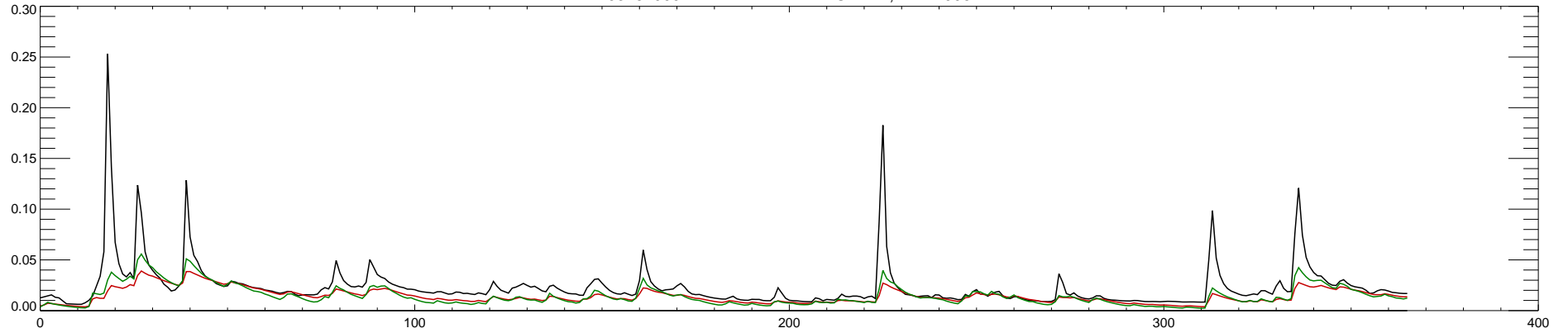
03164000 NEW RIVER NEAR GALAX, VA : 1997
