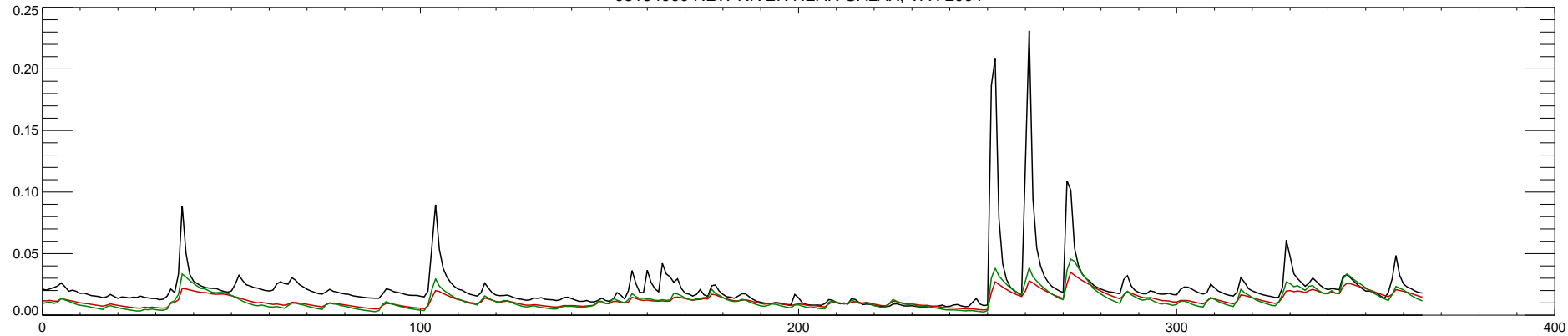
03164000 NEW RIVER NEAR GALAX, VA : 2004
