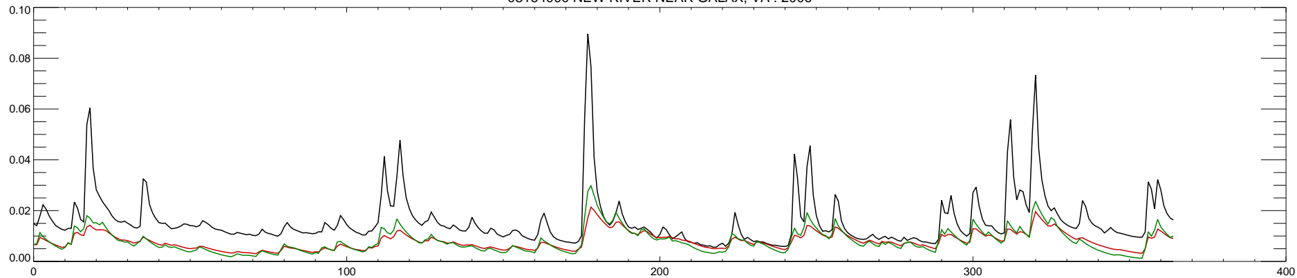
03164000 NEW RIVER NEAR GALAX, VA : 2007
