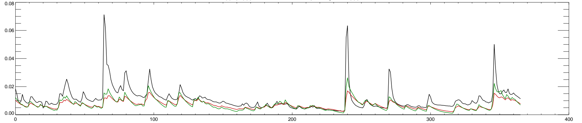
03164000 NEW RIVER NEAR GALAX, VA : 2009
