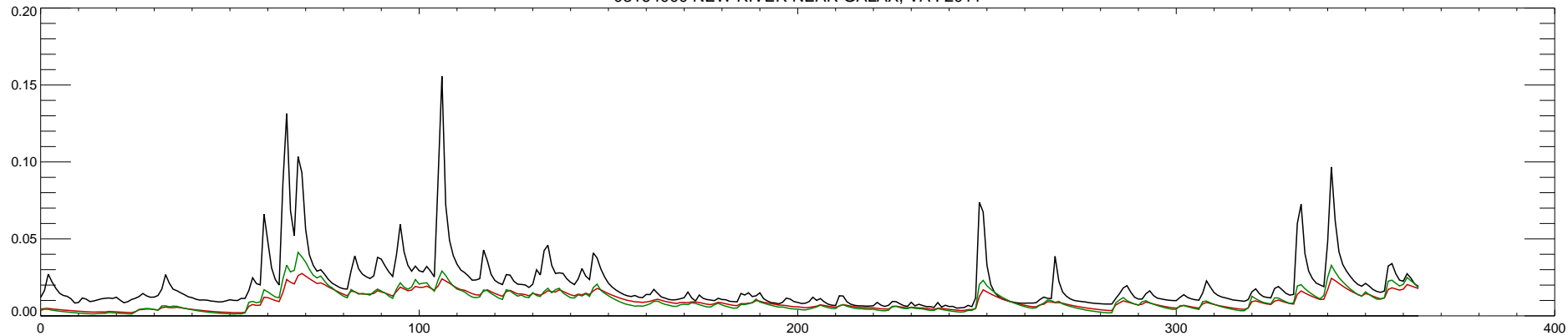
03164000 NEW RIVER NEAR GALAX, VA : 2012
