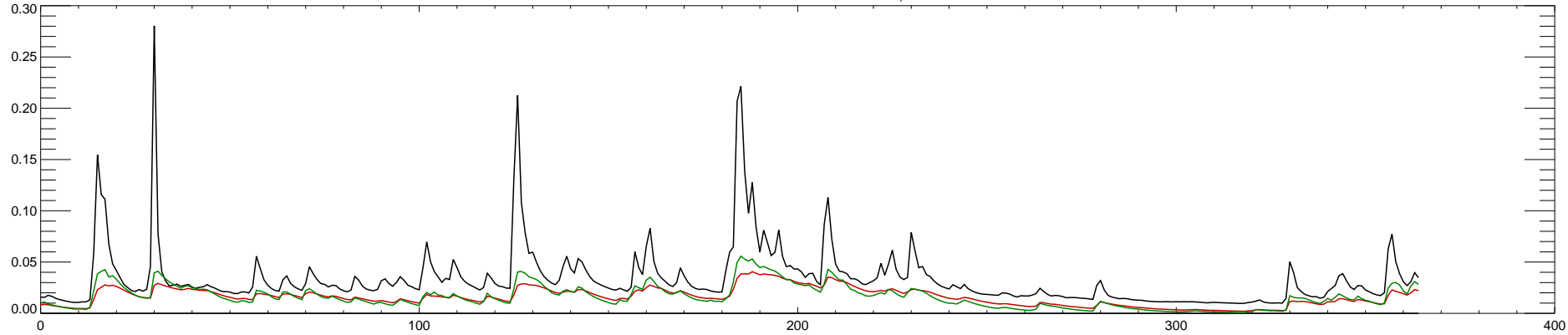
03164000 NEW RIVER NEAR GALAX, VA : 2013
