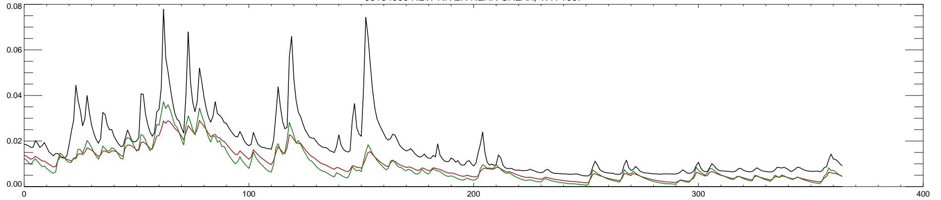
03164000 NEW RIVER NEAR GALAX, VA : 1998
