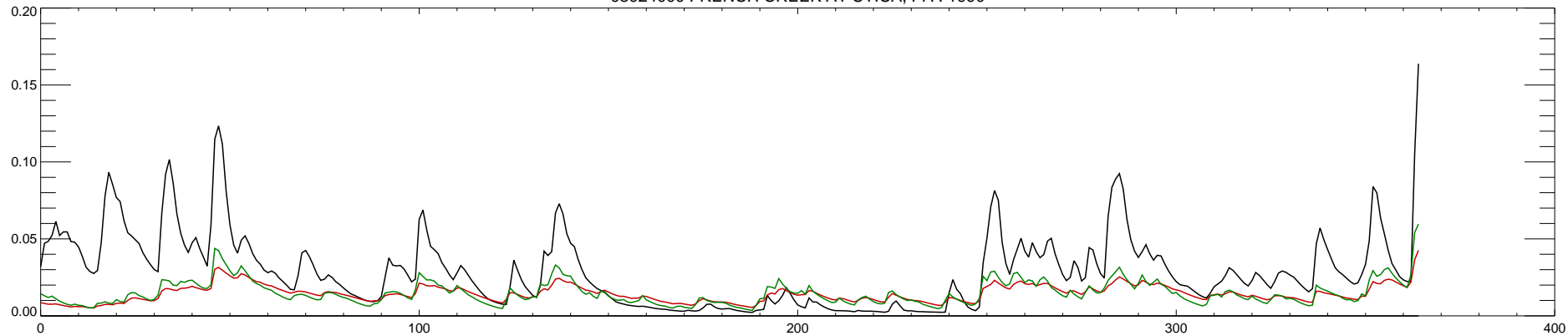
03024000 FRENCH CREEK AT UTICA, PA : 1991
