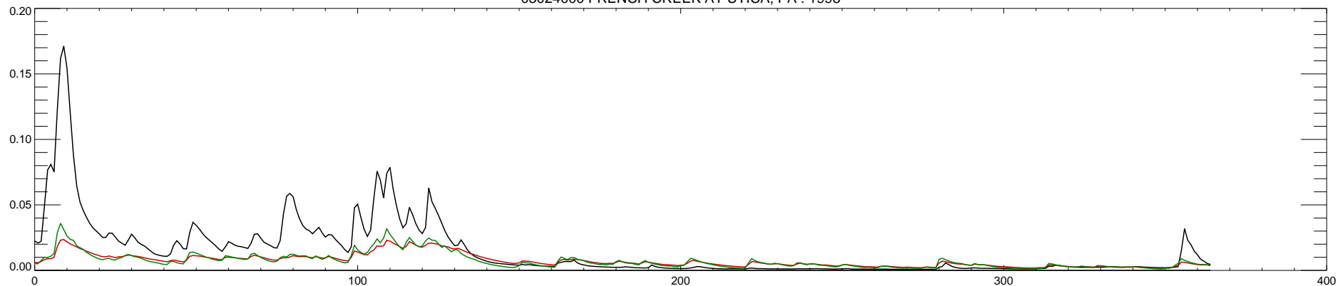
03024000 FRENCH CREEK AT UTICA, PA : 1998
