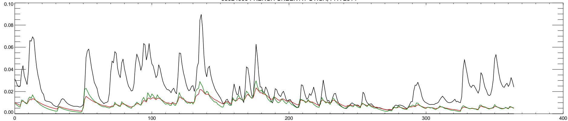
03024000 FRENCH CREEK AT UTICA, PA : 2015
