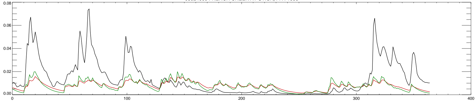
03024000 FRENCH CREEK AT UTICA, PA : 1995
