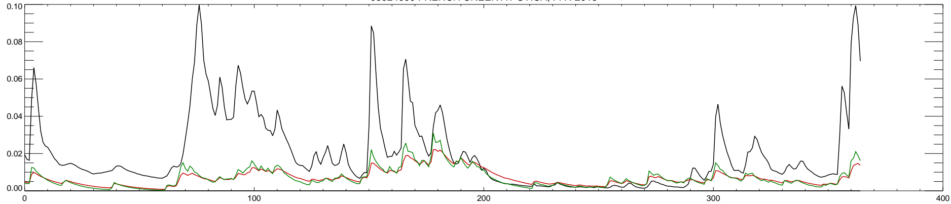
03024000 FRENCH CREEK AT UTICA, PA : 2016
