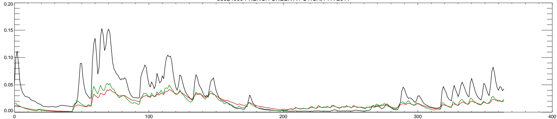
03024000 FRENCH CREEK AT UTICA, PA : 2012
