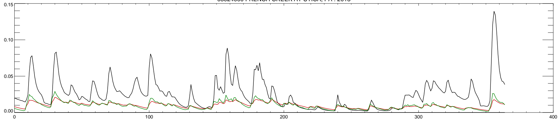
03024000 FRENCH CREEK AT UTICA, PA : 2013
