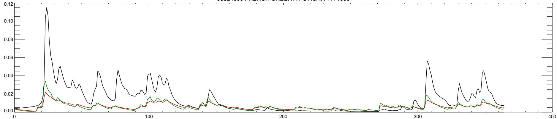
03024000 FRENCH CREEK AT UTICA, PA : 2000
