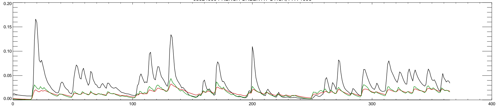
03024000 FRENCH CREEK AT UTICA, PA : 1997
