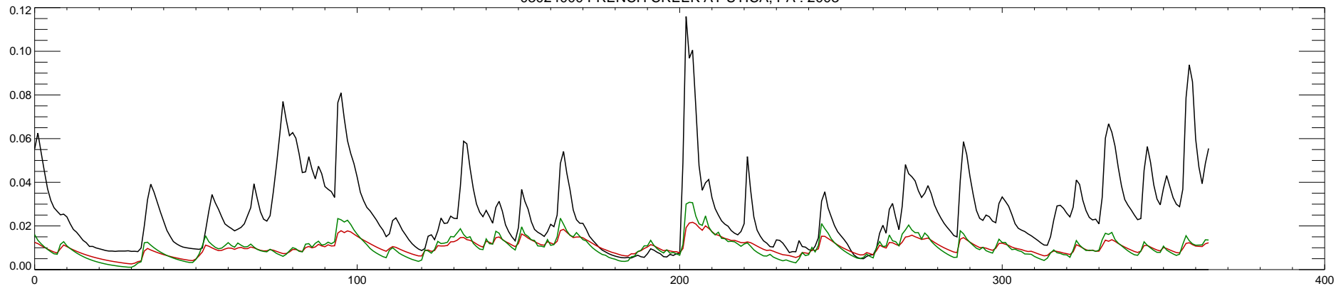
03024000 FRENCH CREEK AT UTICA, PA : 2004
