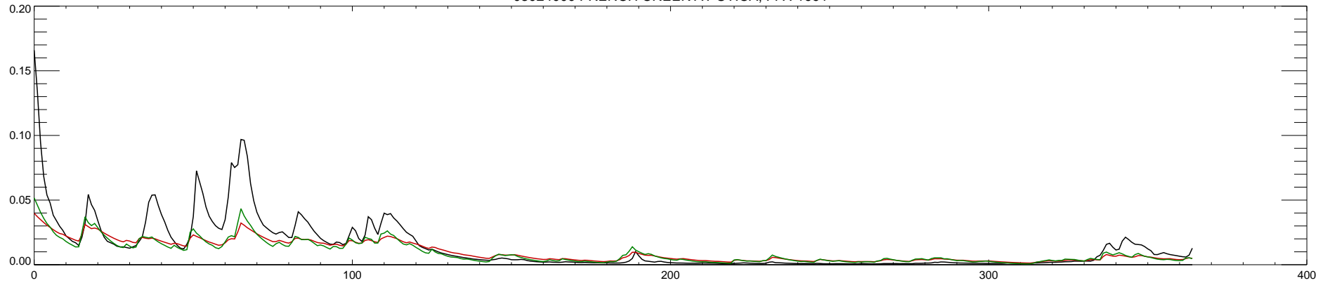
03024000 FRENCH CREEK AT UTICA, PA : 1992
