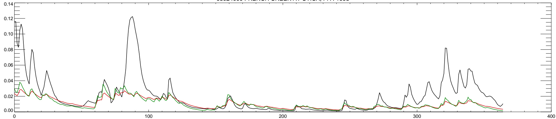
03024000 FRENCH CREEK AT UTICA, PA : 1994
