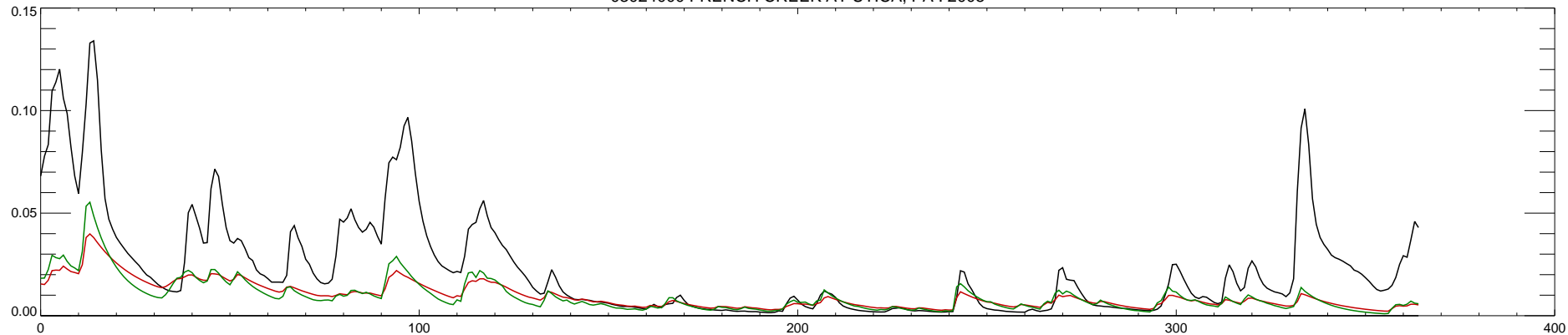
03024000 FRENCH CREEK AT UTICA, PA : 2006
