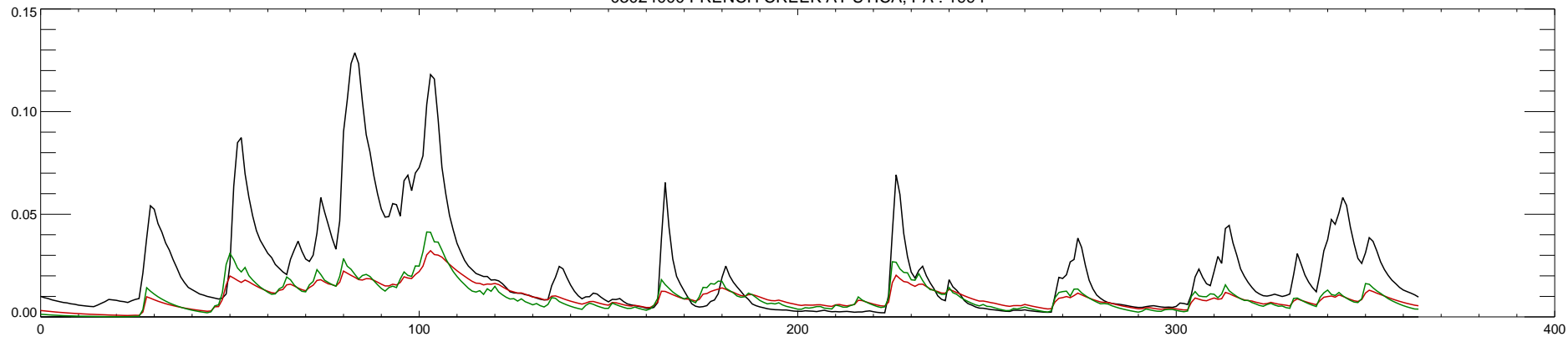
03024000 FRENCH CREEK AT UTICA, PA : 1995
