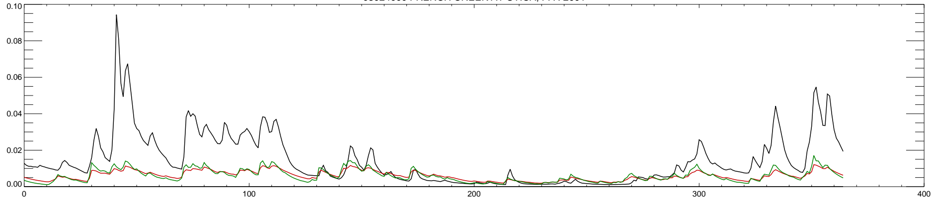
03024000 FRENCH CREEK AT UTICA, PA : 2001
