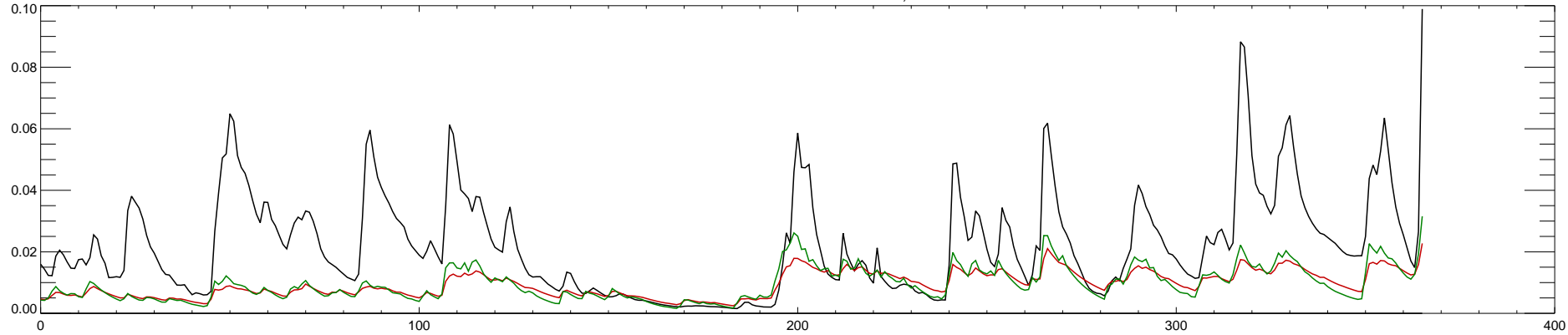
03024000 FRENCH CREEK AT UTICA, PA : 1992
