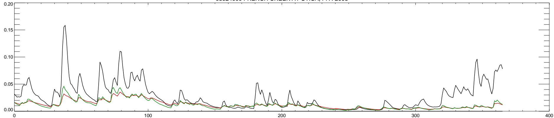
03024000 FRENCH CREEK AT UTICA, PA : 2009
