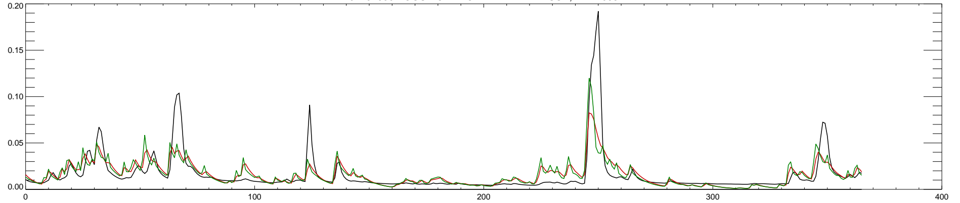
02492000 BOGUE CHITTO RIVER NEAR BUSH, LA : 2009
