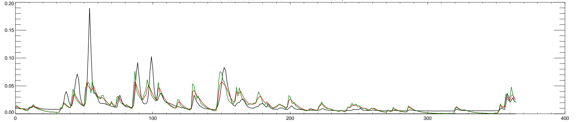
02492000 BOGUE CHITTO RIVER NEAR BUSH, LA : 2015
