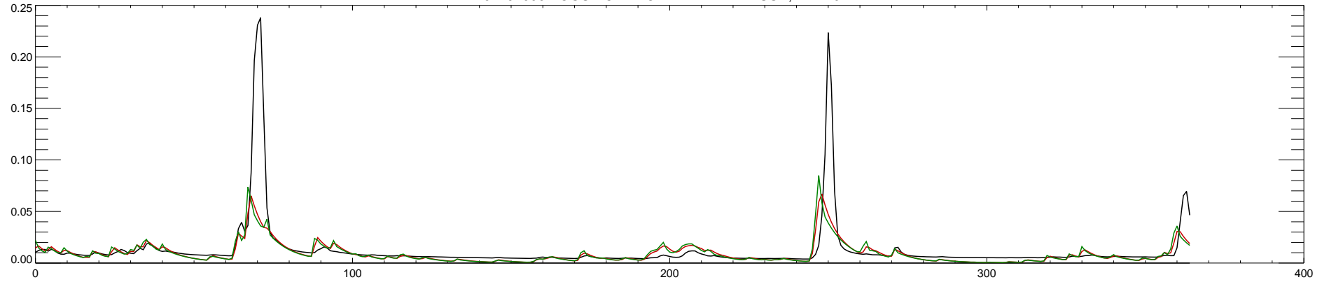
02492000 BOGUE CHITTO RIVER NEAR BUSH, LA : 2012
