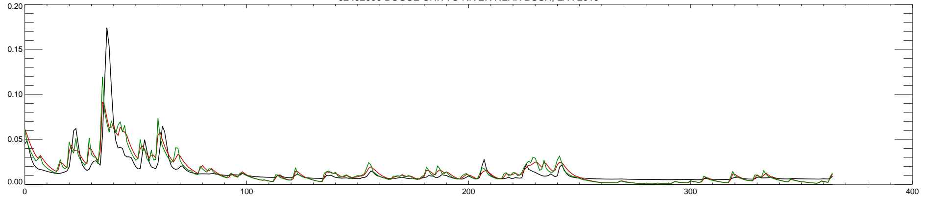
02492000 BOGUE CHITTO RIVER NEAR BUSH, LA : 2010
