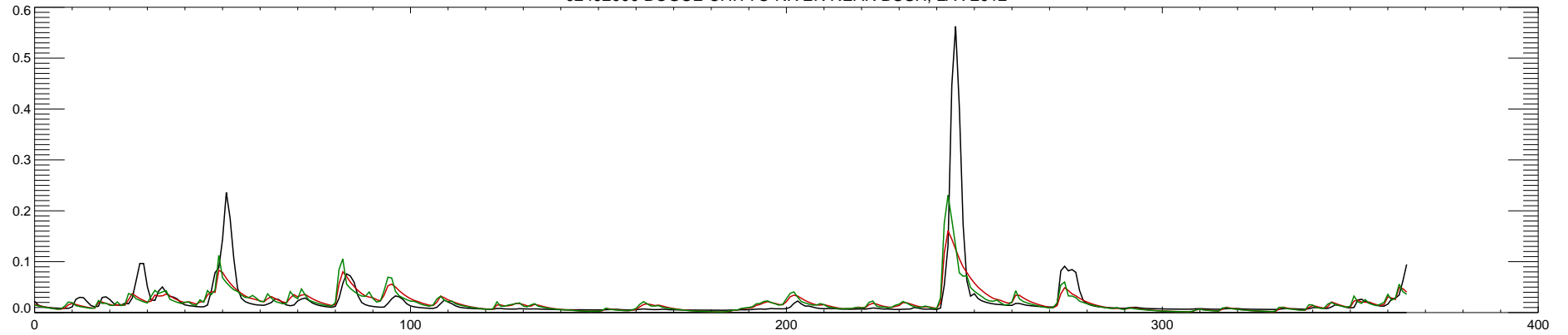
02492000 BOGUE CHITTO RIVER NEAR BUSH, LA : 2013
