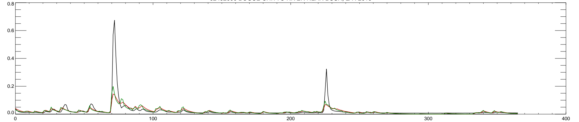
02492000 BOGUE CHITTO RIVER NEAR BUSH, LA : 2016
