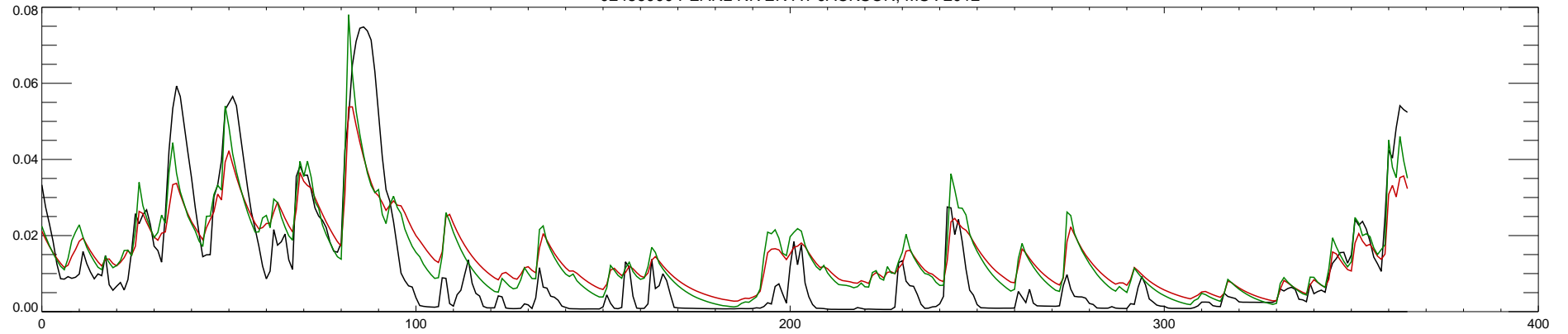
02486000 PEARL RIVER AT JACKSON, MS : 2013
