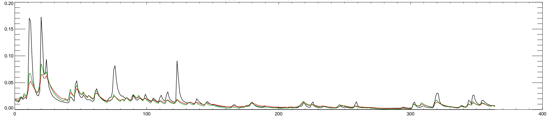
02424000 CAHABA RIVER AT CENTREVILLE AL : 1994
