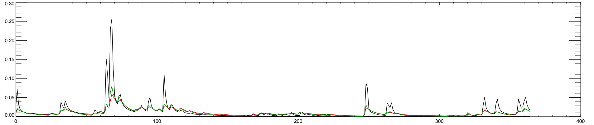
02424000 CAHABA RIVER AT CENTREVILLE AL : 2012
