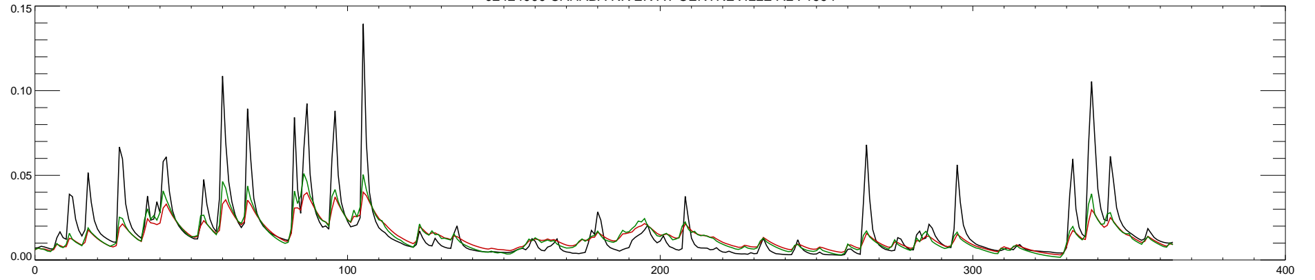
02424000 CAHABA RIVER AT CENTREVILLE AL : 1995
