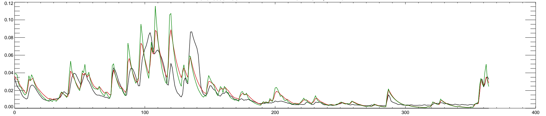
02375500 ESCAMBIA RIVER NEAR CENTURY, FL : 2015
