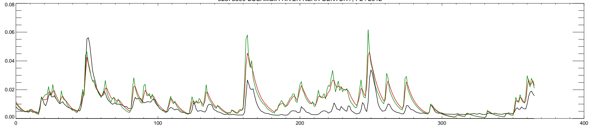
02375500 ESCAMBIA RIVER NEAR CENTURY, FL : 2013
