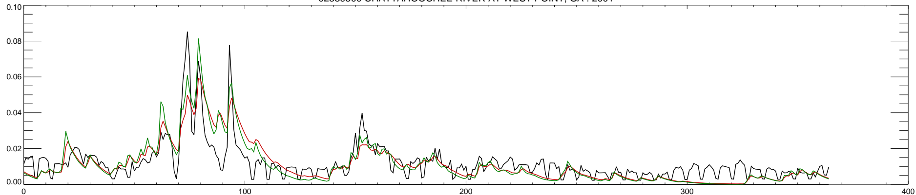
02339500 CHATTAHOOCHEE RIVER AT WEST POINT, GA : 2001
