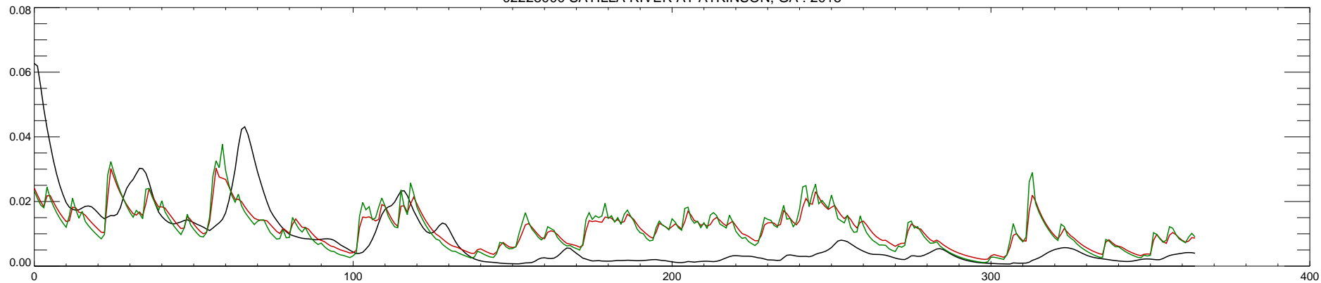
02228000 SATILLA RIVER AT ATKINSON, GA : 2016
