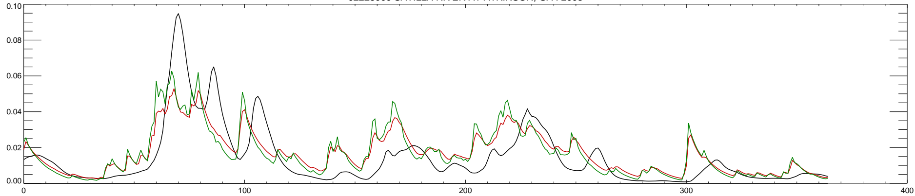
02228000 SATILLA RIVER AT ATKINSON, GA : 2004
