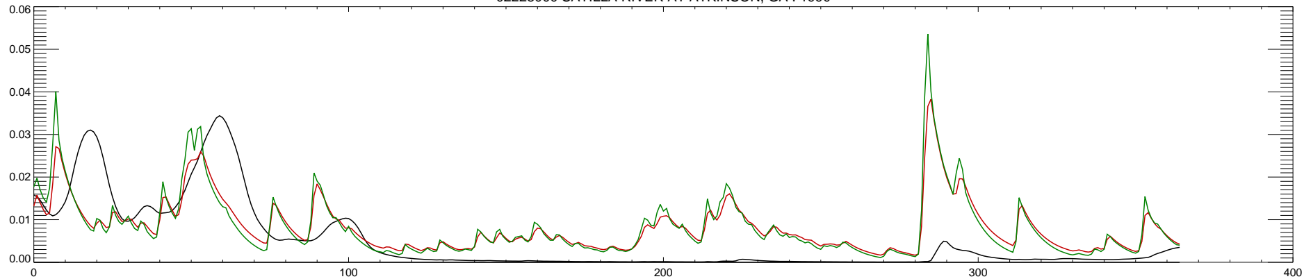
02228000 SATILLA RIVER AT ATKINSON, GA : 1991
