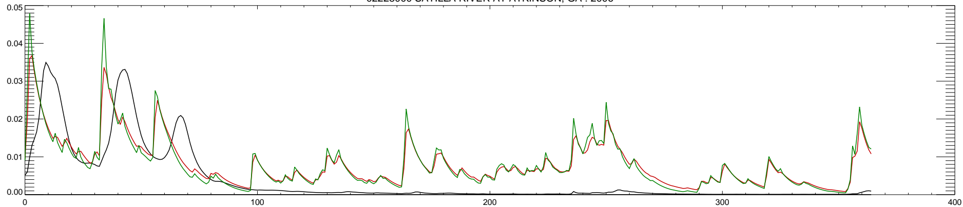
02228000 SATILLA RIVER AT ATKINSON, GA : 2007
