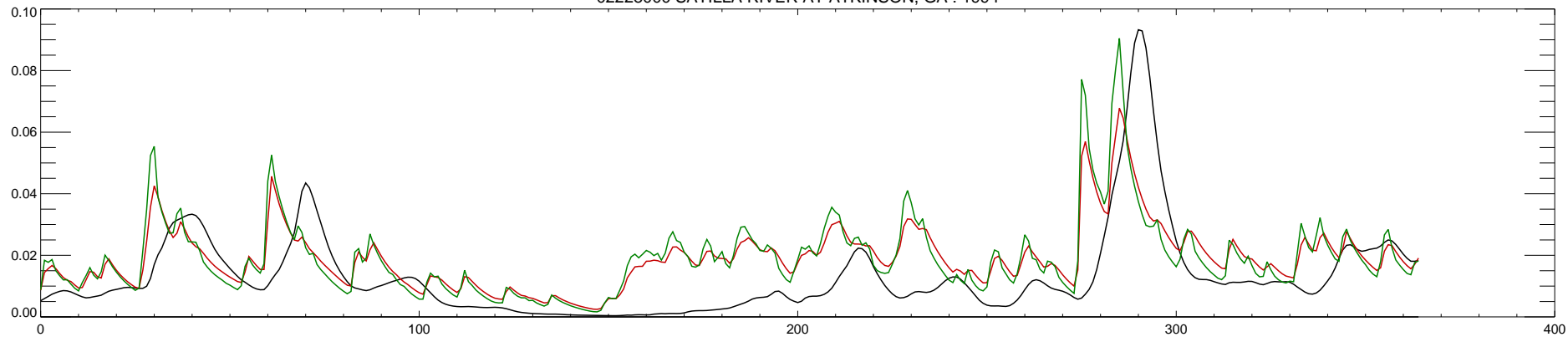
02228000 SATILLA RIVER AT ATKINSON, GA : 1995
