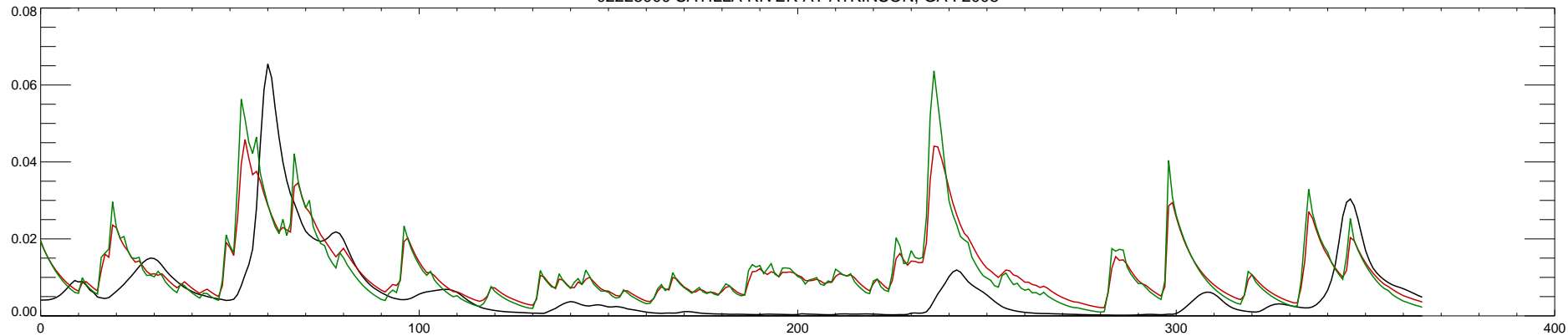
02228000 SATILLA RIVER AT ATKINSON, GA : 2009
