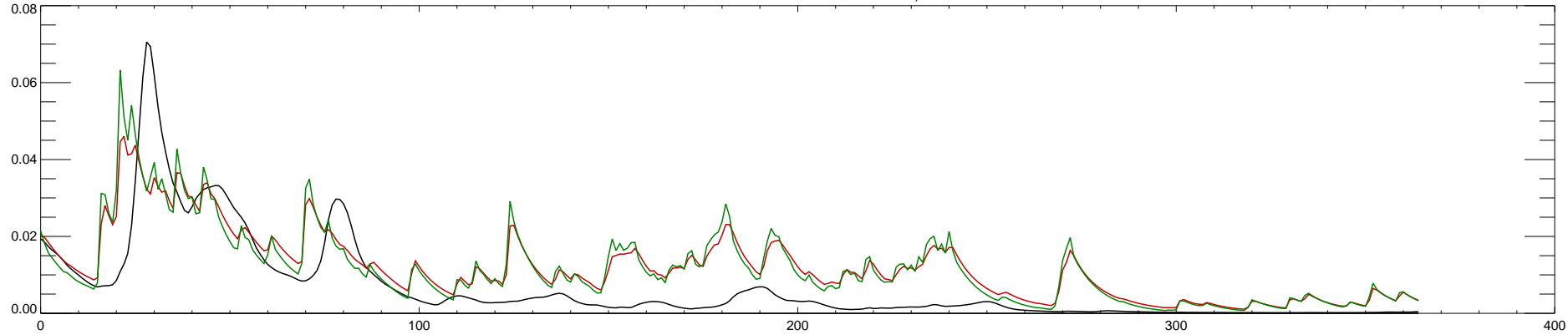
02228000 SATILLA RIVER AT ATKINSON, GA : 2010
