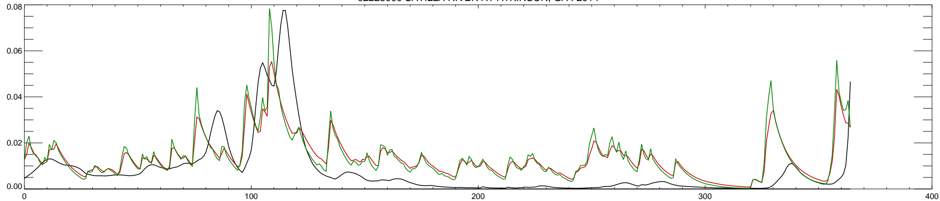
02228000 SATILLA RIVER AT ATKINSON, GA : 2015
