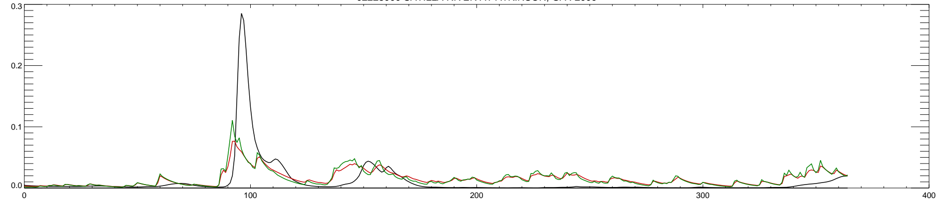
02228000 SATILLA RIVER AT ATKINSON, GA : 2010
