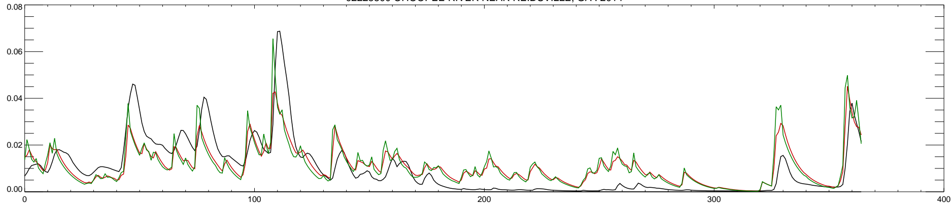
02225500 OHOOPEE RIVER NEAR REIDSVILLE, GA : 2015
