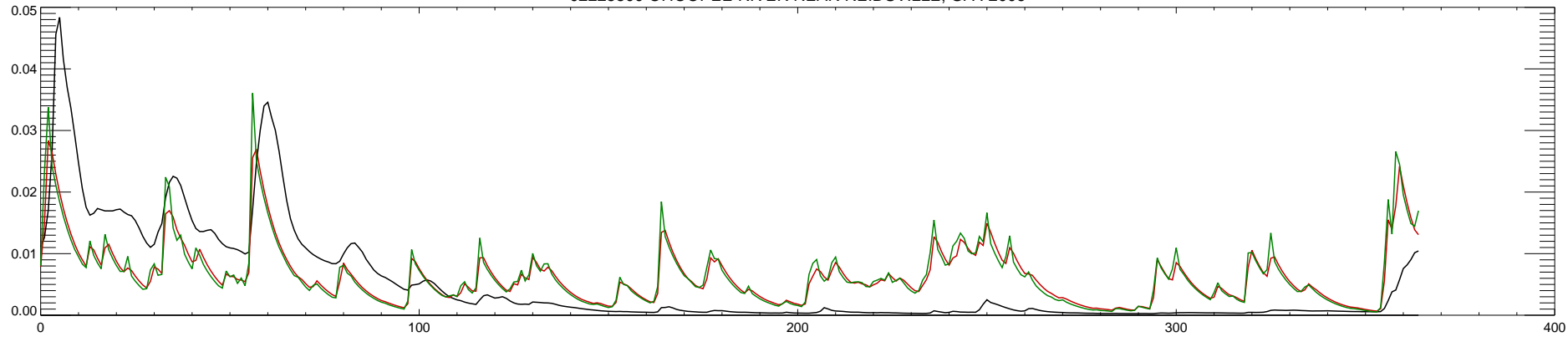
02225500 OHOOPEE RIVER NEAR REIDSVILLE, GA : 2007
