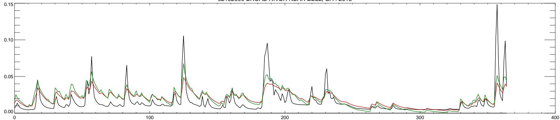
02192000 BROAD RIVER NEAR BELL, GA : 2013
