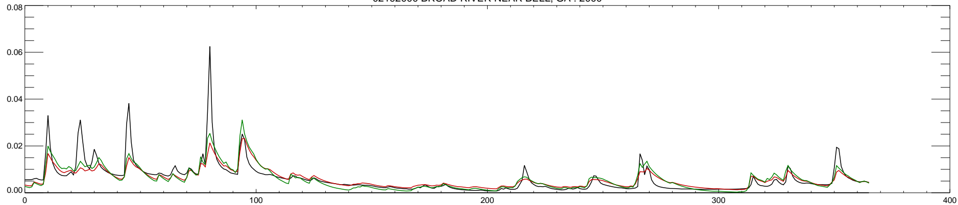
02192000 BROAD RIVER NEAR BELL, GA : 2001
