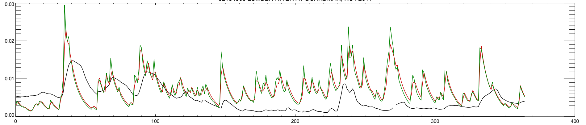
02134500 LUMBER RIVER AT BOARDMAN, NC : 2012
