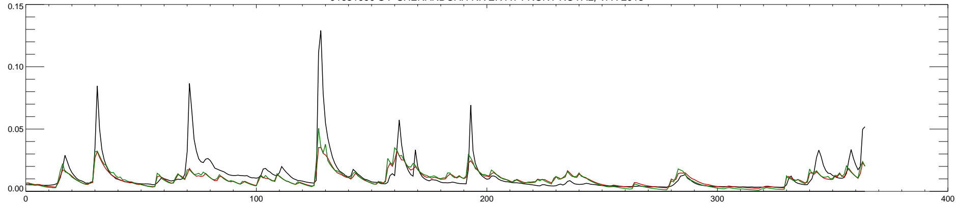
01631000 S F SHENANDOAH RIVER AT FRONT ROYAL, VA : 2013
