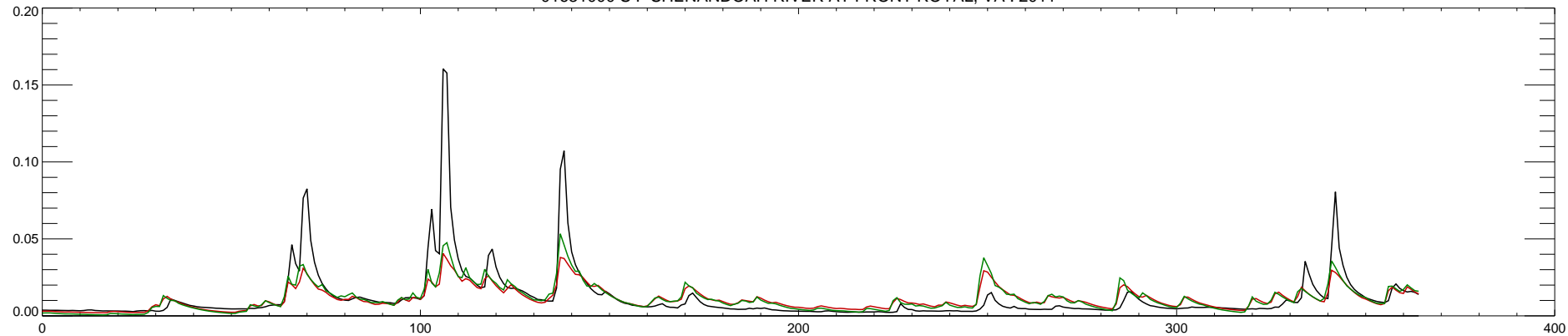
01631000 S F SHENANDOAH RIVER AT FRONT ROYAL, VA : 2012
