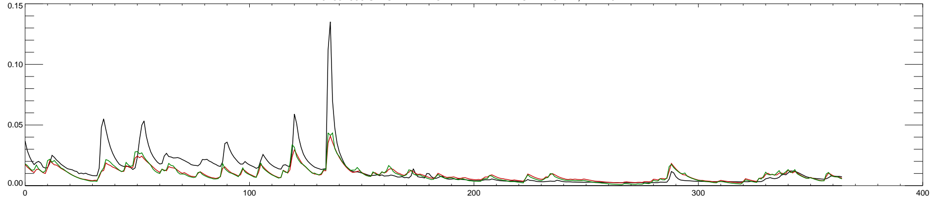
01631000 S F SHENANDOAH RIVER AT FRONT ROYAL, VA : 2015
