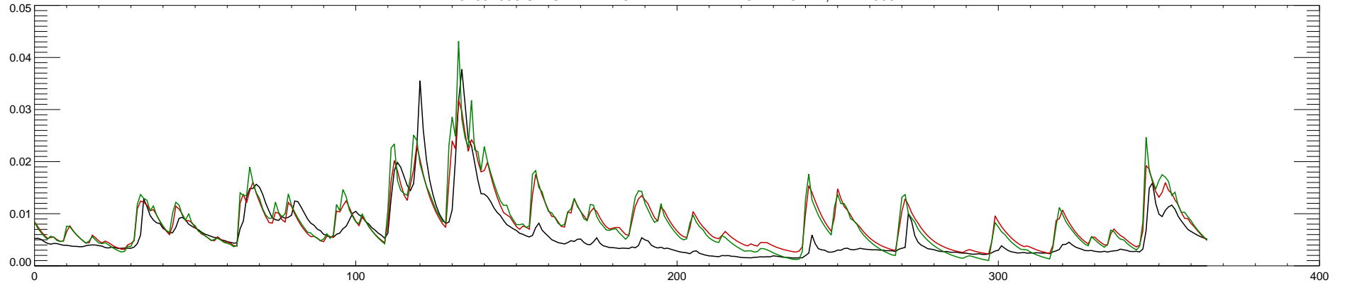
01631000 S F SHENANDOAH RIVER AT FRONT ROYAL, VA : 2009
