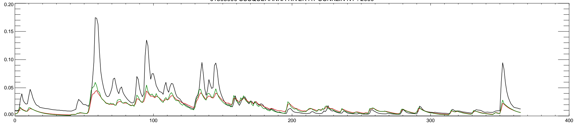
01503000 SUSQUEHANNA RIVER AT CONKLIN NY : 2001
