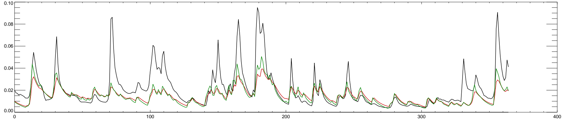
01503000 SUSQUEHANNA RIVER AT CONKLIN NY : 2013
