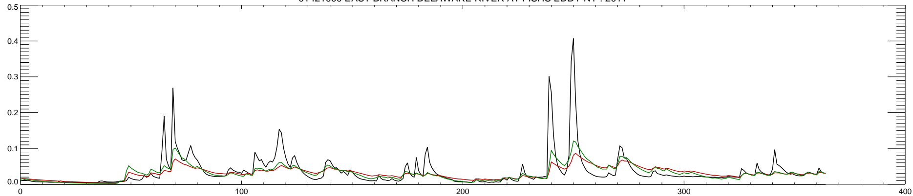
01421000 EAST BRANCH DELAWARE RIVER AT FISHS EDDY NY : 2012
