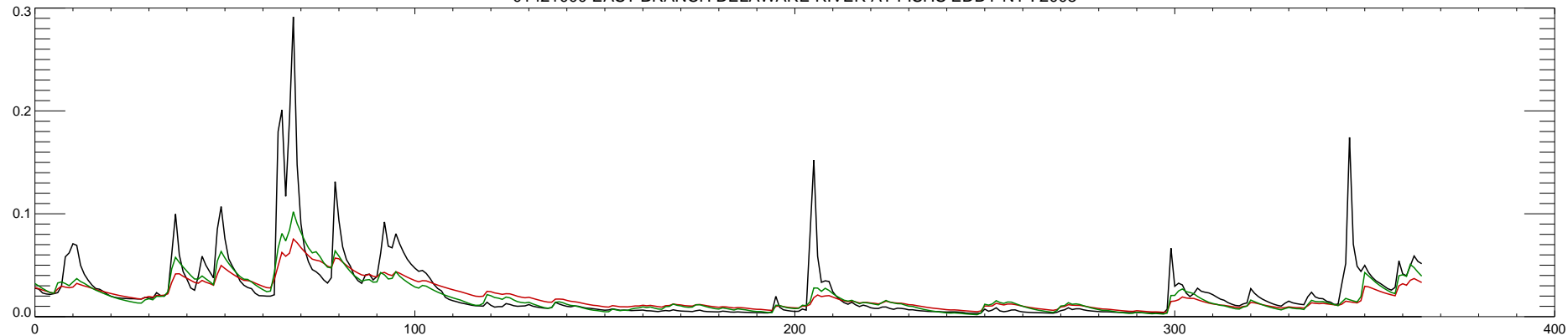
01421000 EAST BRANCH DELAWARE RIVER AT FISHS EDDY NY : 2009
