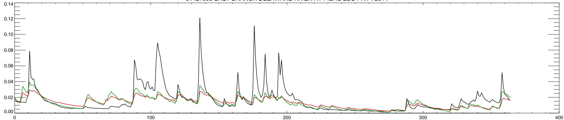
01421000 EAST BRANCH DELAWARE RIVER AT FISHS EDDY NY : 2015
