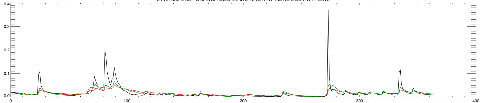
01421000 EAST BRANCH DELAWARE RIVER AT FISHS EDDY NY : 2010
