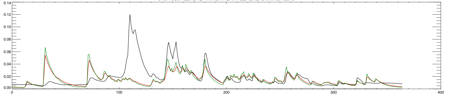
01011000 ALLAGASH RIVER NEAR ALLAGASH, MAINE : 2013
