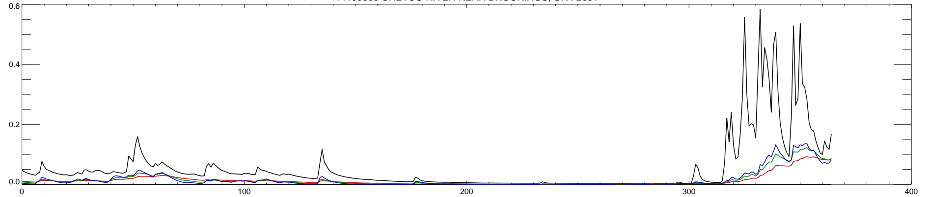
14400000 CHETCO RIVER NEAR BROOKINGS, OR : 2001
