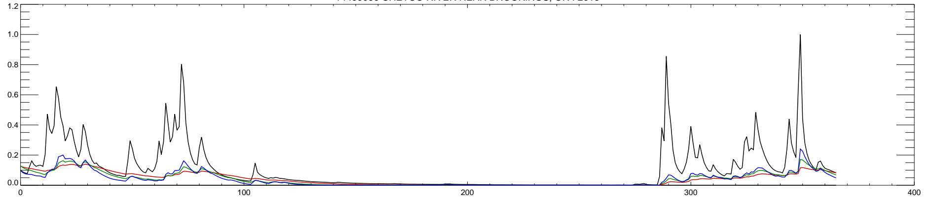
14400000 CHETCO RIVER NEAR BROOKINGS, OR : 2016
