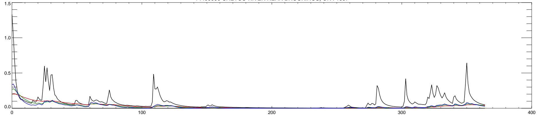
14400000 CHETCO RIVER NEAR BROOKINGS, OR : 1998
