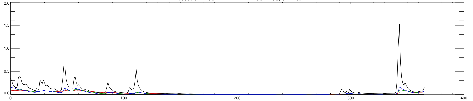
14400000 CHETCO RIVER NEAR BROOKINGS, OR : 2004
