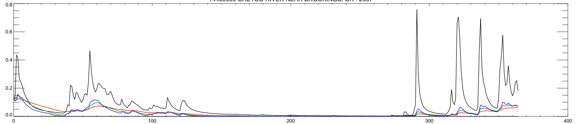
14400000 CHETCO RIVER NEAR BROOKINGS, OR : 2007
