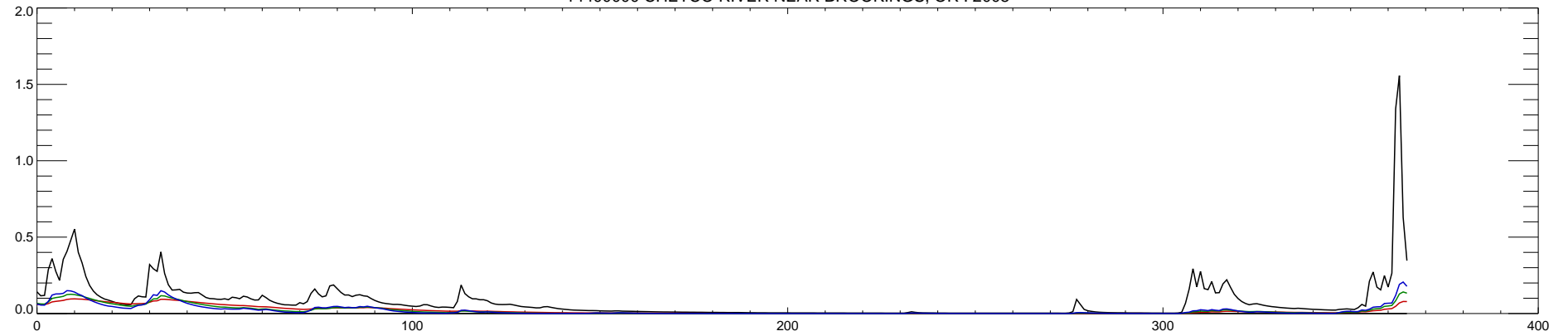
14400000 CHETCO RIVER NEAR BROOKINGS, OR : 2009
