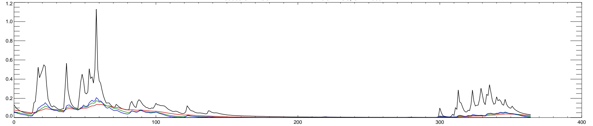
14400000 CHETCO RIVER NEAR BROOKINGS, OR : 2000
