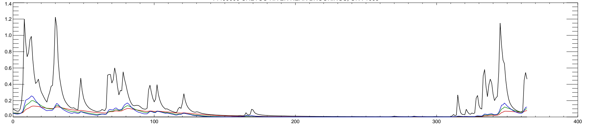
14400000 CHETCO RIVER NEAR BROOKINGS, OR : 1995
