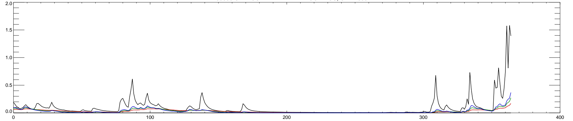
14400000 CHETCO RIVER NEAR BROOKINGS, OR : 2006
