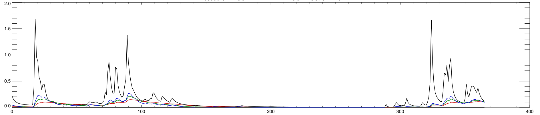
14400000 CHETCO RIVER NEAR BROOKINGS, OR : 2013
