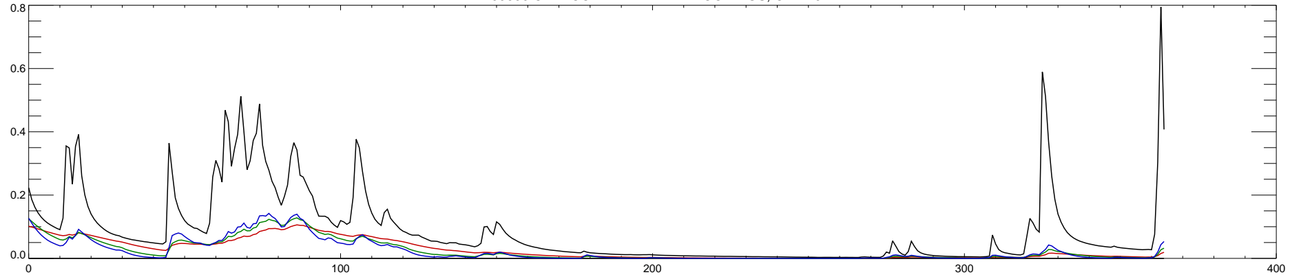
14400000 CHETCO RIVER NEAR BROOKINGS, OR : 2012
