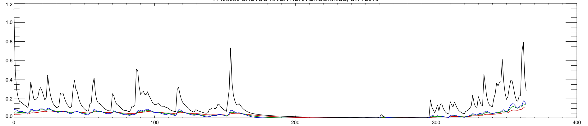
14400000 CHETCO RIVER NEAR BROOKINGS, OR : 2010
