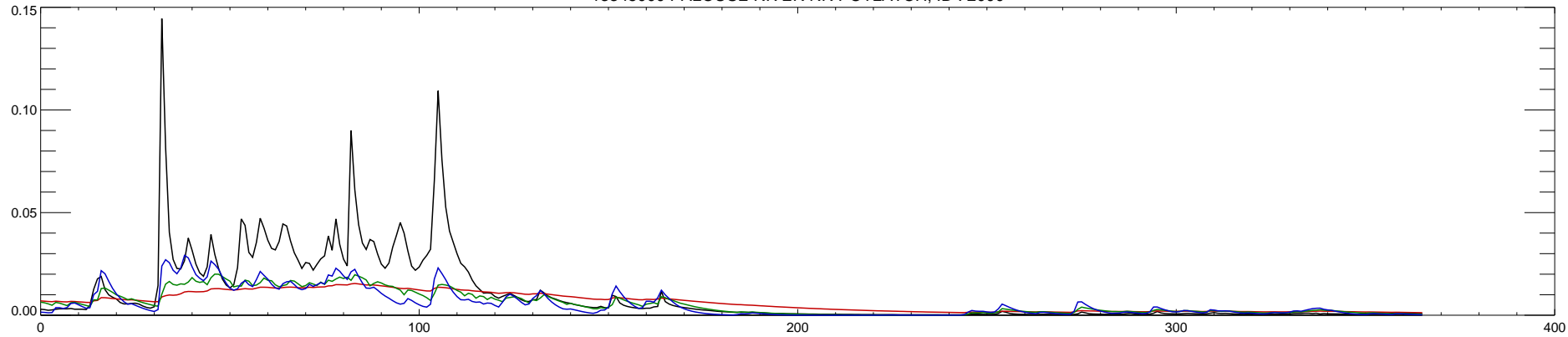
13345000 PALOUSE RIVER NR POTLATCH, ID : 2001
