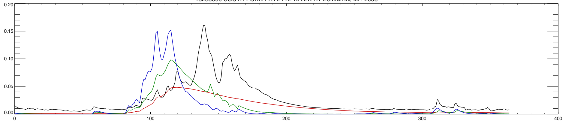
13235000 SOUTH FORK PAYETTE RIVER AT LOWMAN, ID : 2007
