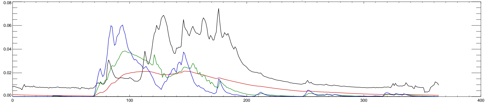
13235000 SOUTH FORK PAYETTE RIVER AT LOWMAN, ID : 1998
