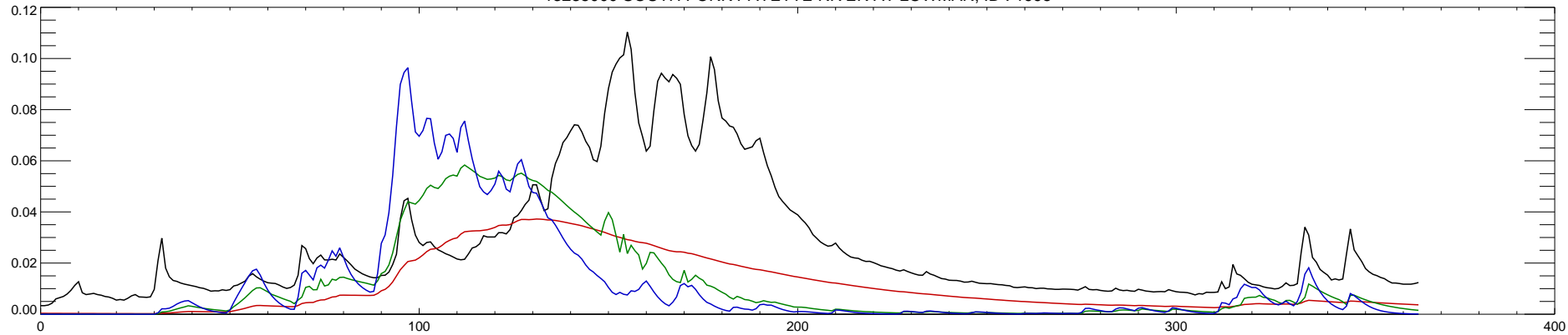
13235000 SOUTH FORK PAYETTE RIVER AT LOWMAN, ID : 1995
