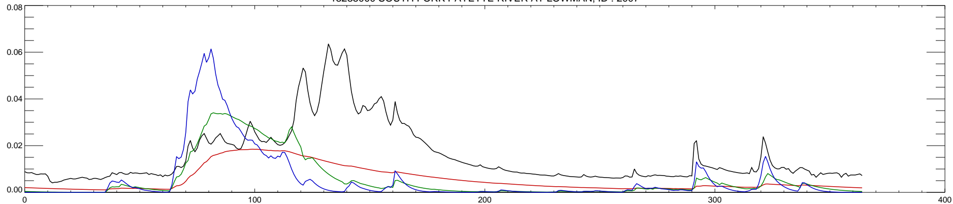
13235000 SOUTH FORK PAYETTE RIVER AT LOWMAN, ID : 2007
