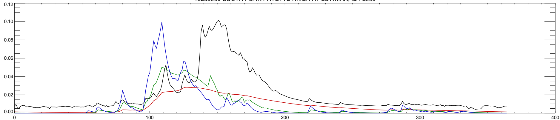
13235000 SOUTH FORK PAYETTE RIVER AT LOWMAN, ID : 2010
