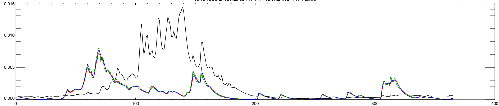
13161500 BRUNEAU RV AT ROWLAND, NV : 2009
