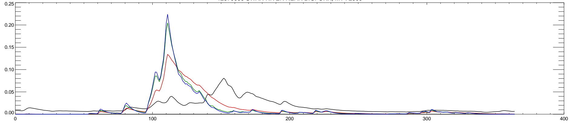
12370000 SWAN RIVER NEAR BIGFORK, MT : 2010
