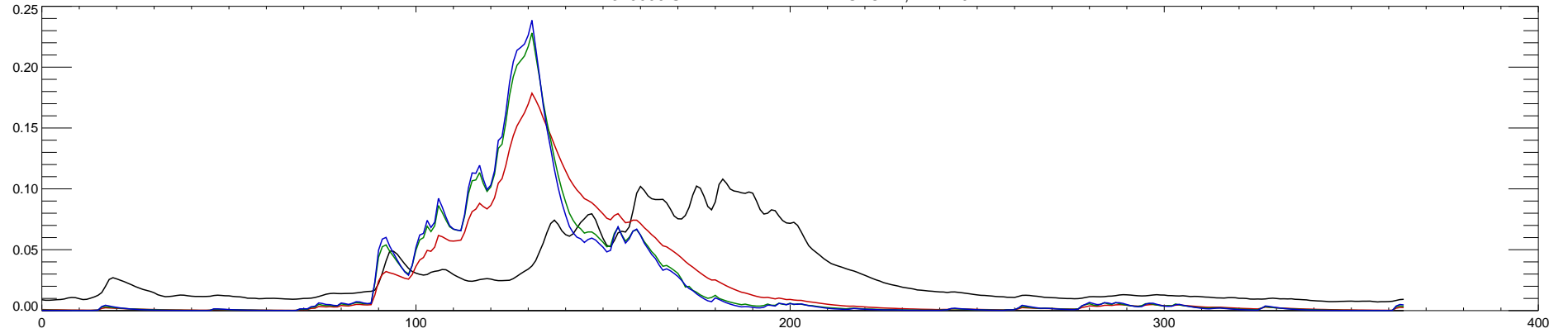
12370000 SWAN RIVER NEAR BIGFORK, MT : 2012
