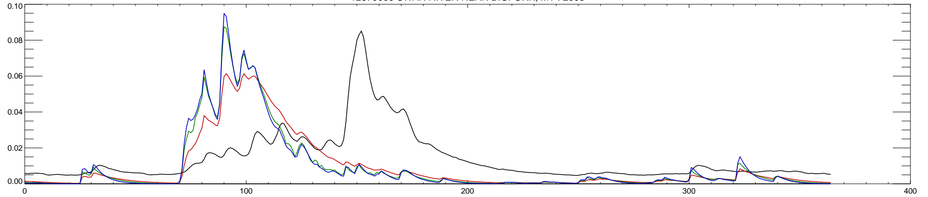
12370000 SWAN RIVER NEAR BIGFORK, MT : 2004
