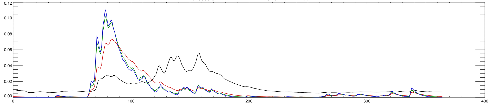
12370000 SWAN RIVER NEAR BIGFORK, MT : 2007
