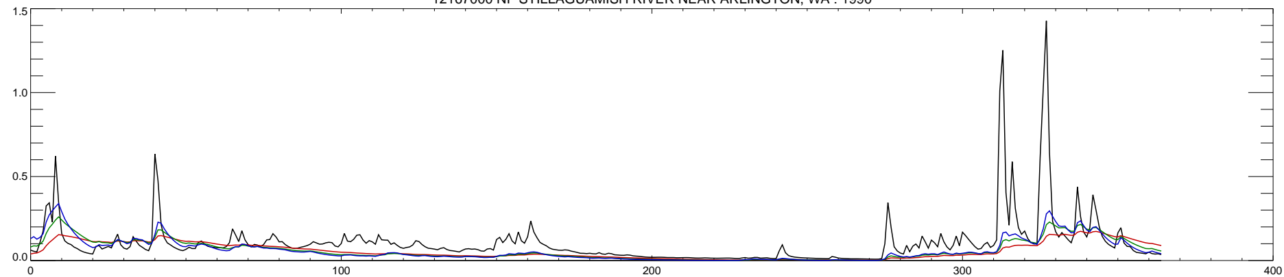
12167000 NF STILLAGUAMISH RIVER NEAR ARLINGTON, WA : 1991
