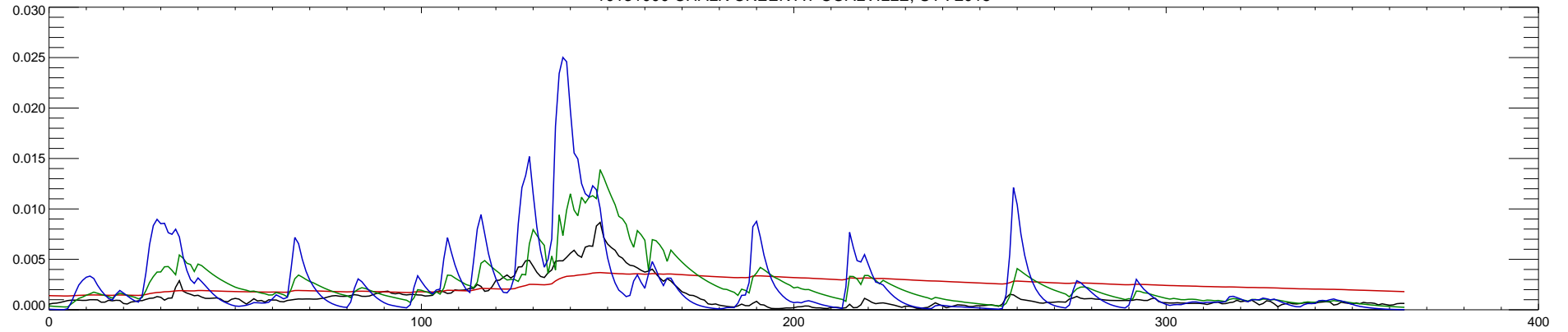
10131000 CHALK CREEK AT COALVILLE, UT : 2016
