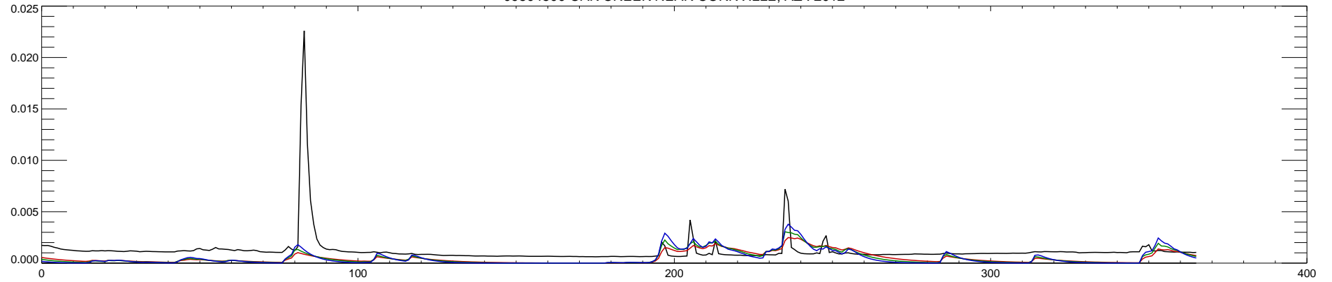
09504500 OAK CREEK NEAR CORNVILLE, AZ : 2013
