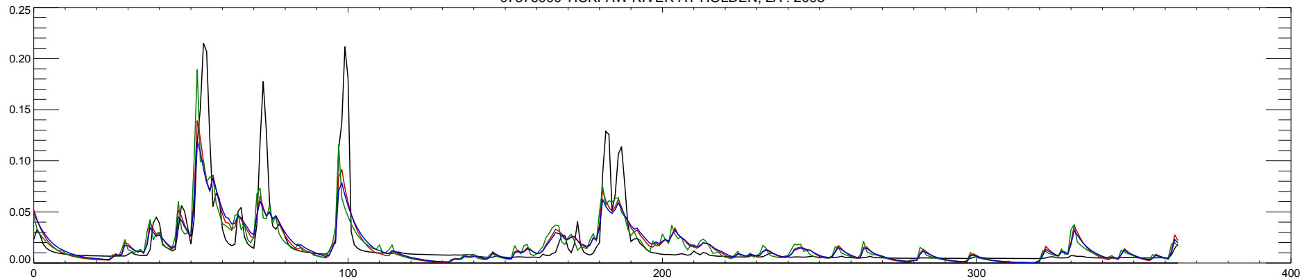
07376000 TICKFAW RIVER AT HOLDEN, LA : 2004
