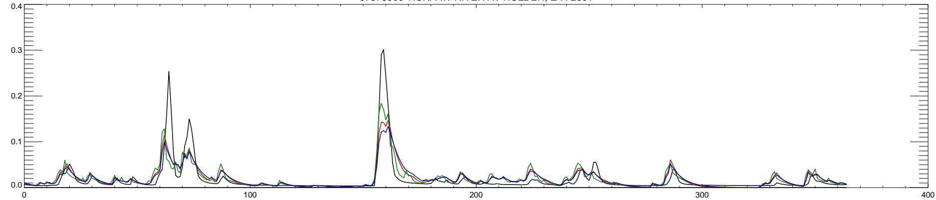
07376000 TICKFAW RIVER AT HOLDEN, LA : 2001
