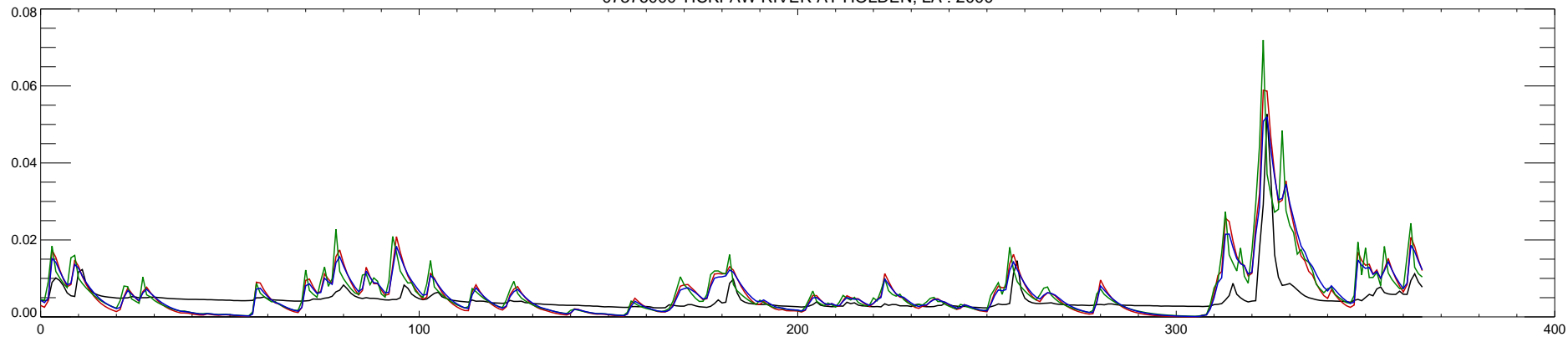
07376000 TICKFAW RIVER AT HOLDEN, LA : 2001
