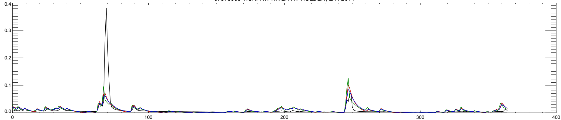
07376000 TICKFAW RIVER AT HOLDEN, LA : 2012
