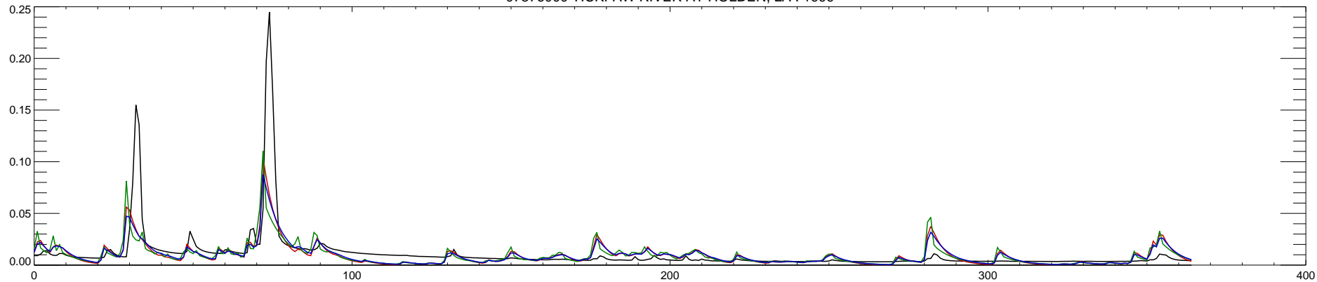
07376000 TICKFAW RIVER AT HOLDEN, LA : 2000
