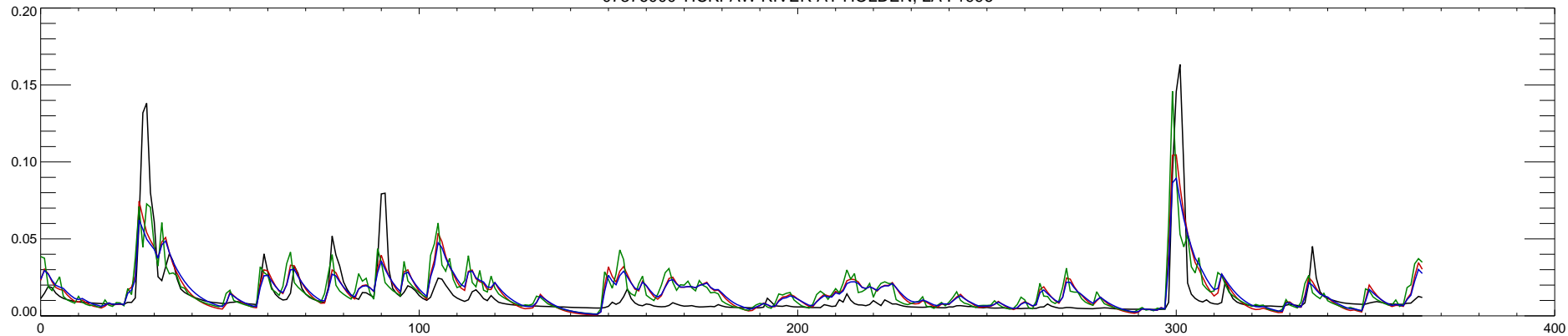
07376000 TICKFAW RIVER AT HOLDEN, LA : 1997
