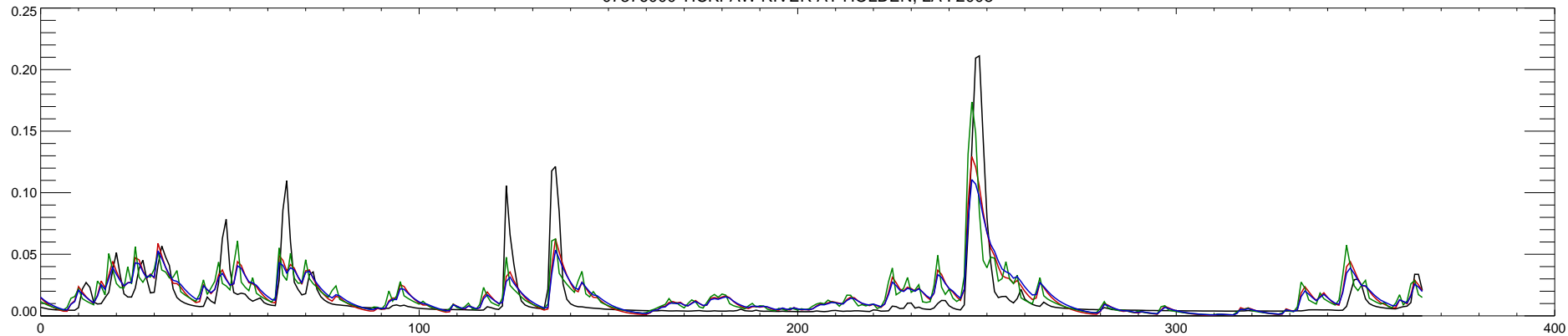
07376000 TICKFAW RIVER AT HOLDEN, LA : 2009
