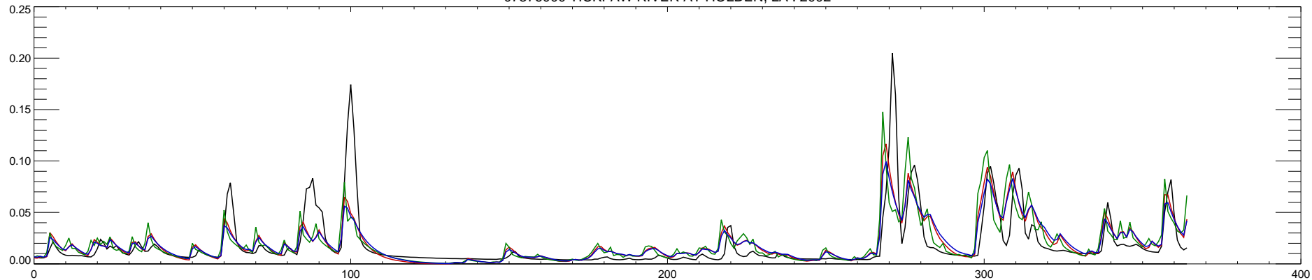
07376000 TICKFAW RIVER AT HOLDEN, LA : 2003
