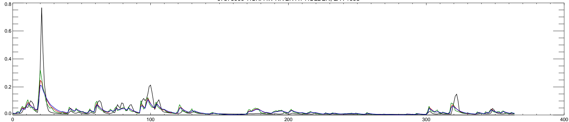
07376000 TICKFAW RIVER AT HOLDEN, LA : 1994
