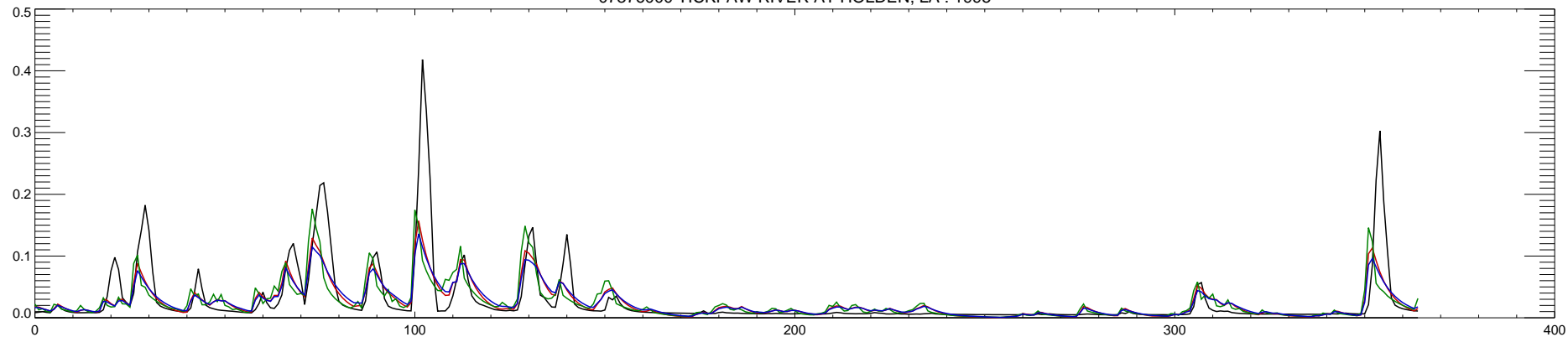
07376000 TICKFAW RIVER AT HOLDEN, LA : 1995
