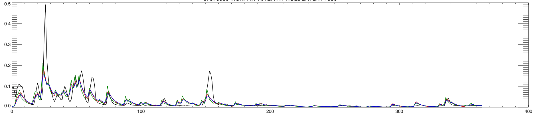
07376000 TICKFAW RIVER AT HOLDEN, LA : 1991
