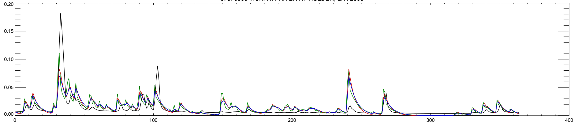
07376000 TICKFAW RIVER AT HOLDEN, LA : 2006
