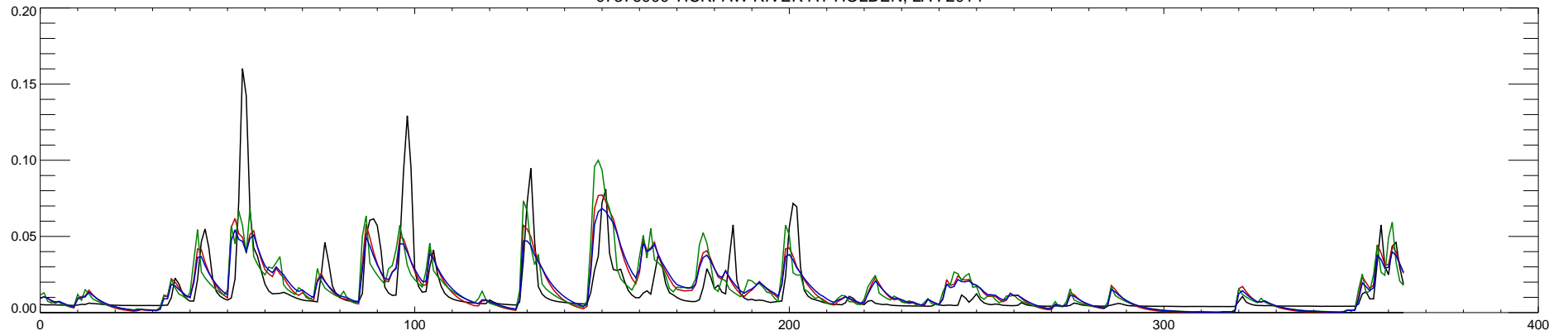
07376000 TICKFAW RIVER AT HOLDEN, LA : 2015
