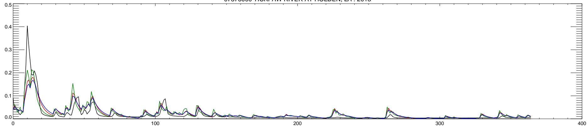
07376000 TICKFAW RIVER AT HOLDEN, LA : 2013
