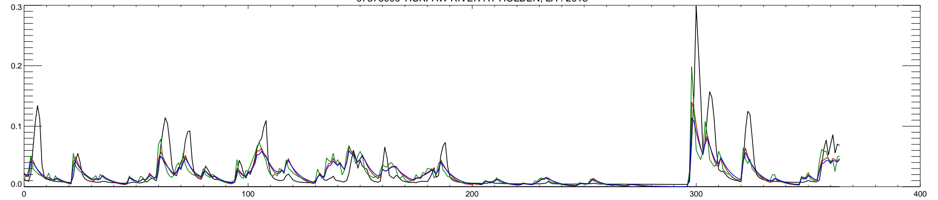
07376000 TICKFAW RIVER AT HOLDEN, LA : 2016
