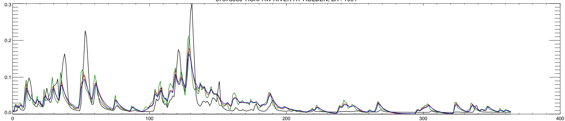
07376000 TICKFAW RIVER AT HOLDEN, LA : 1992
