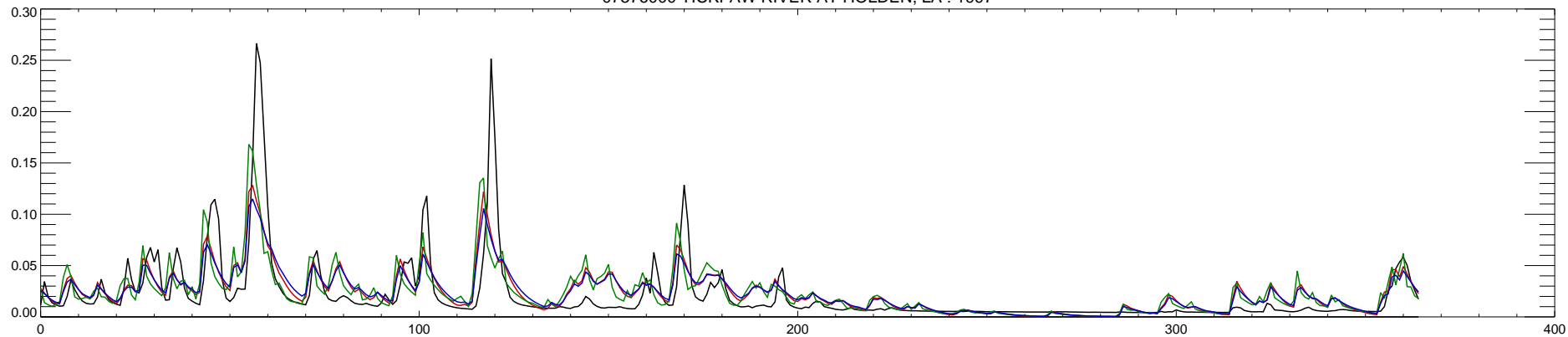
07376000 TICKFAW RIVER AT HOLDEN, LA : 1998
