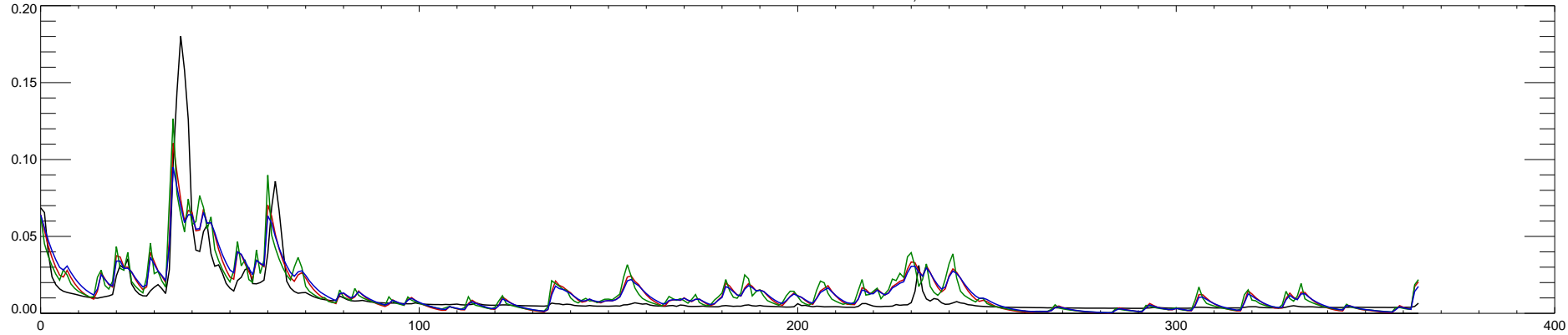
07376000 TICKFAW RIVER AT HOLDEN, LA : 2010
