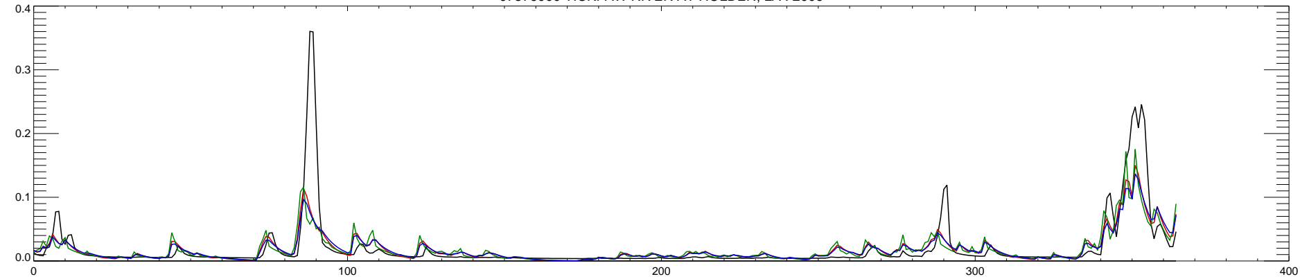
07376000 TICKFAW RIVER AT HOLDEN, LA : 2010
