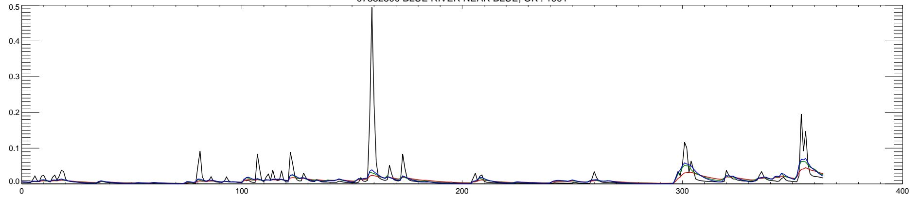
07332500 BLUE RIVER NEAR BLUE, OK : 1992
