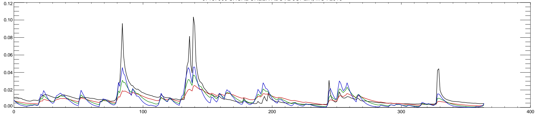
07187000 SHOAL CREEK ABOVE JOPLIN, MO : 2010
