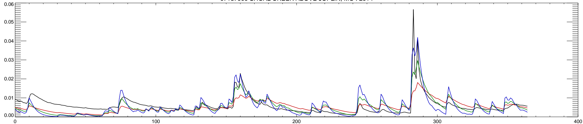
07187000 SHOAL CREEK ABOVE JOPLIN, MO : 2015
