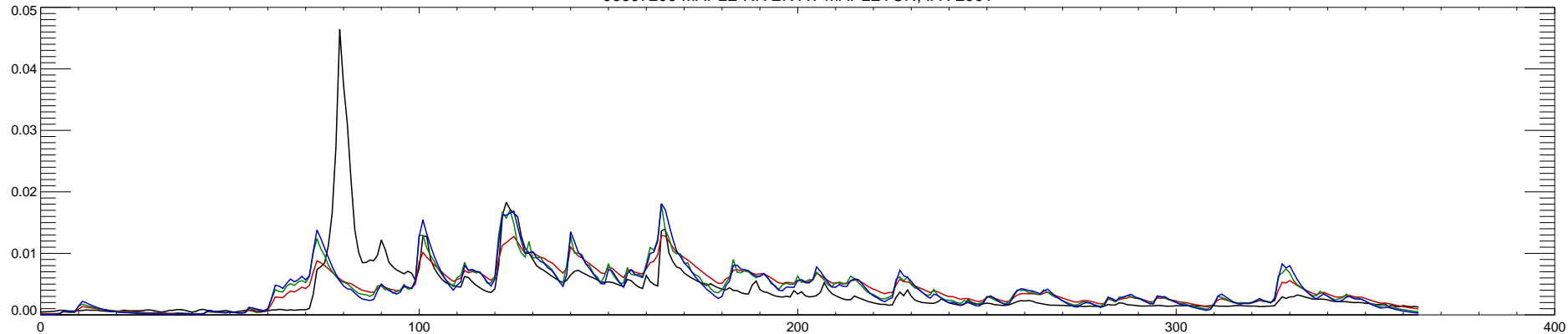
06607200 MAPLE RIVER AT MAPLETON, IA : 2001
