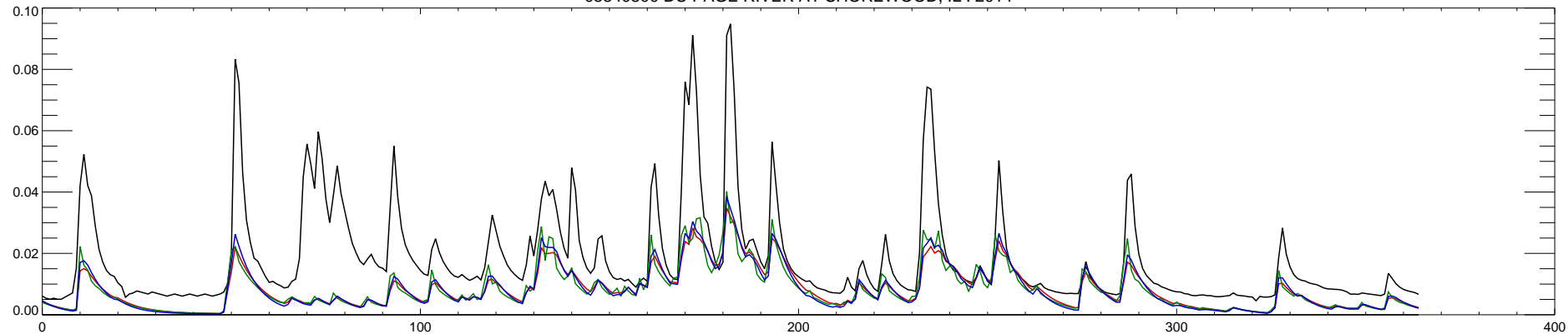
05540500 DU PAGE RIVER AT SHOREWOOD, IL : 2015
