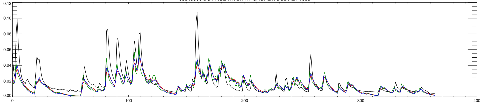
05540500 DU PAGE RIVER AT SHOREWOOD, IL : 1994
