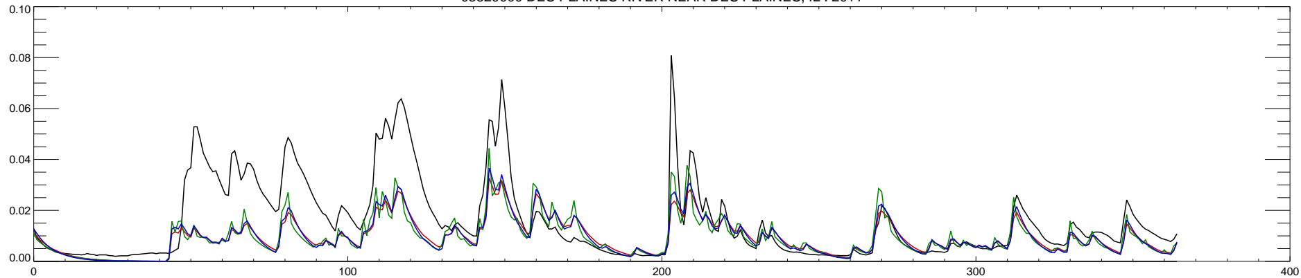
05529000 DES PLAINES RIVER NEAR DES PLAINES, IL : 2012
