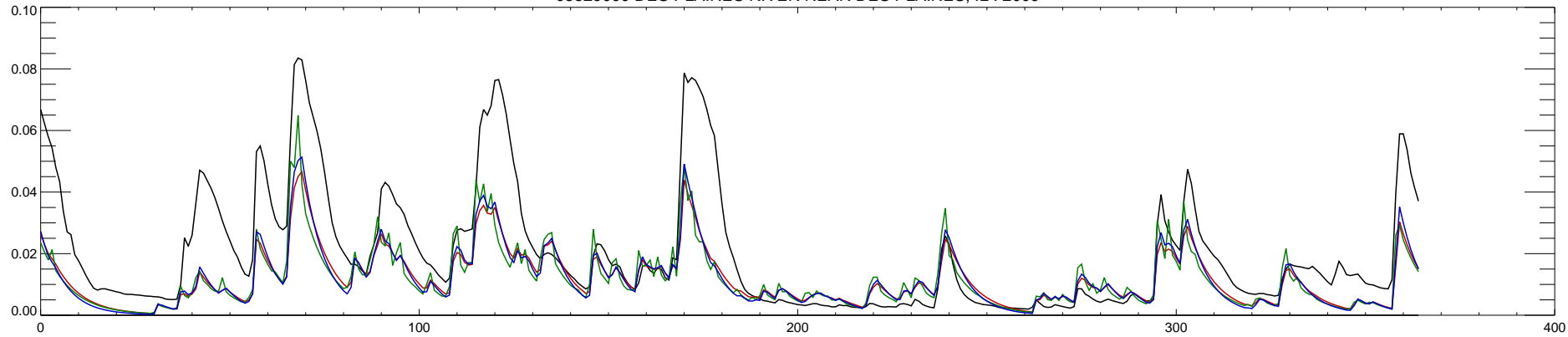
05529000 DES PLAINES RIVER NEAR DES PLAINES, IL : 2010
