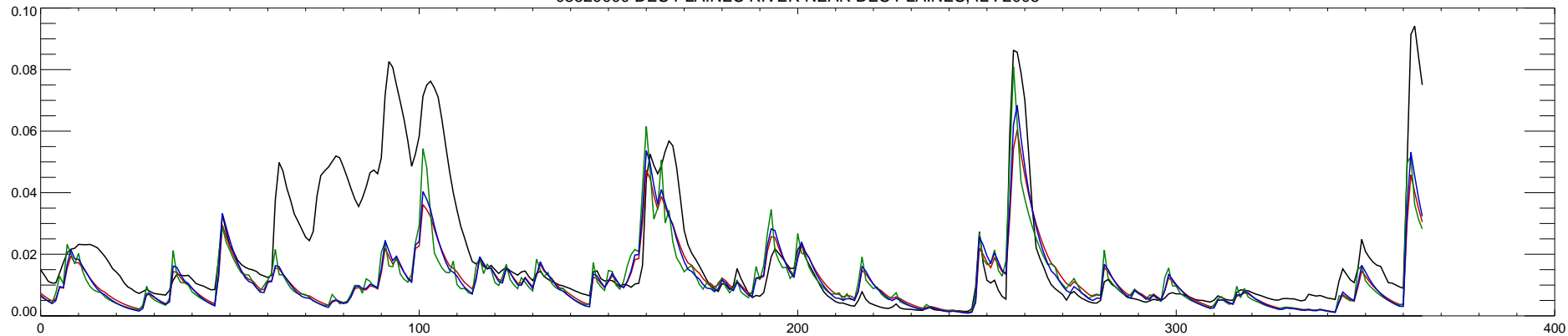
05529000 DES PLAINES RIVER NEAR DES PLAINES, IL : 2009
