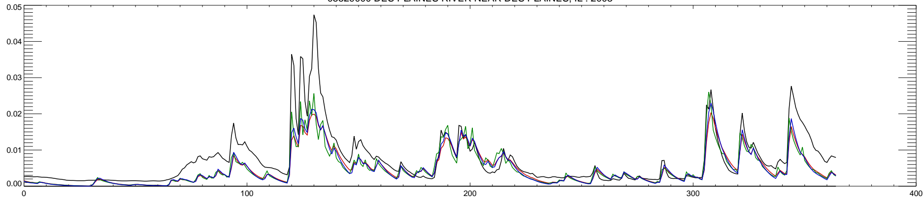
05529000 DES PLAINES RIVER NEAR DES PLAINES, IL : 2004
