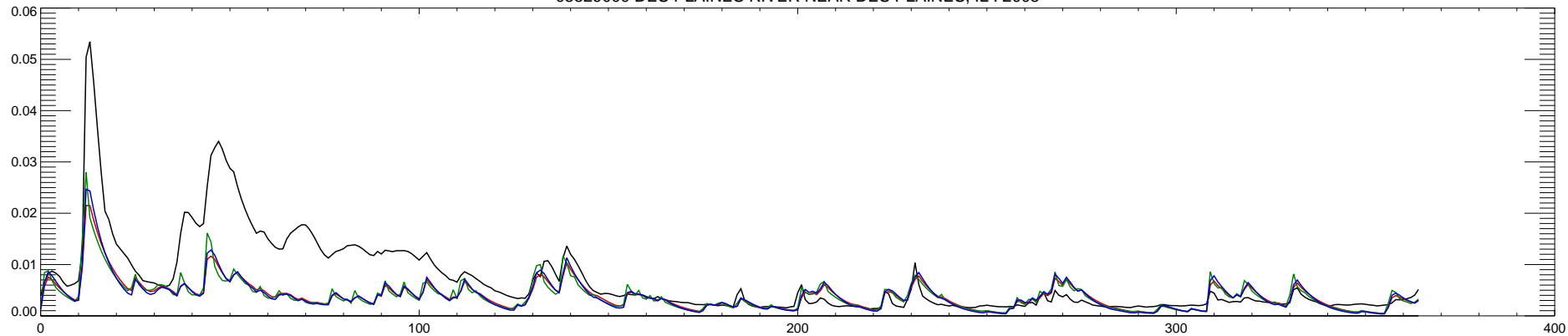
05529000 DES PLAINES RIVER NEAR DES PLAINES, IL : 2006
