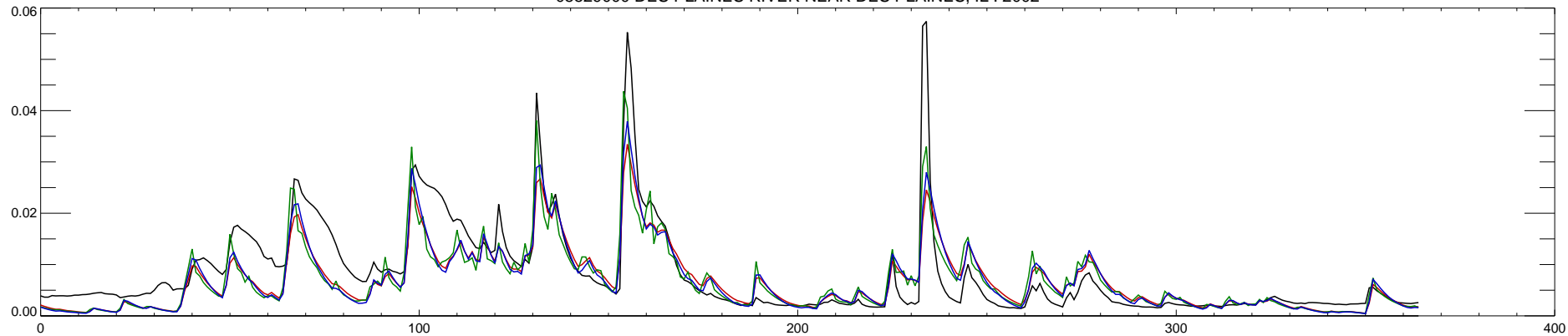
05529000 DES PLAINES RIVER NEAR DES PLAINES, IL : 2003
