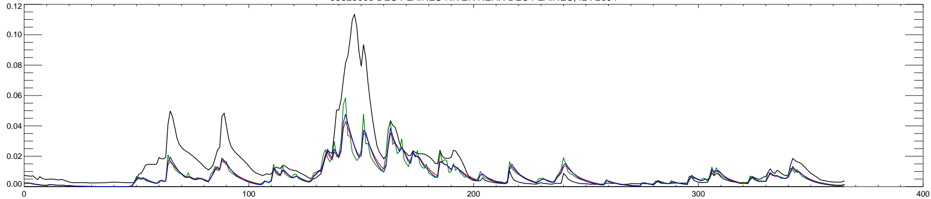
05529000 DES PLAINES RIVER NEAR DES PLAINES, IL : 2004
