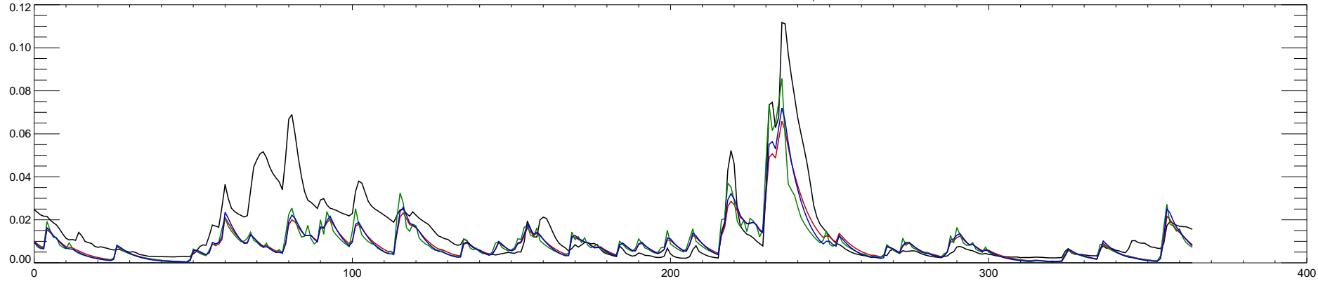
05529000 DES PLAINES RIVER NEAR DES PLAINES, IL : 2007
