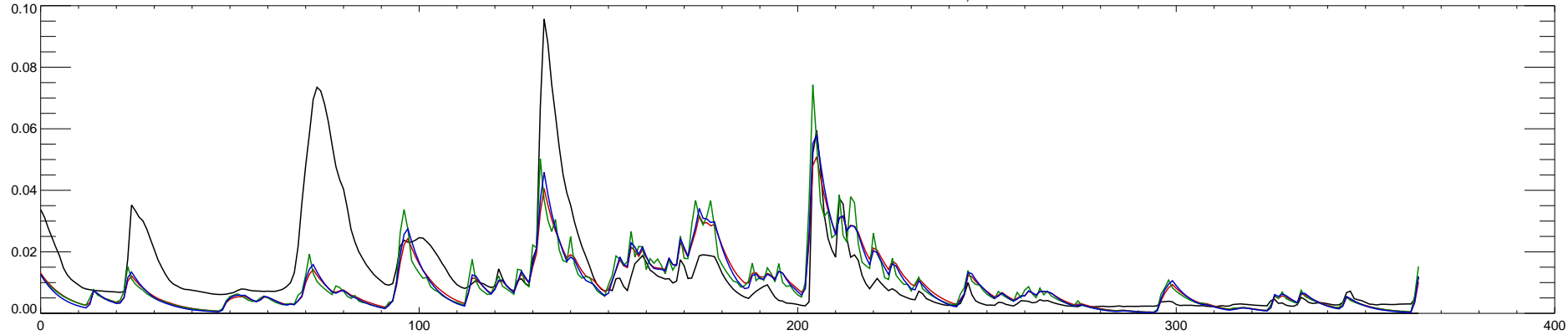
05529000 DES PLAINES RIVER NEAR DES PLAINES, IL : 2010
