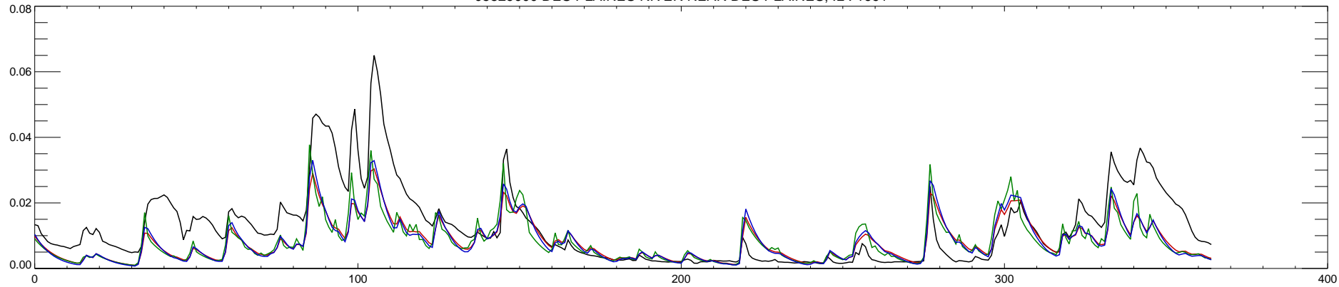
05529000 DES PLAINES RIVER NEAR DES PLAINES, IL : 1992
