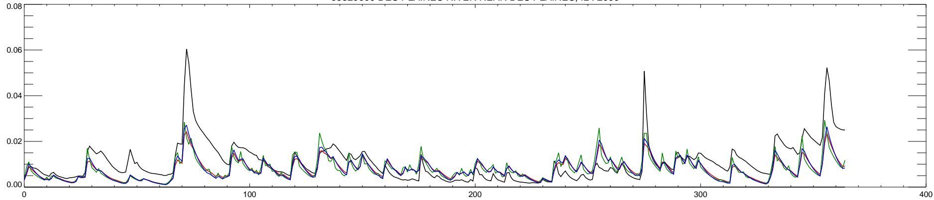
05529000 DES PLAINES RIVER NEAR DES PLAINES, IL : 2007
