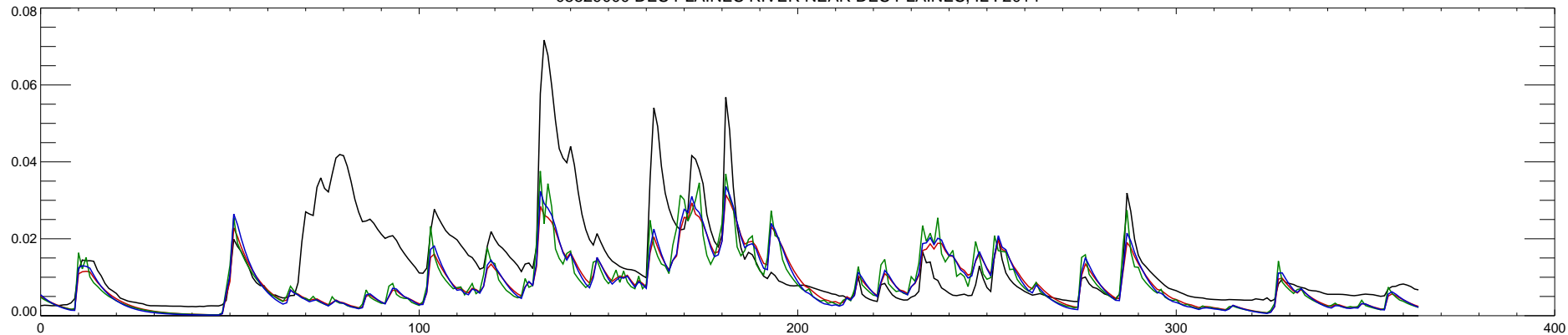
05529000 DES PLAINES RIVER NEAR DES PLAINES, IL : 2015
