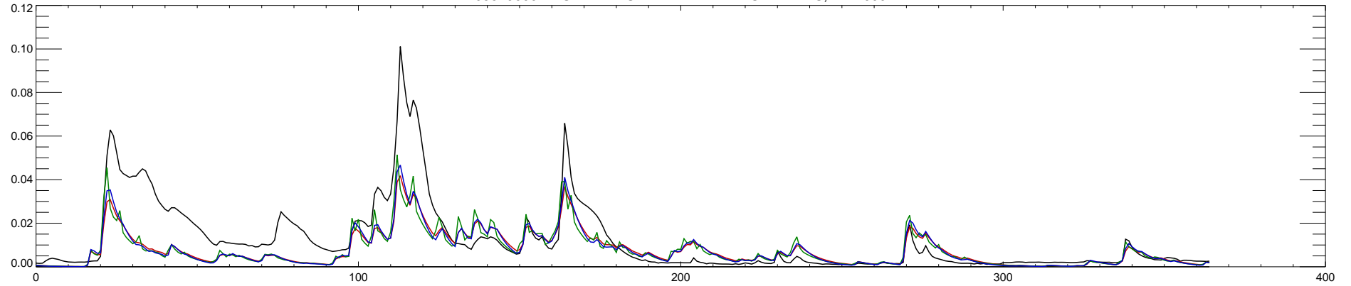
05529000 DES PLAINES RIVER NEAR DES PLAINES, IL : 2000
