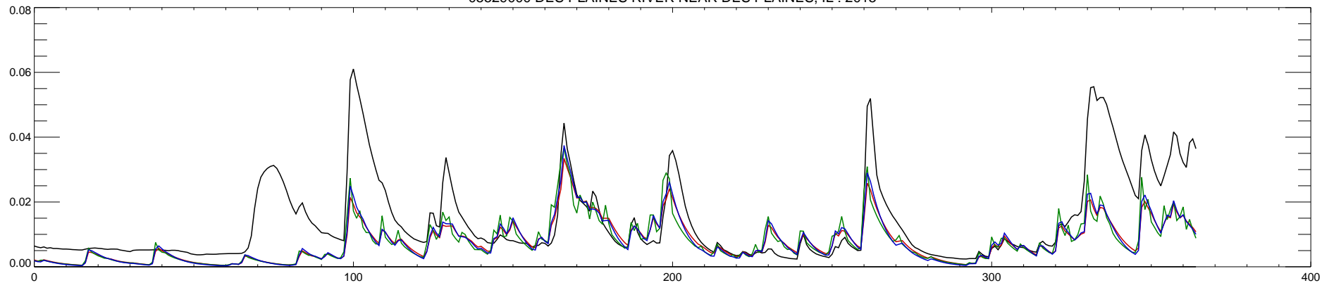
05529000 DES PLAINES RIVER NEAR DES PLAINES, IL : 2016
