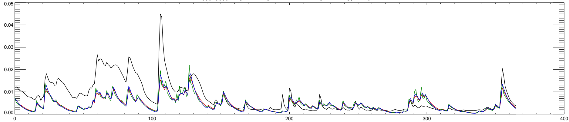
05529000 DES PLAINES RIVER NEAR DES PLAINES, IL : 2013
