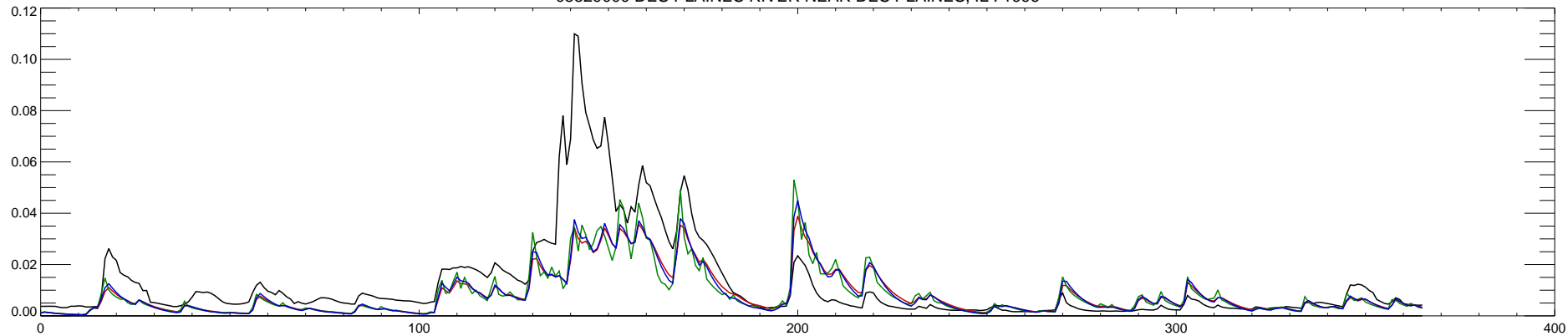
05529000 DES PLAINES RIVER NEAR DES PLAINES, IL : 1997
