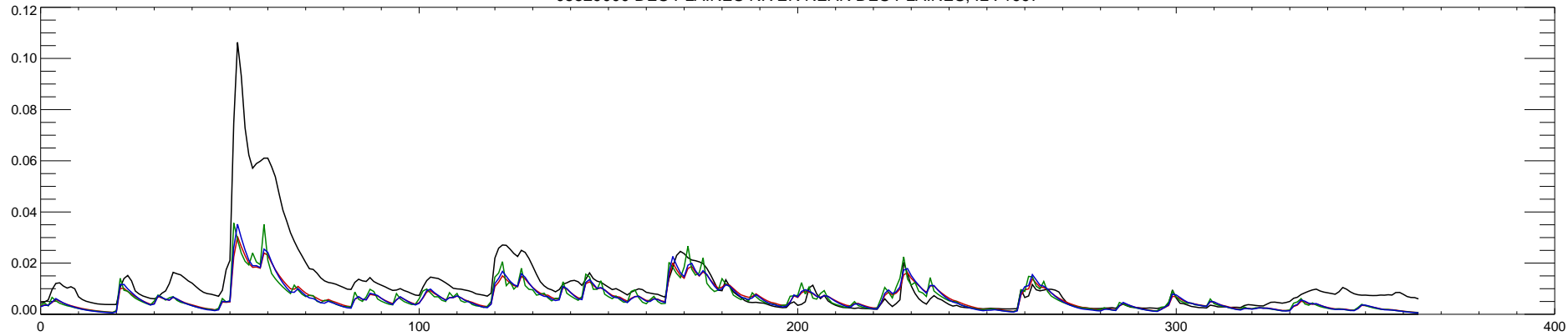
05529000 DES PLAINES RIVER NEAR DES PLAINES, IL : 1998
