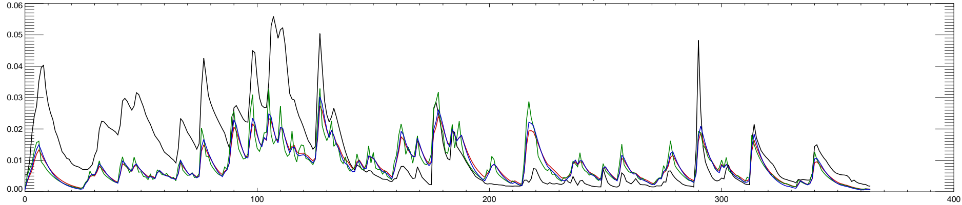
05529000 DES PLAINES RIVER NEAR DES PLAINES, IL : 1998
