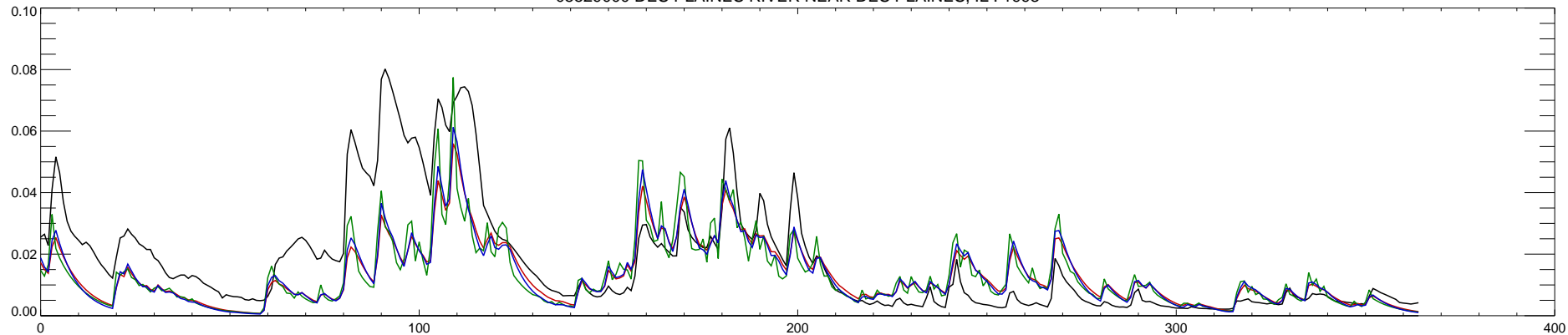
05529000 DES PLAINES RIVER NEAR DES PLAINES, IL : 1994
