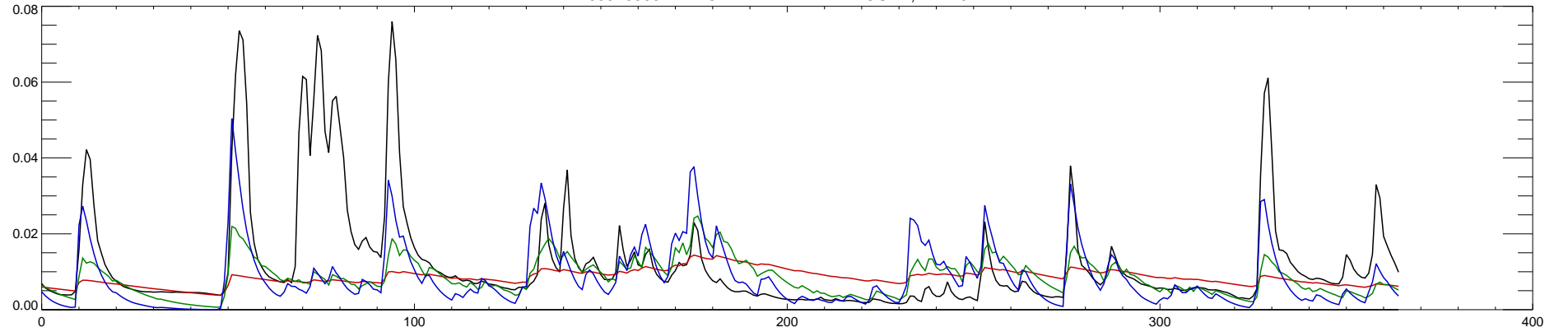
05516500 YELLOW RIVER AT PLYMOUTH, IN : 2015
