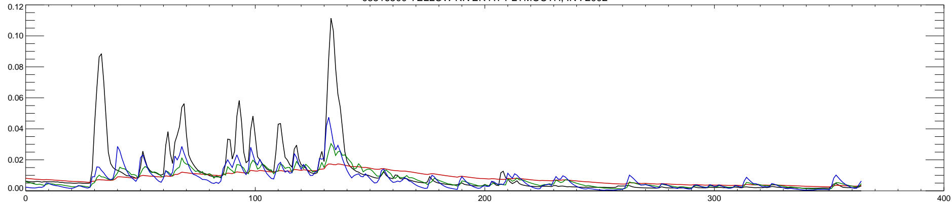
05516500 YELLOW RIVER AT PLYMOUTH, IN : 2003
