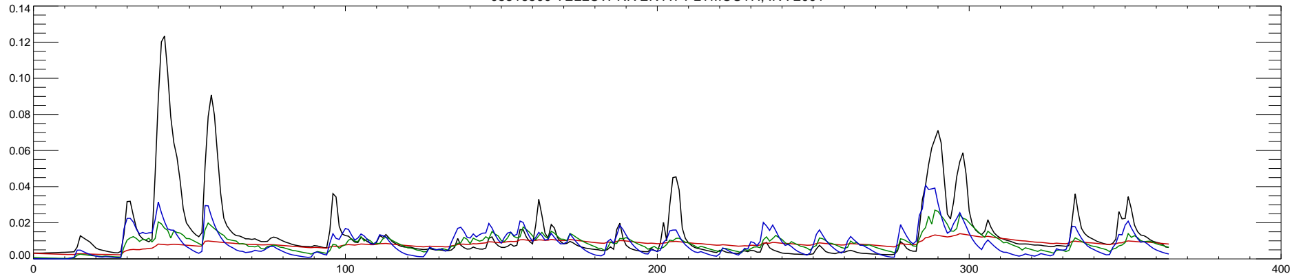
05516500 YELLOW RIVER AT PLYMOUTH, IN : 2001
