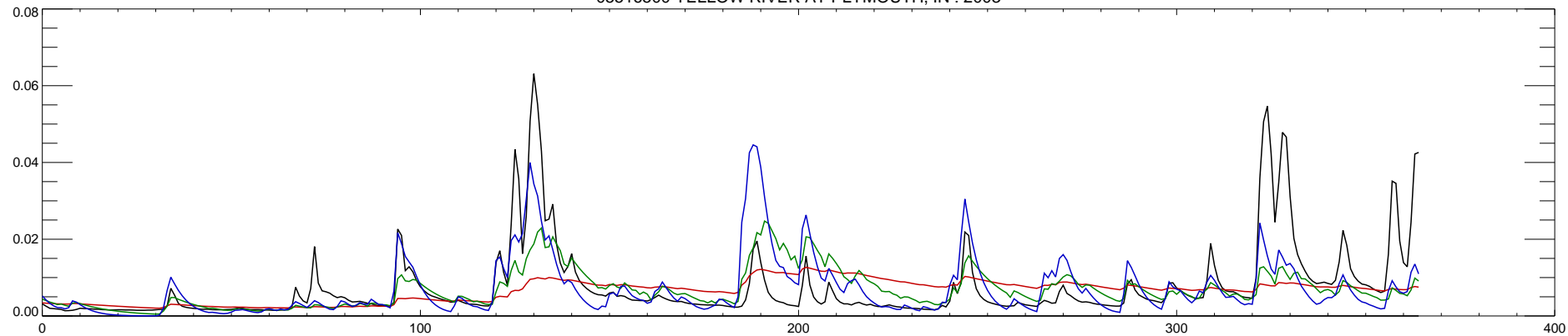
05516500 YELLOW RIVER AT PLYMOUTH, IN : 2004
