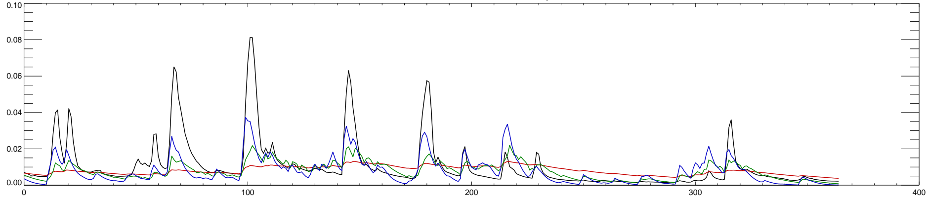
05516500 YELLOW RIVER AT PLYMOUTH, IN : 1995
