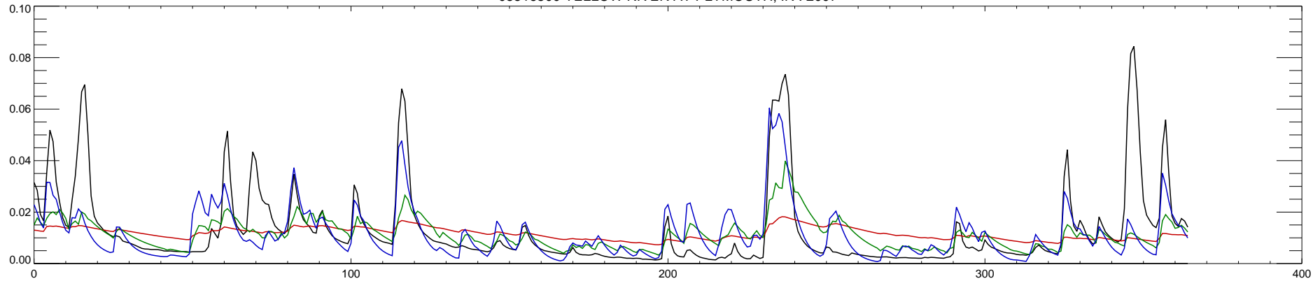
05516500 YELLOW RIVER AT PLYMOUTH, IN : 2007
