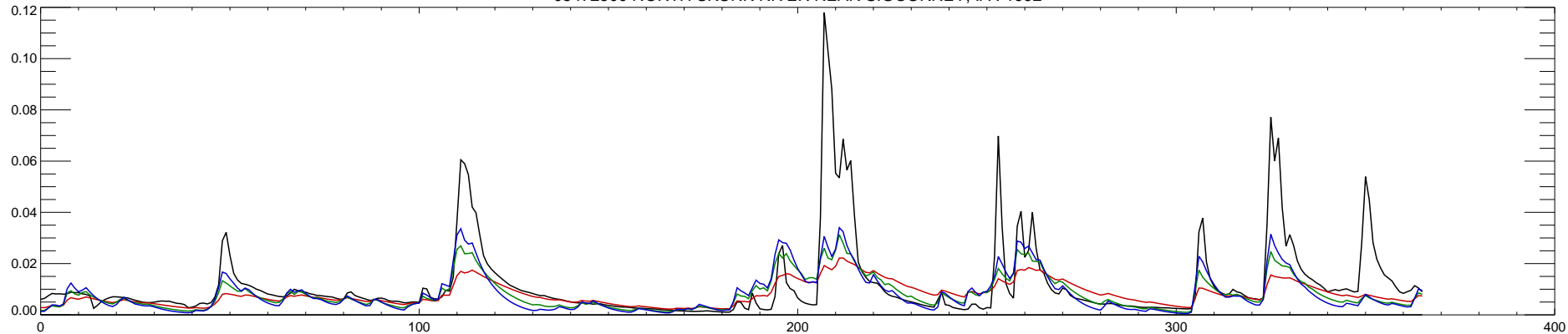
05472500 NORTH SKUNK RIVER NEAR SIGOURNEY, IA : 1992
