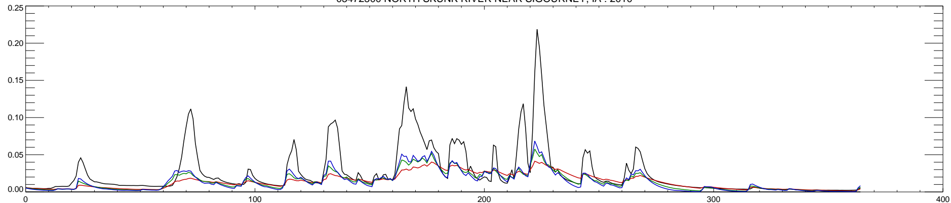
05472500 NORTH SKUNK RIVER NEAR SIGOURNEY, IA : 2010
