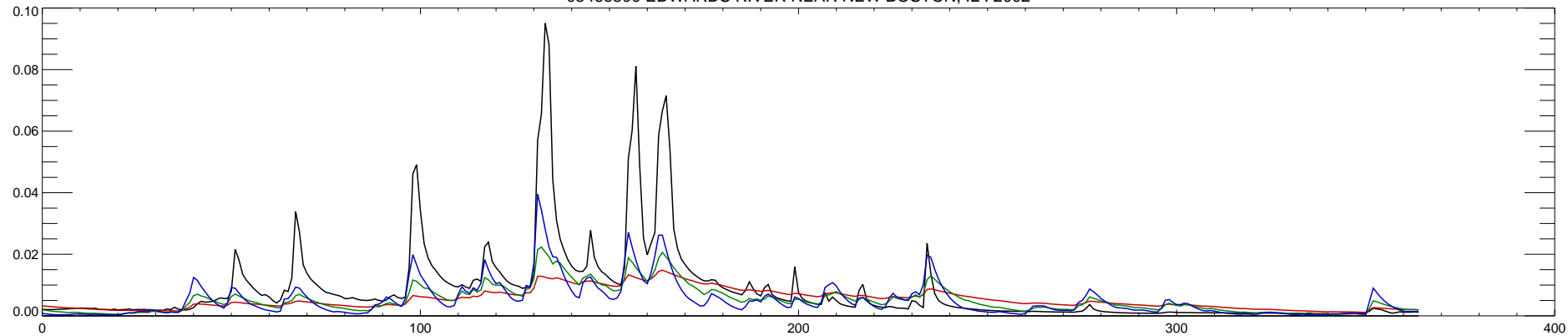
05466500 EDWARDS RIVER NEAR NEW BOSTON, IL : 2003
