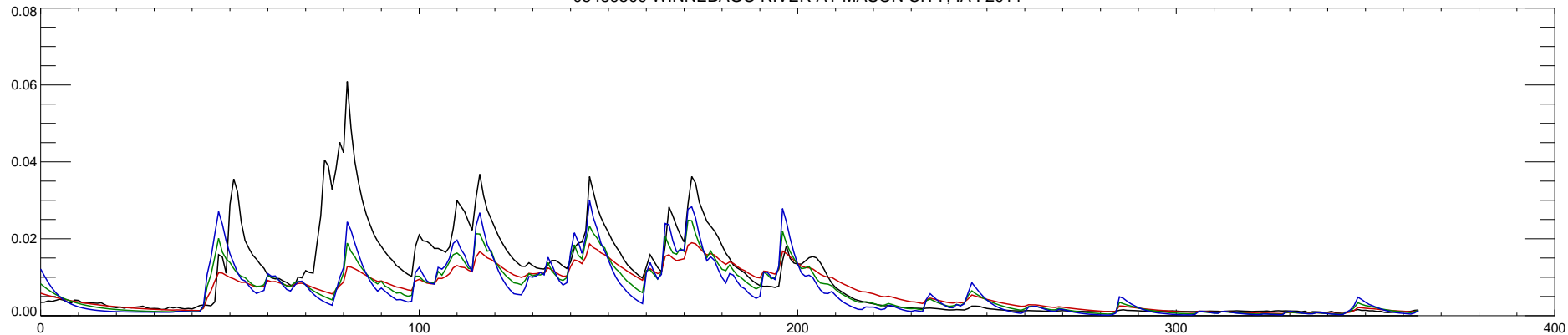
05459500 WINNEBAGO RIVER AT MASON CITY, IA : 2012
