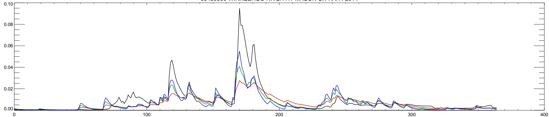
05459500 WINNEBAGO RIVER AT MASON CITY, IA : 2015
