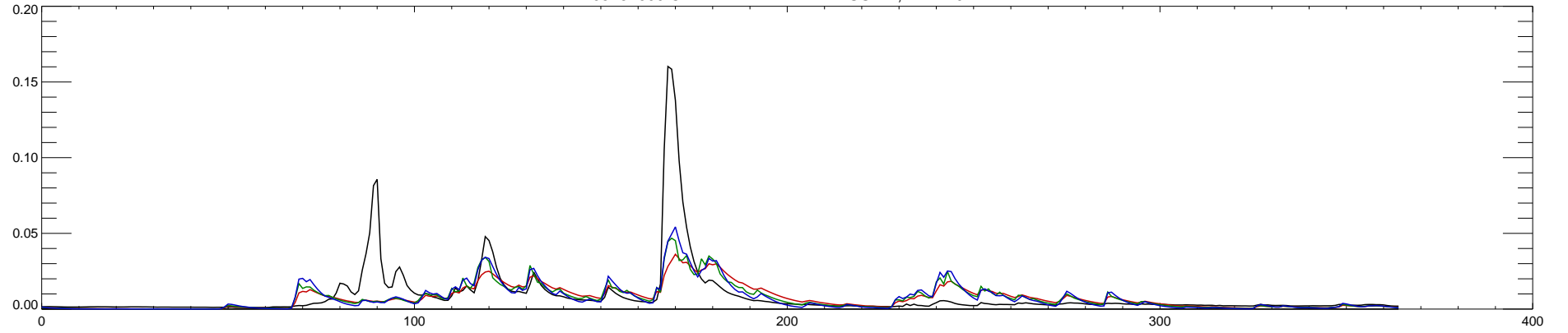
05457000 CEDAR RIVER NEAR AUSTIN, MN : 2015
