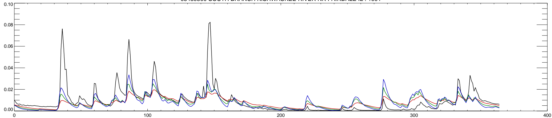
05439500 SOUTH BRANCH KISHWAUKEE RIVER NR FAIRDALE IL : 1992
