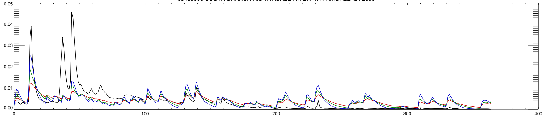
05439500 SOUTH BRANCH KISHWAUKEE RIVER NR FAIRDALE IL : 2006
