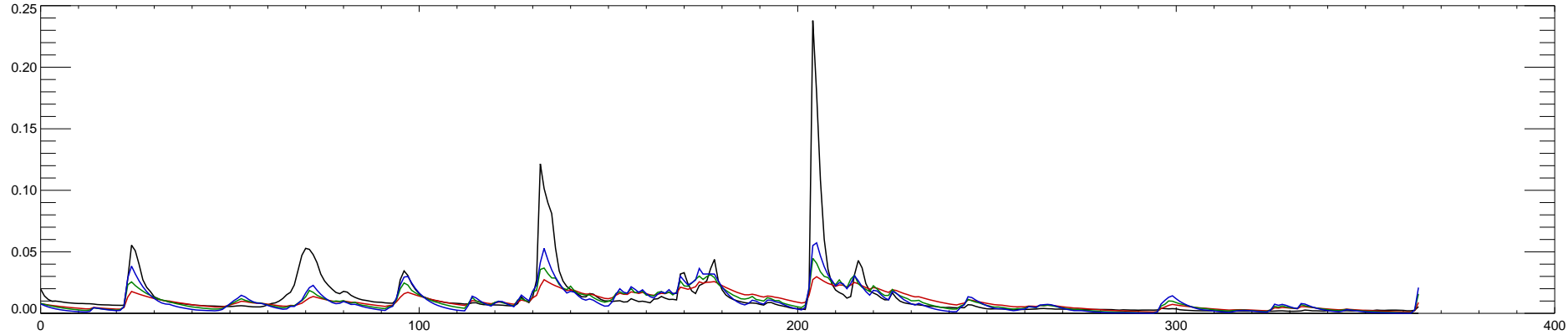
05439500 SOUTH BRANCH KISHWAUKEE RIVER NR FAIRDALE IL : 2010
