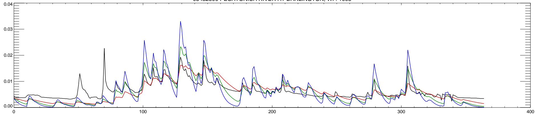
05432500 PECATONICA RIVER AT DARLINGTON, WI : 1995
