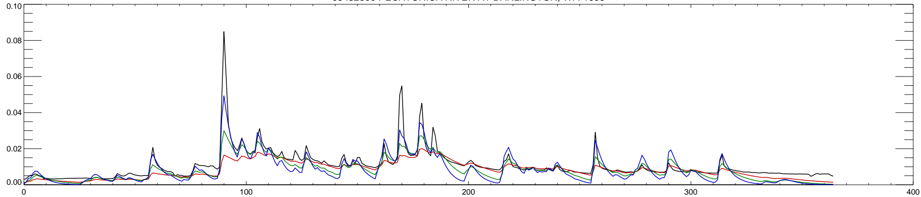
05432500 PECATONICA RIVER AT DARLINGTON, WI : 1998
