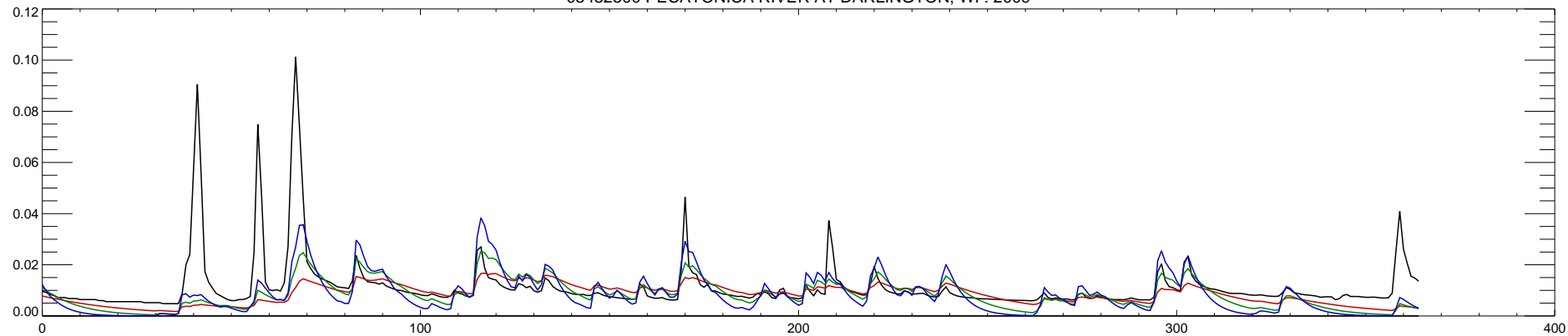
05432500 PECATONICA RIVER AT DARLINGTON, WI : 2010
