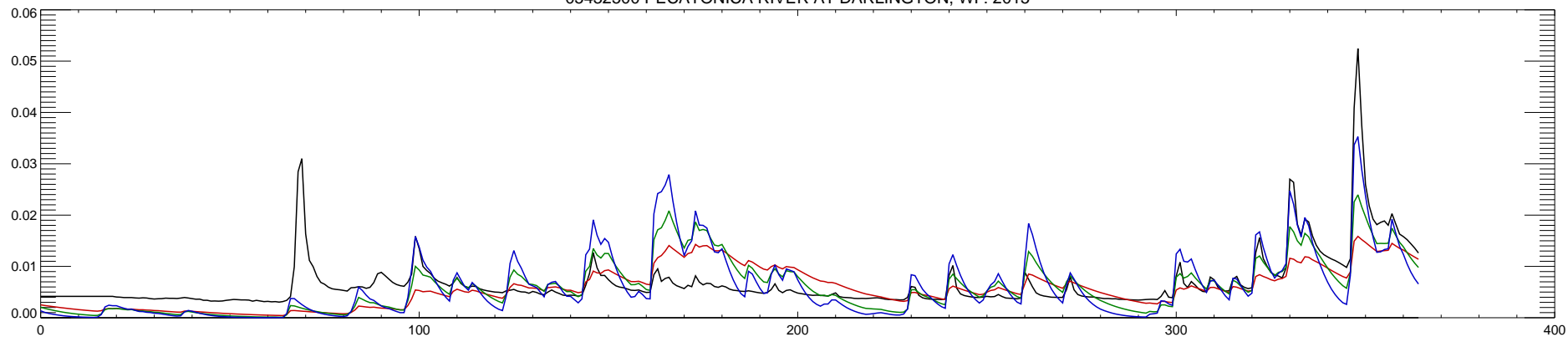
05432500 PECATONICA RIVER AT DARLINGTON, WI : 2016
