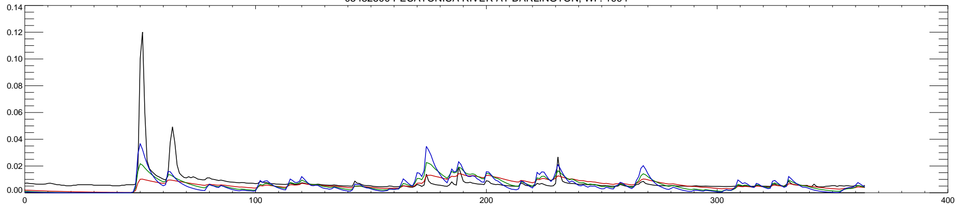
05432500 PECATONICA RIVER AT DARLINGTON, WI : 1995
