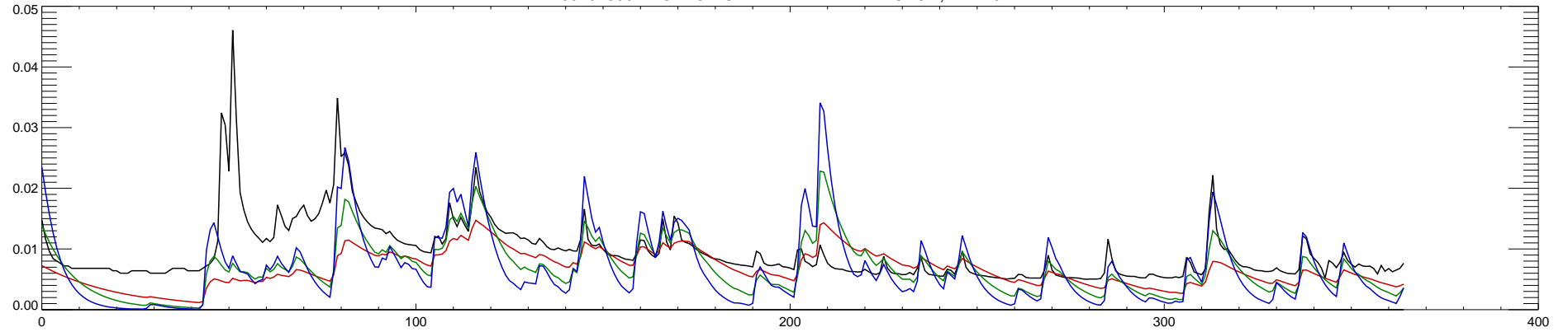
05432500 PECATONICA RIVER AT DARLINGTON, WI : 2012
