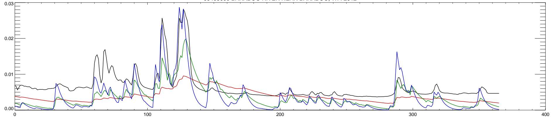
05405000 BARABOO RIVER NEAR BARABOO, WI : 2013
