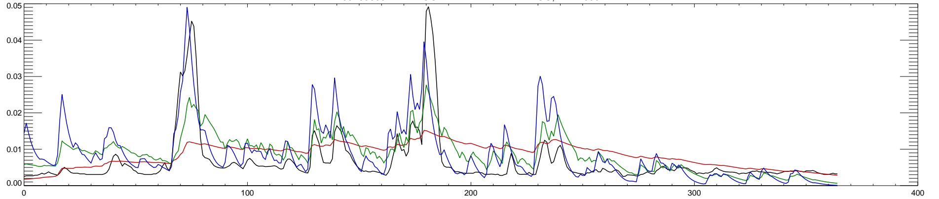
05405000 BARABOO RIVER NEAR BARABOO, WI : 1991
