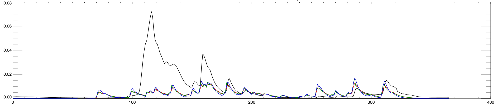
05131500 LITTLE FORK RIVER AT LITTLEFORK, MN : 2009
