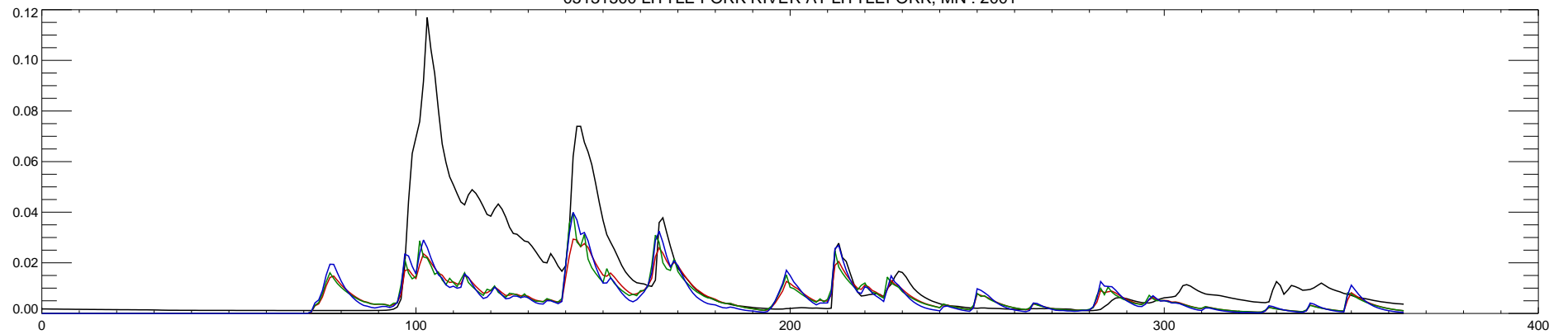
05131500 LITTLE FORK RIVER AT LITTLEFORK, MN : 2001
