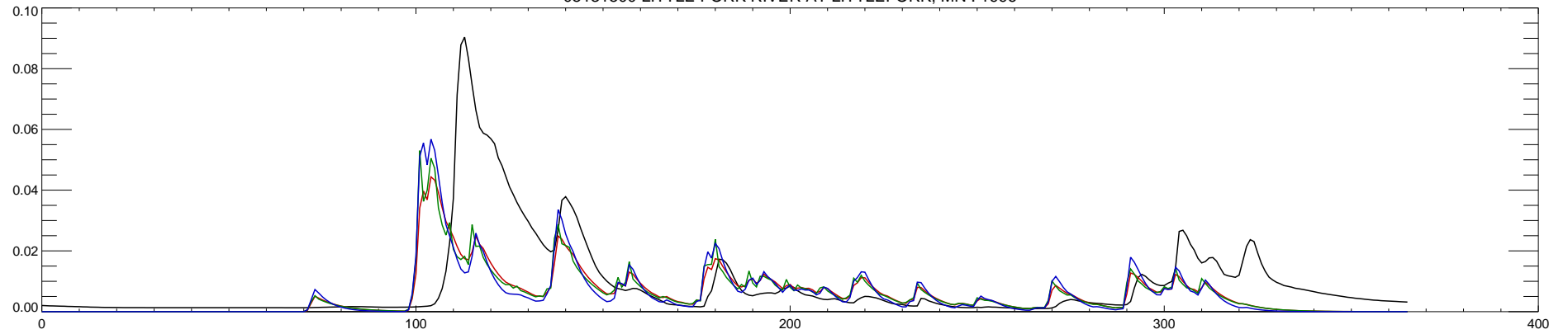
05131500 LITTLE FORK RIVER AT LITTLEFORK, MN : 1997
