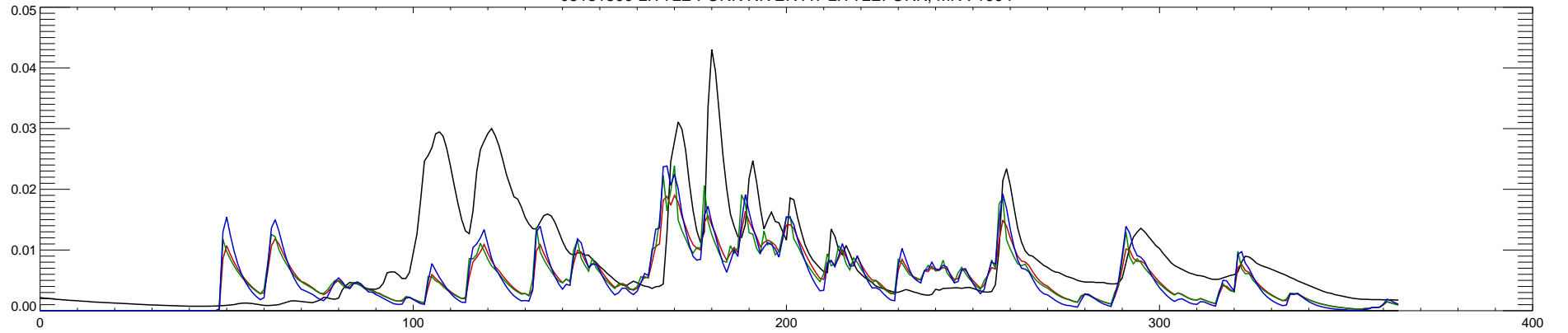
05131500 LITTLE FORK RIVER AT LITTLEFORK, MN : 1995
