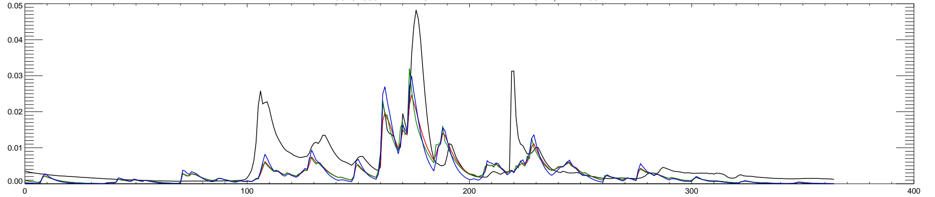
05131500 LITTLE FORK RIVER AT LITTLEFORK, MN : 2003
