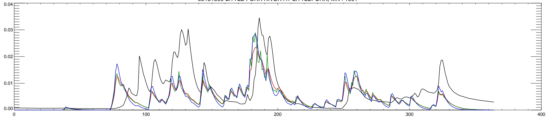
05131500 LITTLE FORK RIVER AT LITTLEFORK, MN : 1992
