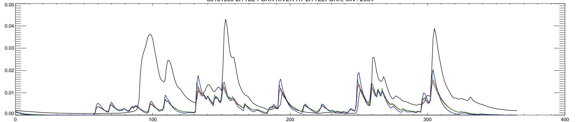
05131500 LITTLE FORK RIVER AT LITTLEFORK, MN : 2004
