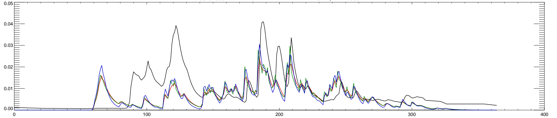
05131500 LITTLE FORK RIVER AT LITTLEFORK, MN : 1994
