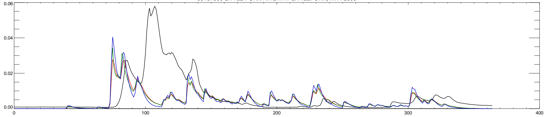
05131500 LITTLE FORK RIVER AT LITTLEFORK, MN : 2010
