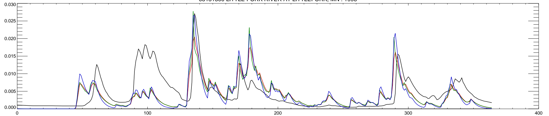
05131500 LITTLE FORK RIVER AT LITTLEFORK, MN : 1998
