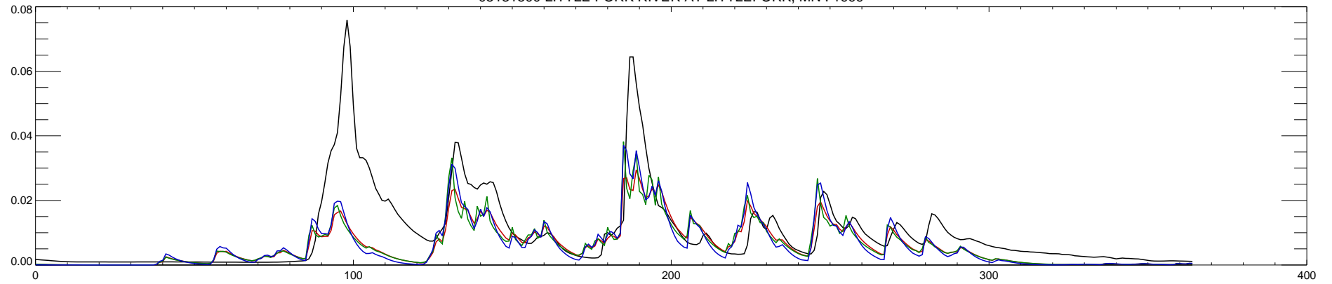
05131500 LITTLE FORK RIVER AT LITTLEFORK, MN : 2000
