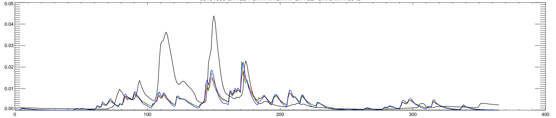
05131500 LITTLE FORK RIVER AT LITTLEFORK, MN : 2013
