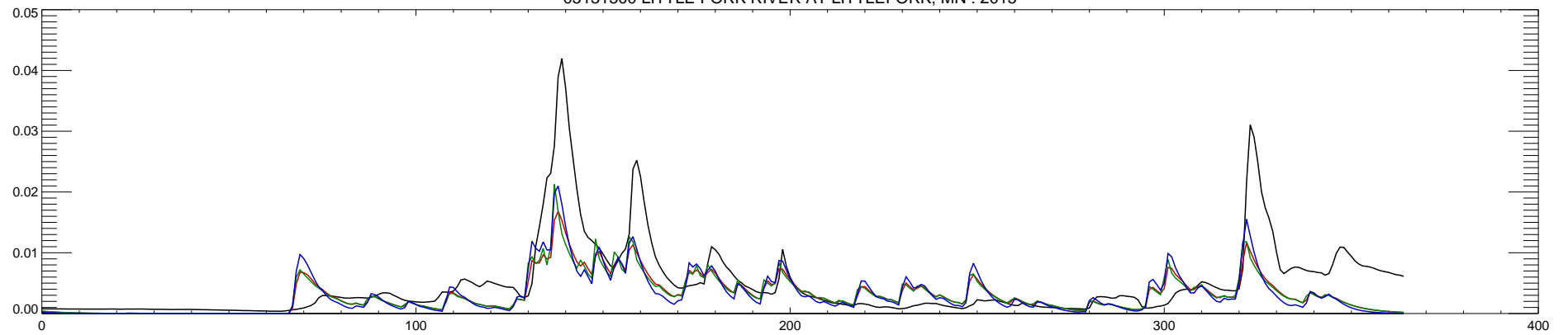
05131500 LITTLE FORK RIVER AT LITTLEFORK, MN : 2016
