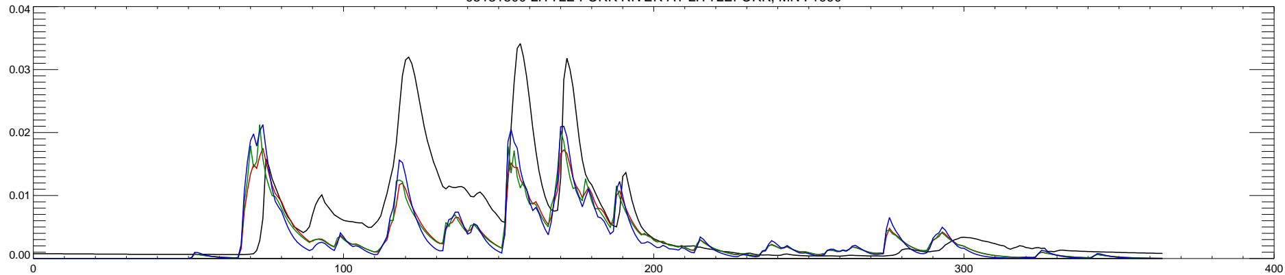
05131500 LITTLE FORK RIVER AT LITTLEFORK, MN : 1991
