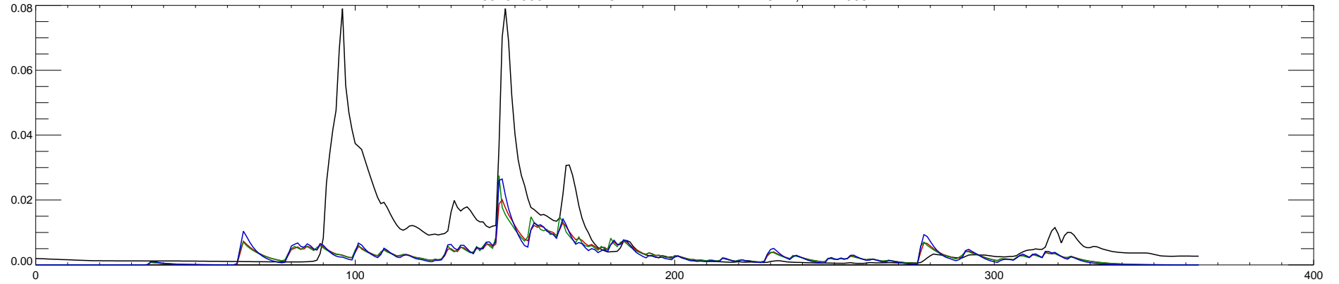
05131500 LITTLE FORK RIVER AT LITTLEFORK, MN : 2006
