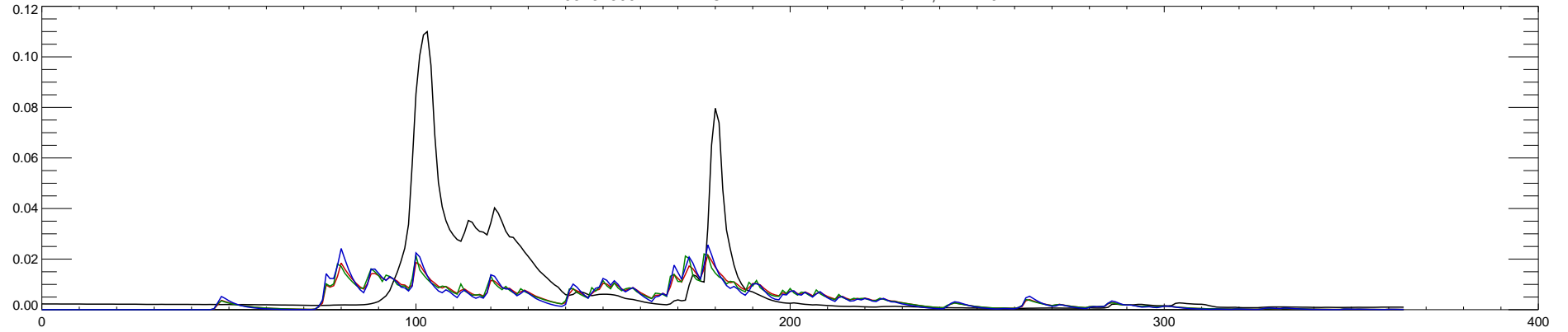
05131500 LITTLE FORK RIVER AT LITTLEFORK, MN : 2012
