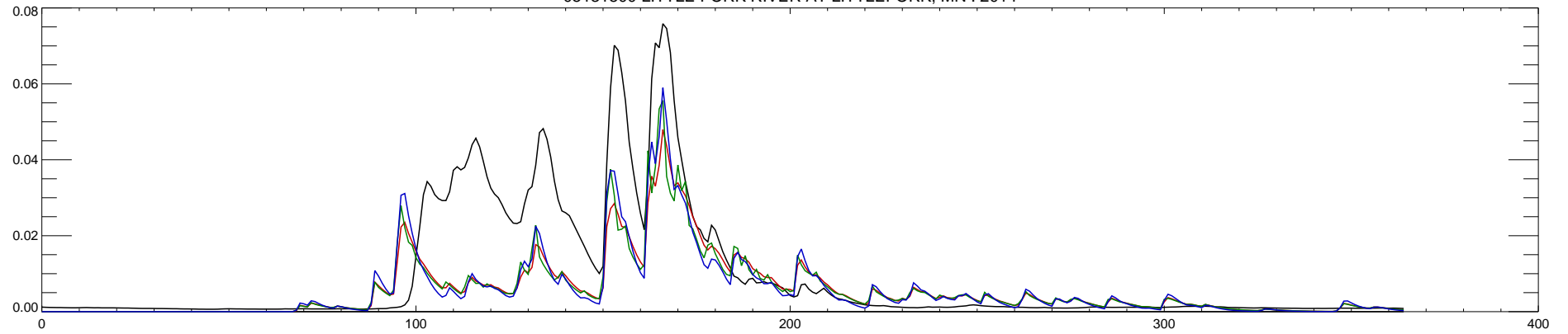
05131500 LITTLE FORK RIVER AT LITTLEFORK, MN : 2015
