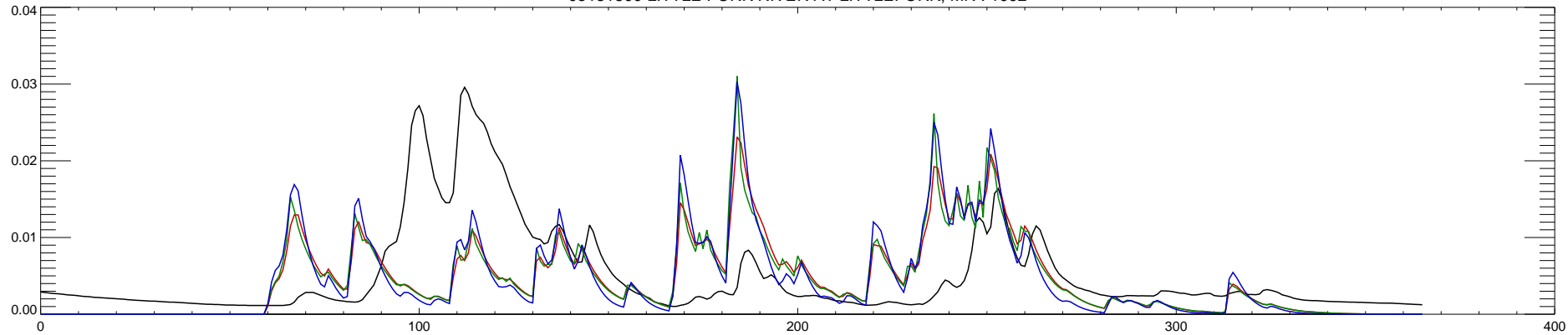
05131500 LITTLE FORK RIVER AT LITTLEFORK, MN : 1992
