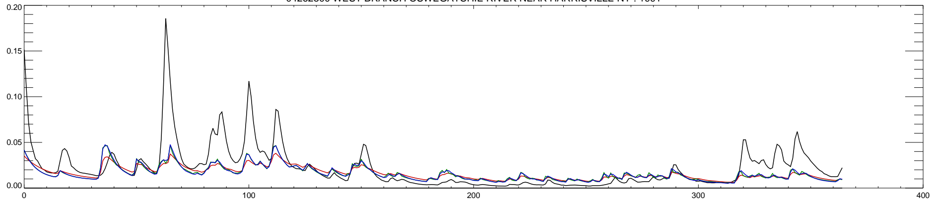
04262500 WEST BRANCH OSWEGATCHIE RIVER NEAR HARRISVILLE NY : 1992
