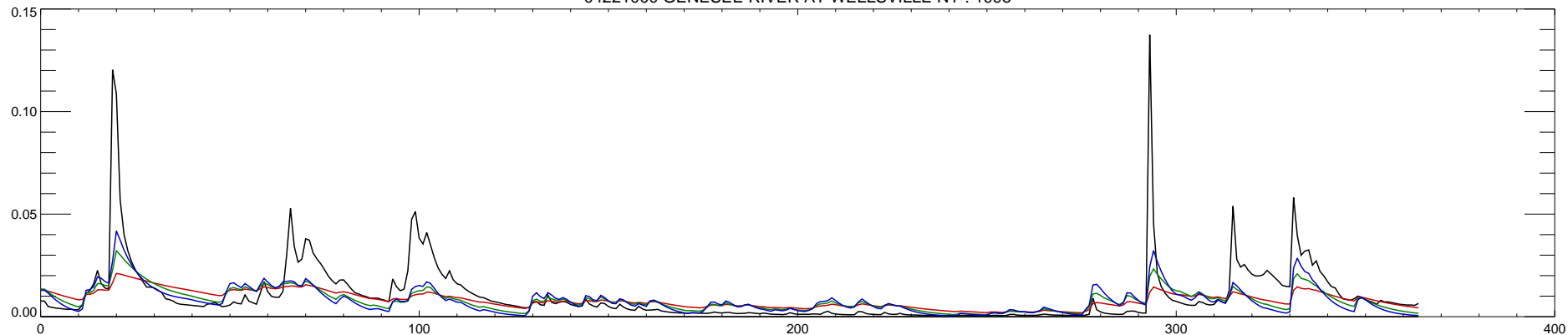
04221000 GENESEE RIVER AT WELLSVILLE NY : 1995
