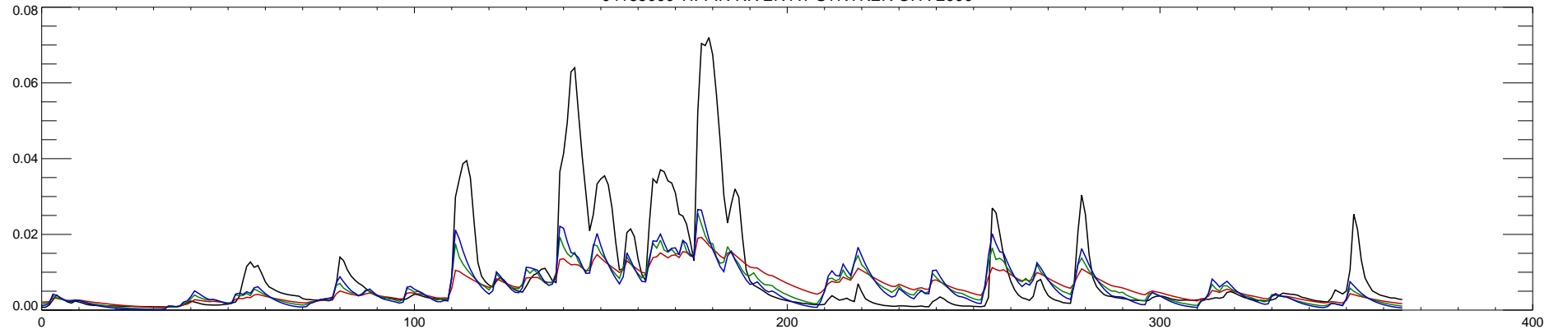
04185000 TIFFIN RIVER AT STRYKER OH : 2001
