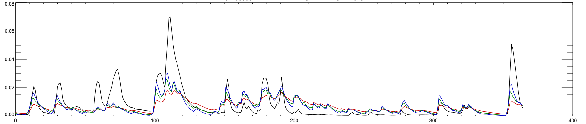
04185000 TIFFIN RIVER AT STRYKER OH : 2013
