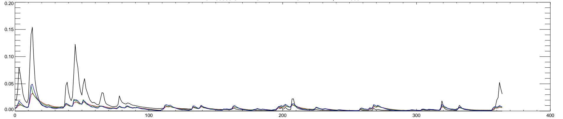
04180000 CEDAR CREEK NEAR CEDARVILLE, IN : 2006
