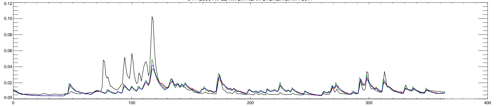
04142000 RIFLE RIVER NEAR STERLING, MI : 2012
