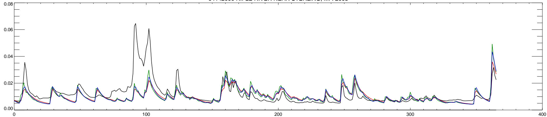
04142000 RIFLE RIVER NEAR STERLING, MI : 2009
