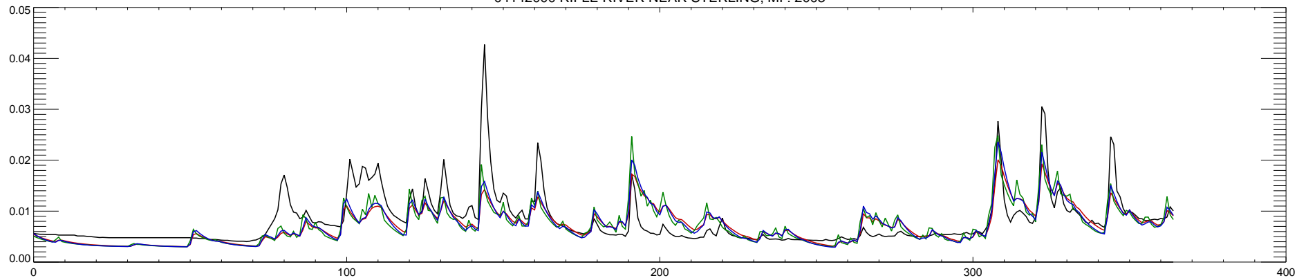
04142000 RIFLE RIVER NEAR STERLING, MI : 2004
