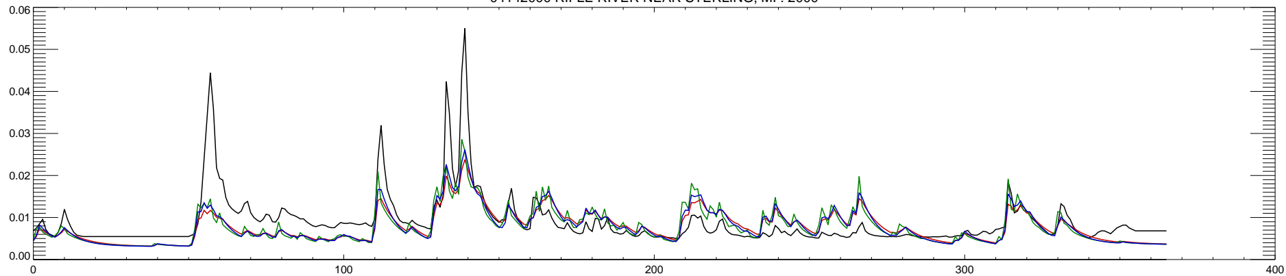
04142000 RIFLE RIVER NEAR STERLING, MI : 2001
