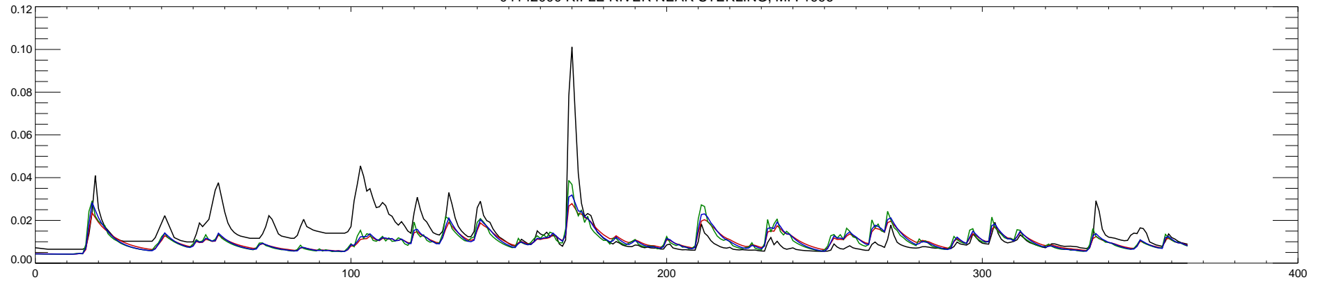
04142000 RIFLE RIVER NEAR STERLING, MI : 1997
