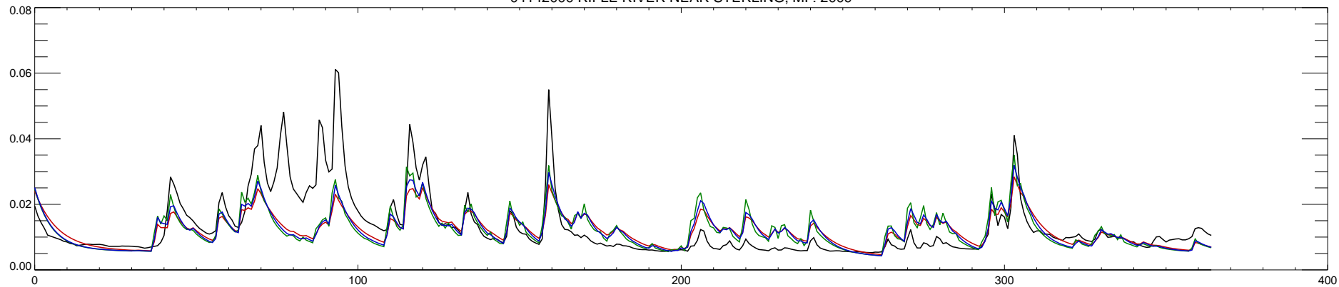
04142000 RIFLE RIVER NEAR STERLING, MI : 2010
