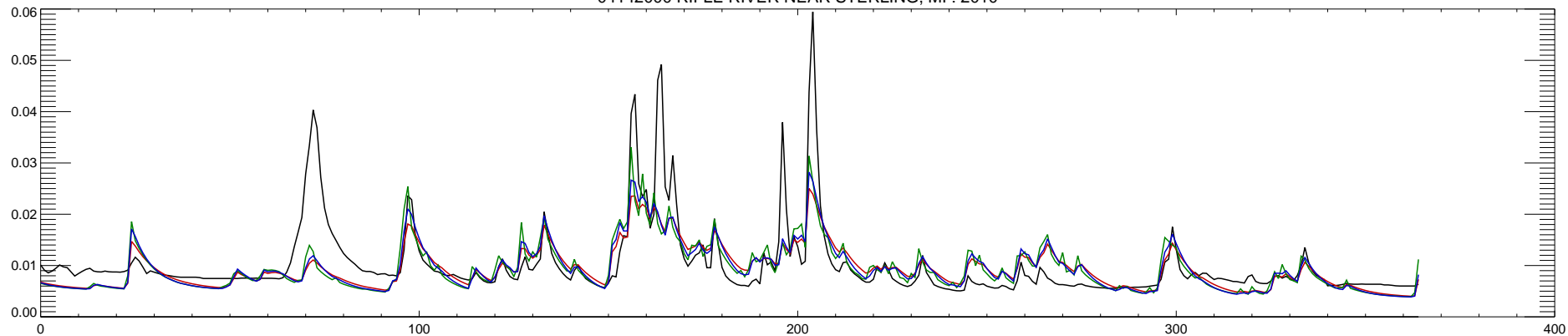
04142000 RIFLE RIVER NEAR STERLING, MI : 2010
