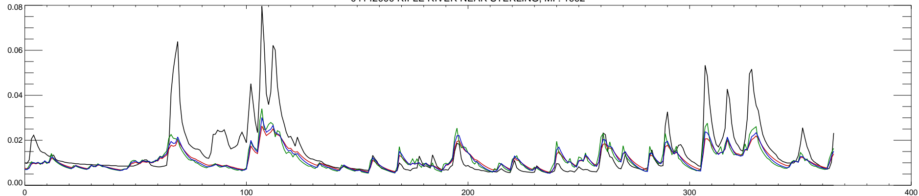
04142000 RIFLE RIVER NEAR STERLING, MI : 1992
