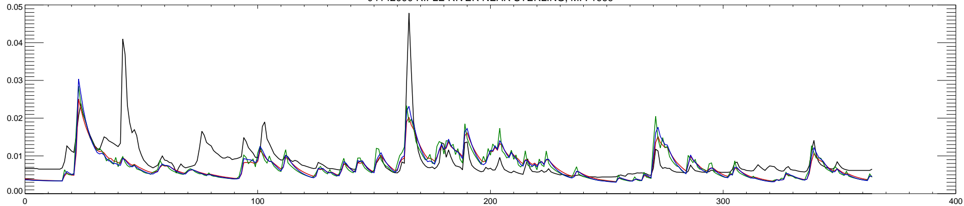
04142000 RIFLE RIVER NEAR STERLING, MI : 2000
