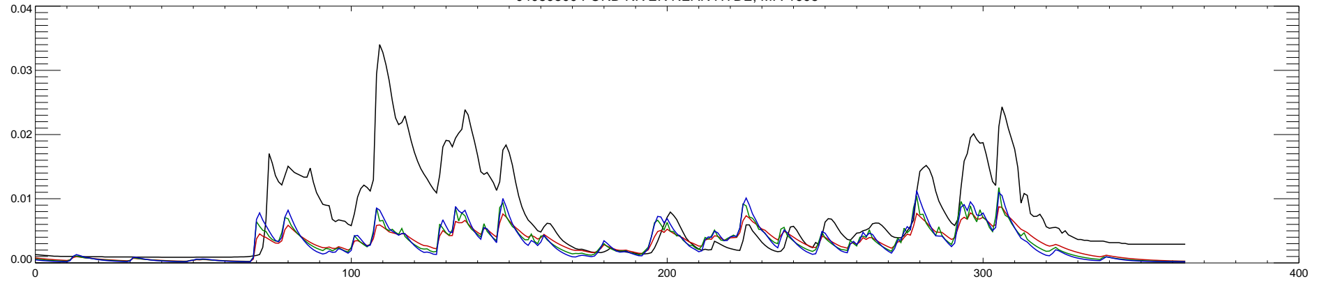
04059500 FORD RIVER NEAR HYDE, MI : 1995
