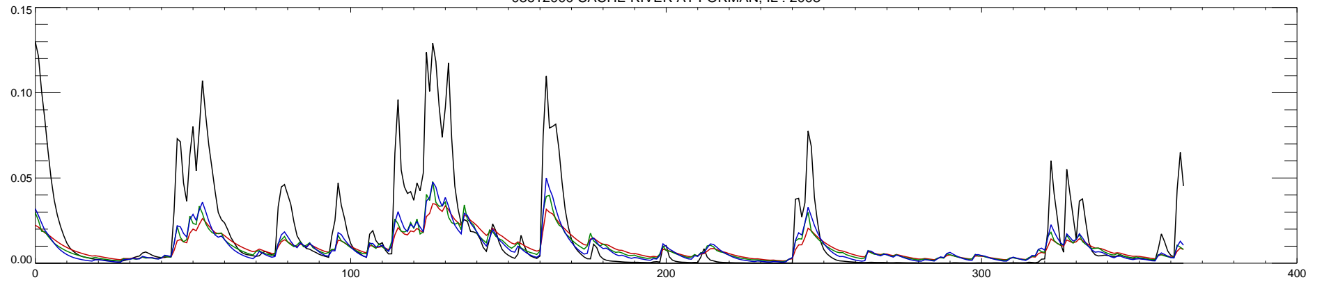
03612000 CACHE RIVER AT FORMAN, IL : 2004
