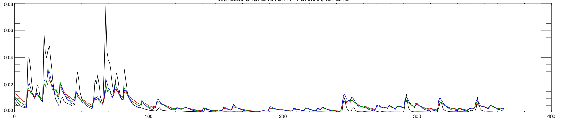
03612000 CACHE RIVER AT FORMAN, IL : 2013
