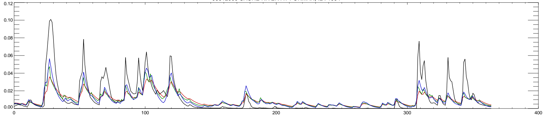
03612000 CACHE RIVER AT FORMAN, IL : 1995
