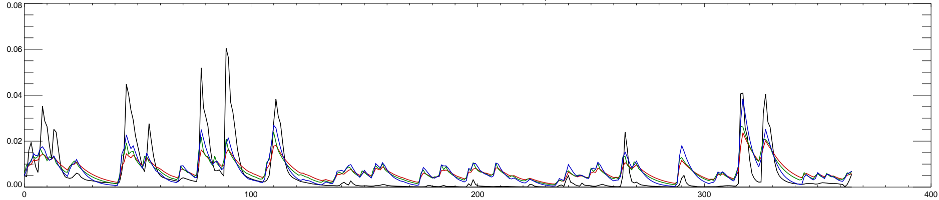
03612000 CACHE RIVER AT FORMAN, IL : 1992
