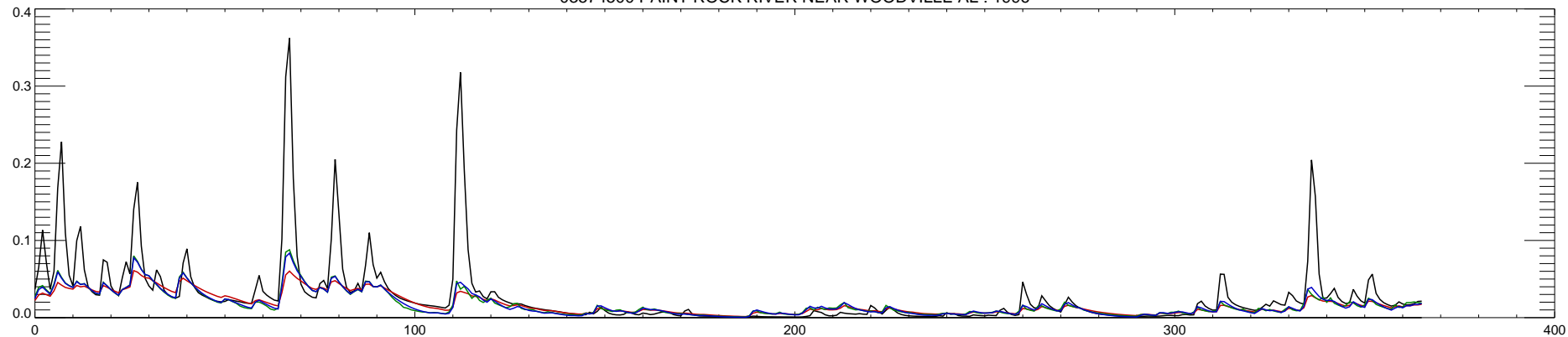
03574500 PAINT ROCK RIVER NEAR WOODVILLE AL : 1997
