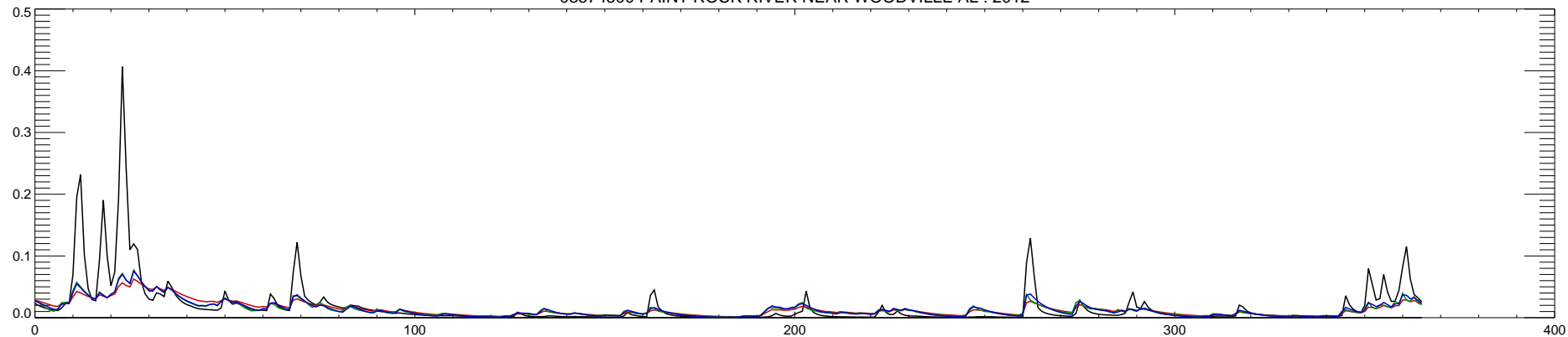
03574500 PAINT ROCK RIVER NEAR WOODVILLE AL : 2013
