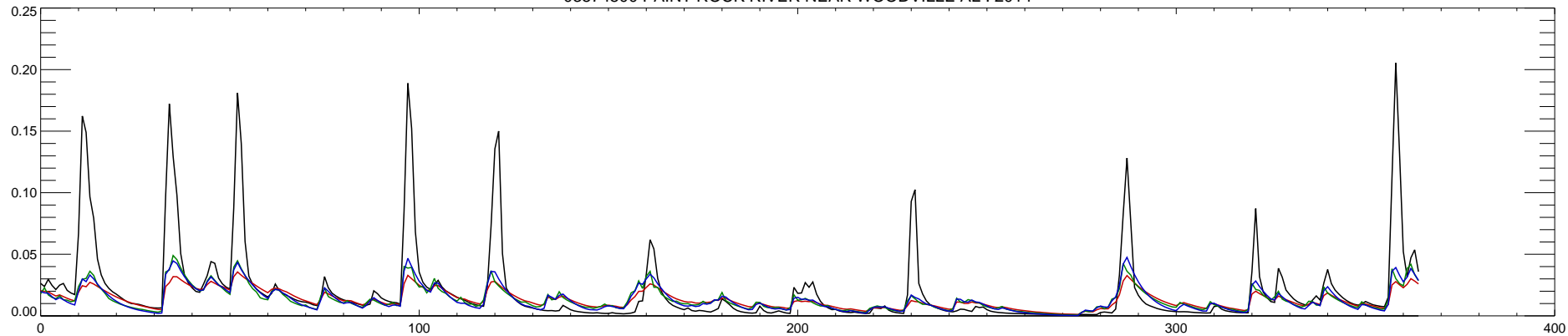
03574500 PAINT ROCK RIVER NEAR WOODVILLE AL : 2015
