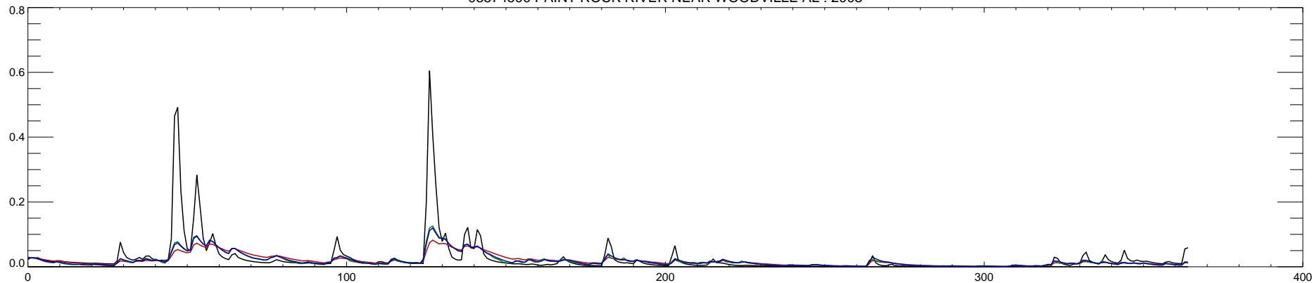
03574500 PAINT ROCK RIVER NEAR WOODVILLE AL : 2004
