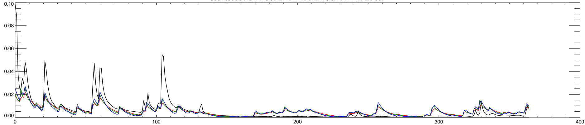
03574500 PAINT ROCK RIVER NEAR WOODVILLE AL : 2007
