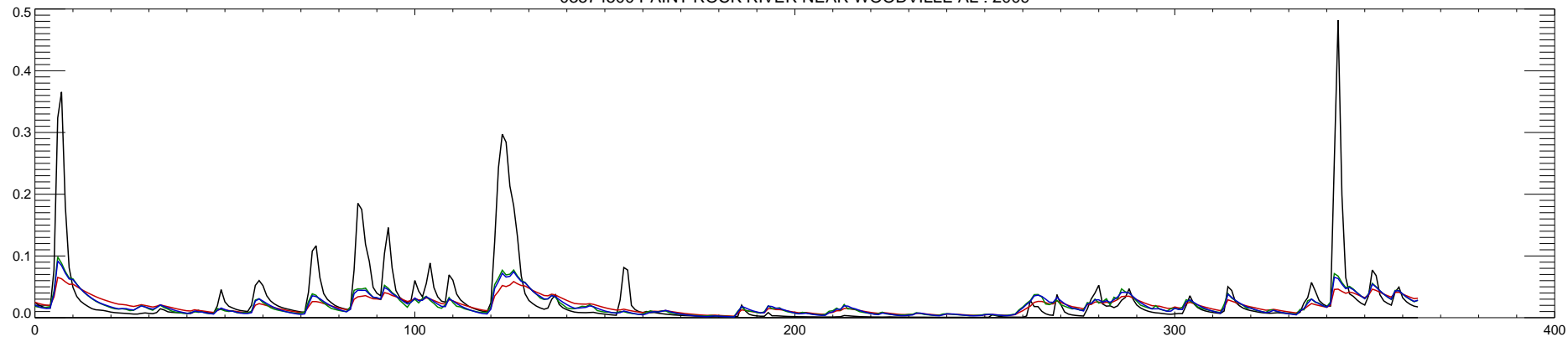
03574500 PAINT ROCK RIVER NEAR WOODVILLE AL : 2010
