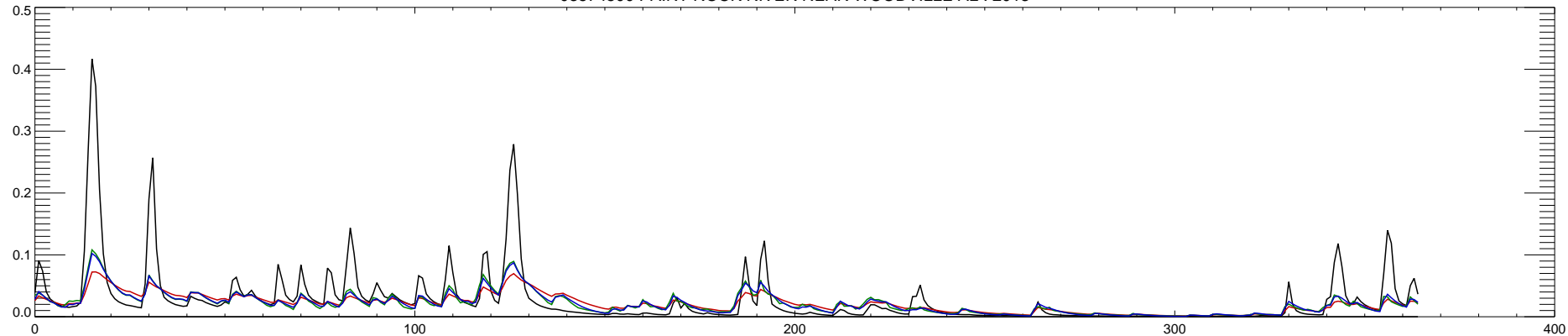
03574500 PAINT ROCK RIVER NEAR WOODVILLE AL : 2013
