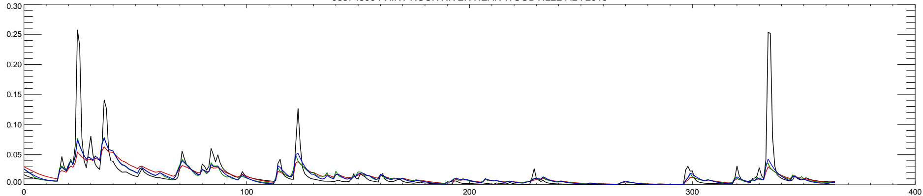
03574500 PAINT ROCK RIVER NEAR WOODVILLE AL : 2010
