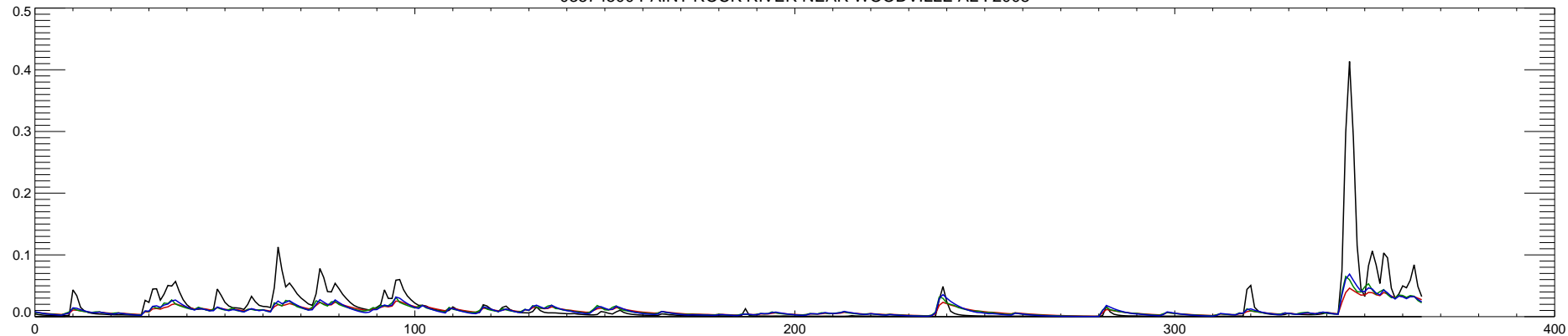
03574500 PAINT ROCK RIVER NEAR WOODVILLE AL : 2009
