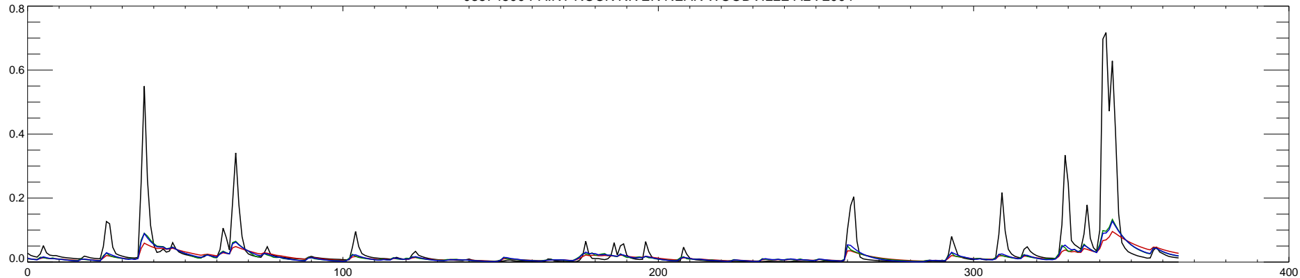
03574500 PAINT ROCK RIVER NEAR WOODVILLE AL : 2004
