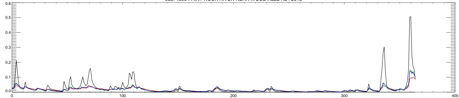
03574500 PAINT ROCK RIVER NEAR WOODVILLE AL : 2016
