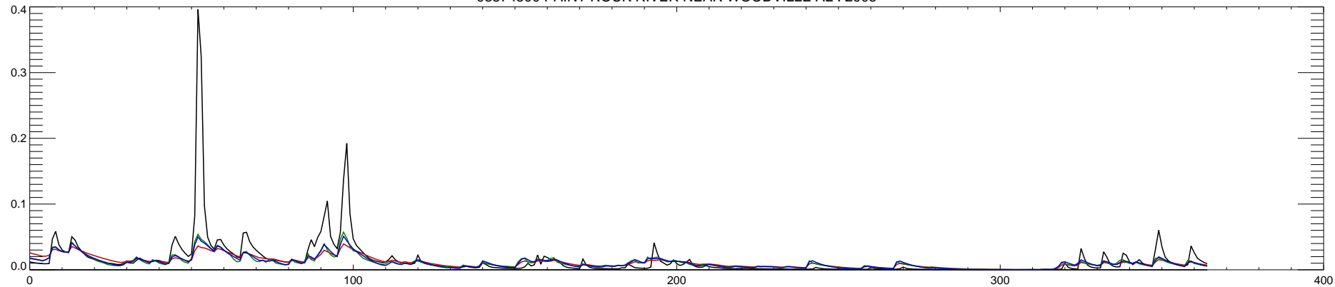
03574500 PAINT ROCK RIVER NEAR WOODVILLE AL : 2006
