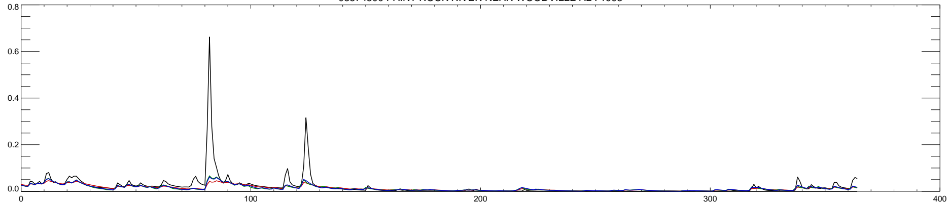
03574500 PAINT ROCK RIVER NEAR WOODVILLE AL : 1994
