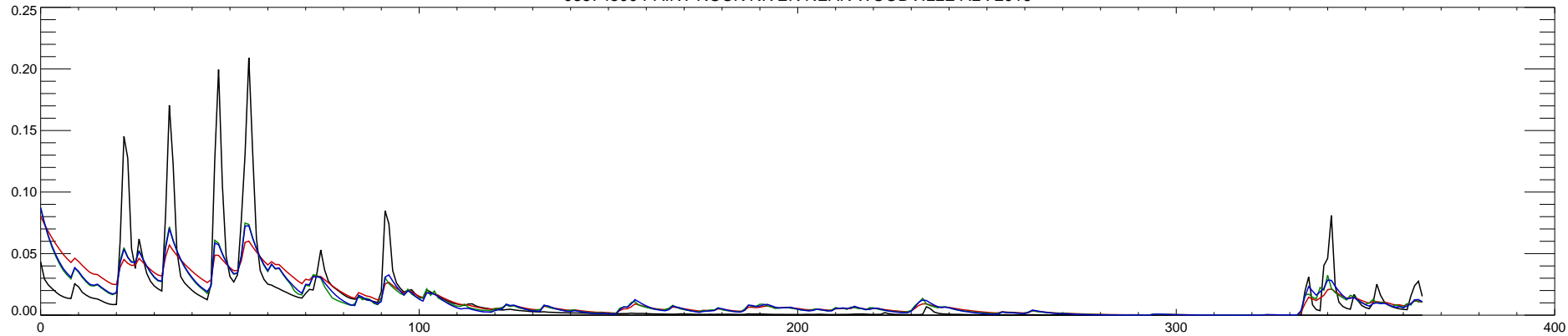
03574500 PAINT ROCK RIVER NEAR WOODVILLE AL : 2016
