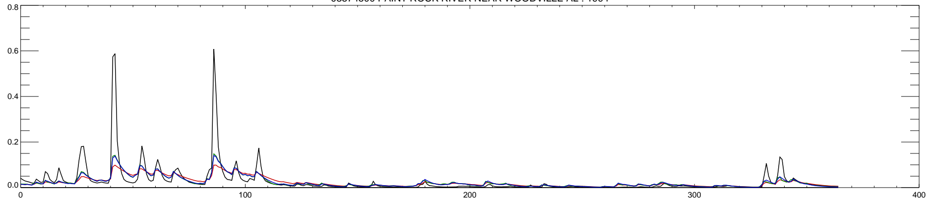
03574500 PAINT ROCK RIVER NEAR WOODVILLE AL : 1995
