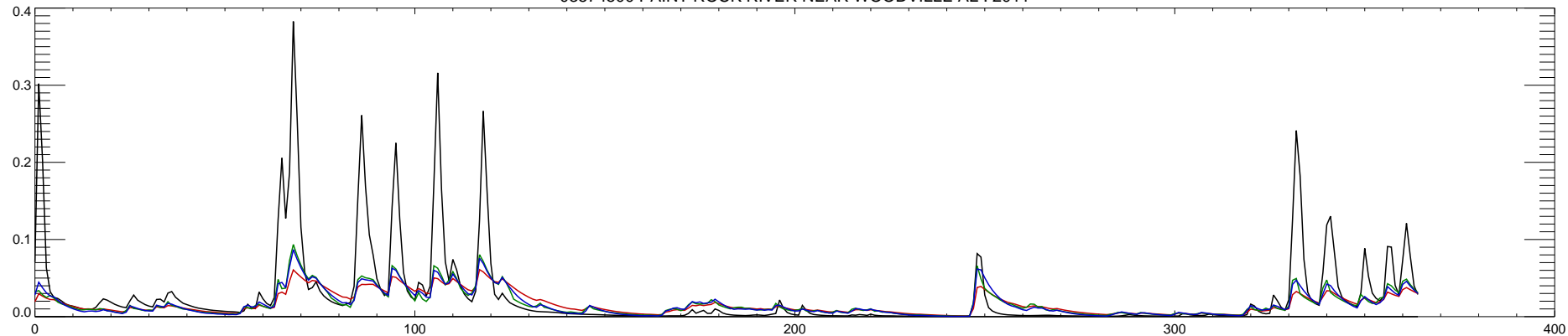
03574500 PAINT ROCK RIVER NEAR WOODVILLE AL : 2012
