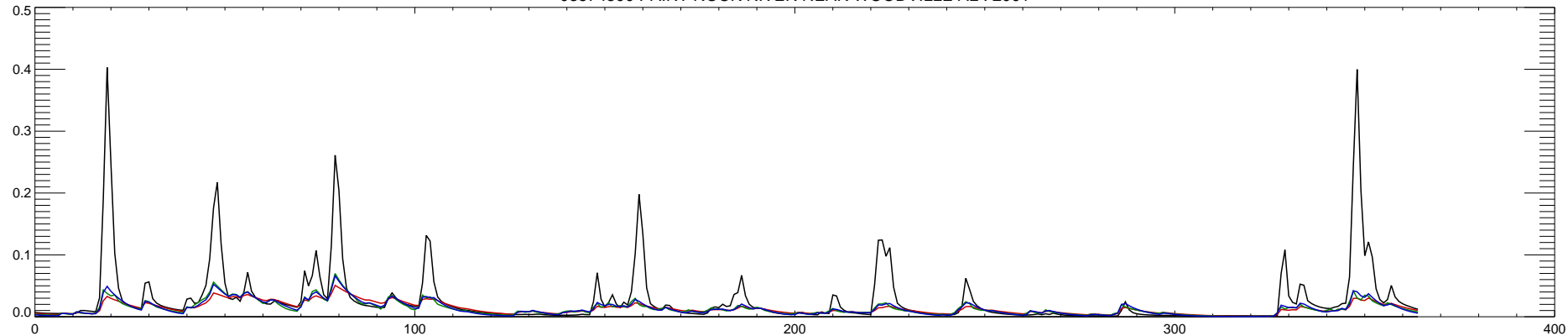
03574500 PAINT ROCK RIVER NEAR WOODVILLE AL : 2001
