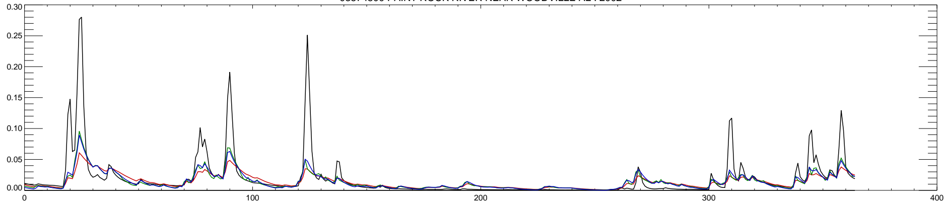
03574500 PAINT ROCK RIVER NEAR WOODVILLE AL : 2003
