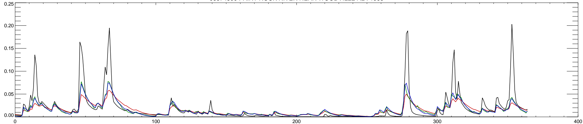
03574500 PAINT ROCK RIVER NEAR WOODVILLE AL : 1995
