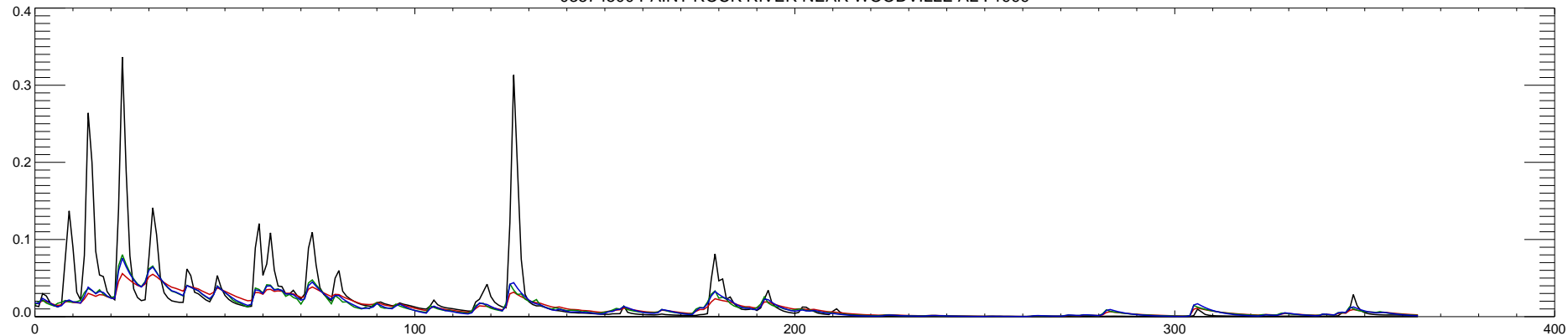
03574500 PAINT ROCK RIVER NEAR WOODVILLE AL : 2000
