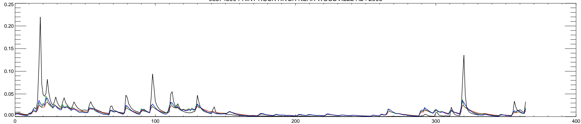
03574500 PAINT ROCK RIVER NEAR WOODVILLE AL : 2007
