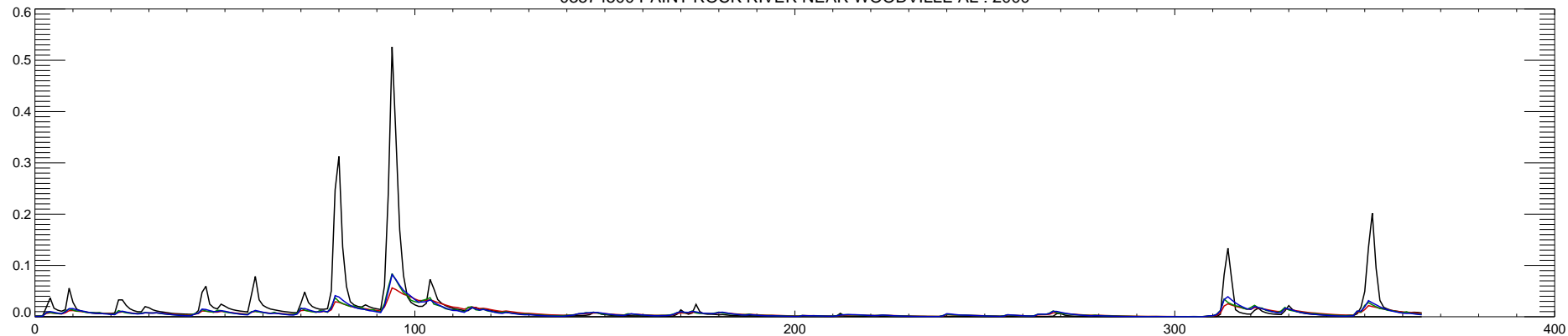
03574500 PAINT ROCK RIVER NEAR WOODVILLE AL : 2001
