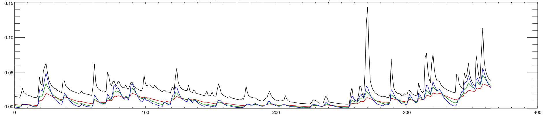
03443000 FRENCH BROAD RIVER AT BLANTYRE, NC : 2003
