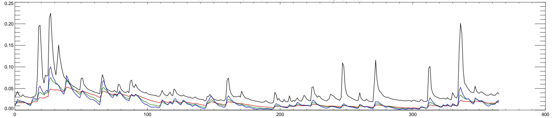
03443000 FRENCH BROAD RIVER AT BLANTYRE, NC : 1997
