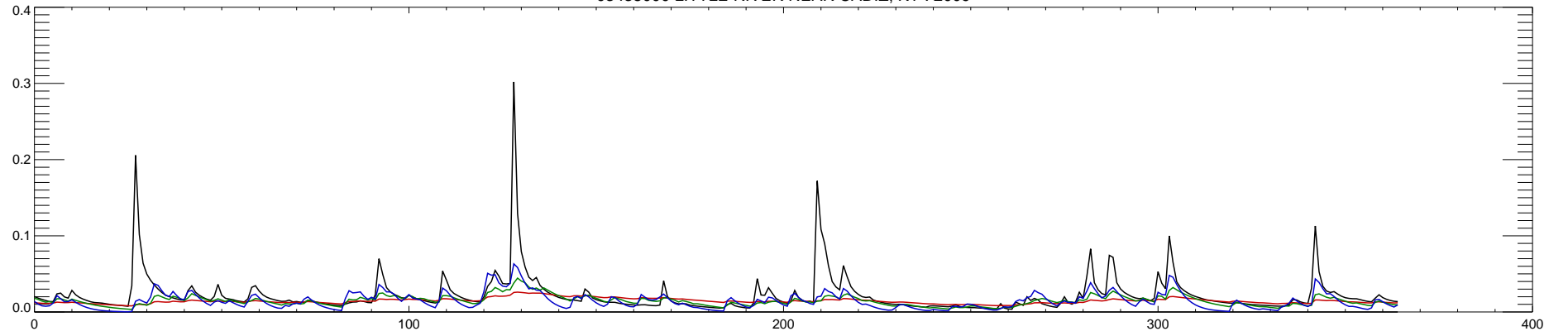
03438000 LITTLE RIVER NEAR CADIZ, KY : 2010
